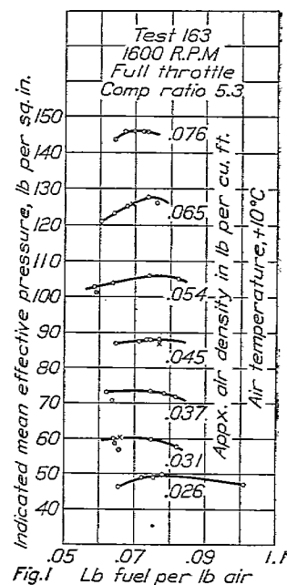
Fig. 1 Test on 8-cylinder engine, bore 4.72 inches, stroke 5.12 inches.
