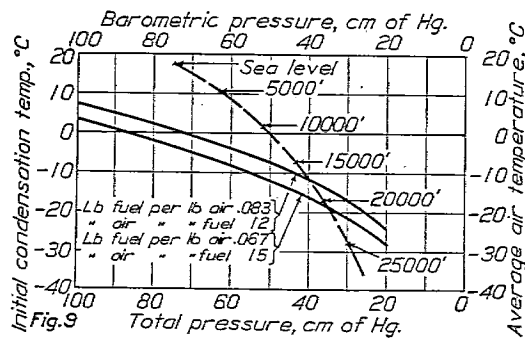
Fuel characteristics of domestic aviation gasoline (from Wilson and Barnard).
