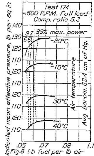
Test on 8-cylinder engine, bore 4.72 inches stroke 5.12 inches.
