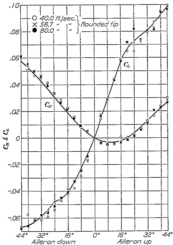
FIG. 9.—Clark Y wing. Aileron span 20 inches. Aileron chord 2.5 inches. Curva line represents rectangular tips—points not shown
