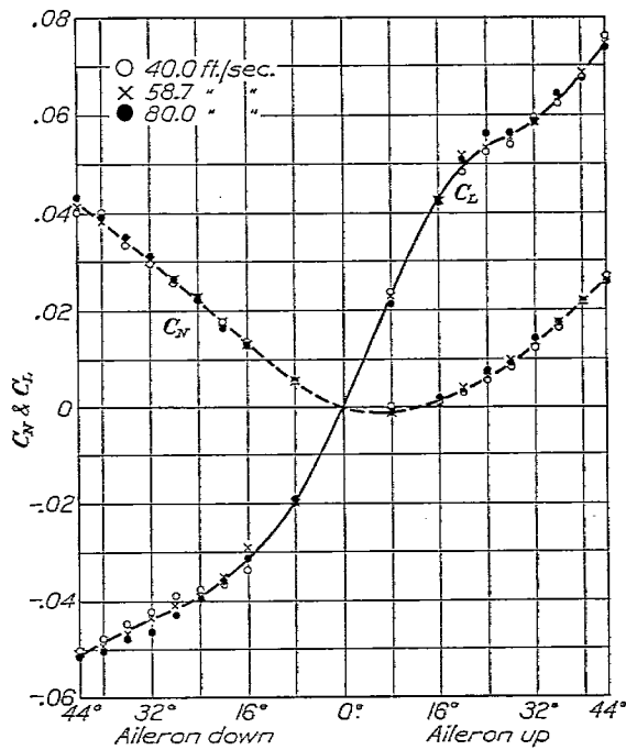
FIG. 8.—U. S. A. 27 wing. Aileron span 15 inches. Aileron chord 2.5 inches
