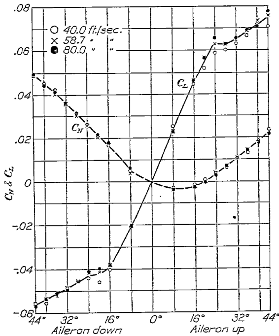
FIG. 7.—Clark Y wing. Aileron span 15 inches. Aileron chord 2.5 inches
