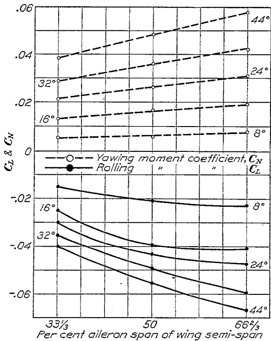
FIG. 13.—Clark Y wing. Aileron span varying. Aileron chord 2.5 inches. Aileron down
