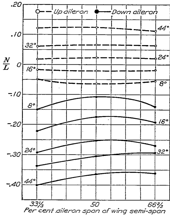
FIG. 15.—Clark Y wing. Aileron span varying. Aileron chord 2.5 inches. N/L=0.417 C_N/C_L
