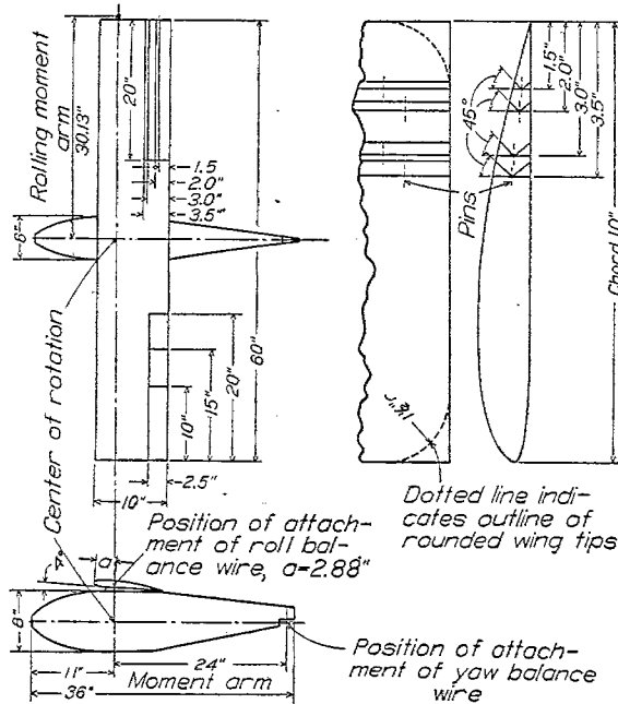
FIG. 3.—Varying aileron chord end of wing, Clark Y section, showing method of hinging ailerons. U. S. A. 27 similarly constructed
