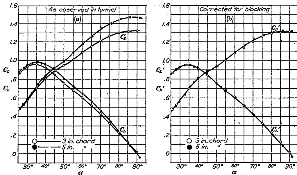
FIGURE 59.—Clark Y wings. A. R. 8
