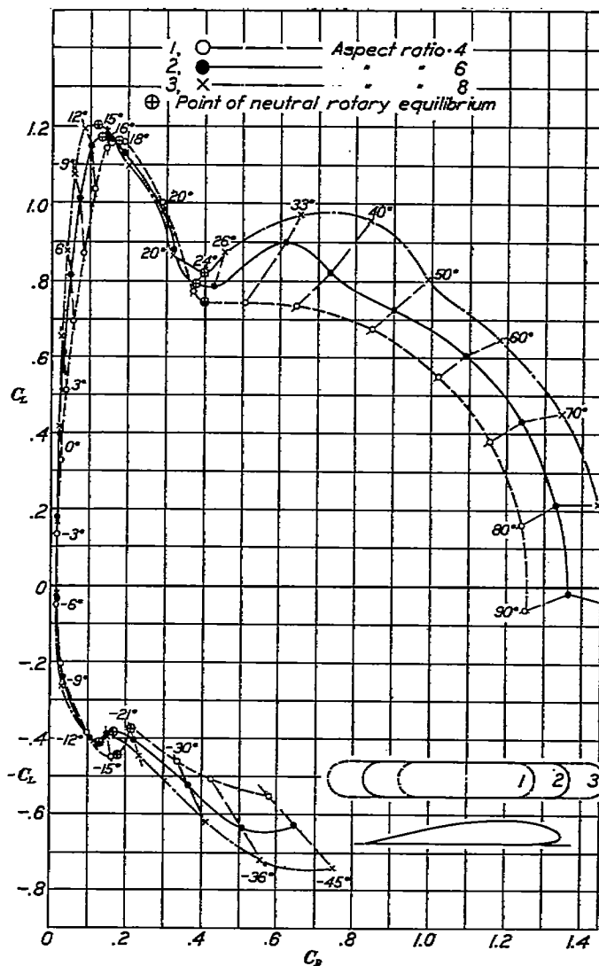
FIGURE 8.—Monoplane wings. Aspect ratio effect. Clark Y. Circular tips. 5-inch chord. FIGURE 9.—Monoplane wings. Aspect ratio effect. Polars. Clark Y. Circular tips. 5-inch chord.
