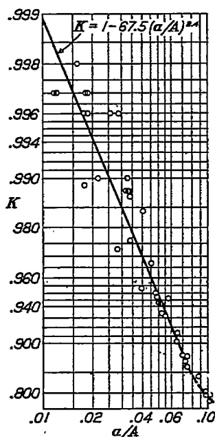
FIGURE 55.—Blocking correction versus area ratio (logarithmic)
