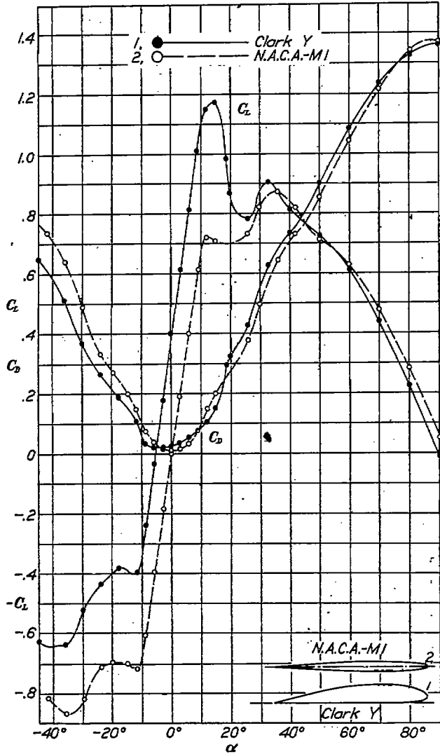
FIGURE 20.—Monoplane wings. Profile effect. Clark Y. and N. A. C. A.-M1. Circular tips. 5-inch chord. A. R. 6
