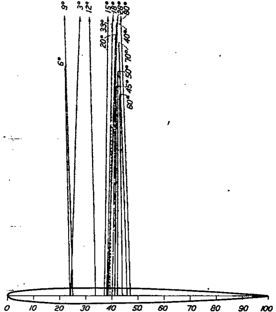
FIGURE 23.—Monoplane vector diagram. N. A. C. A.-M1. Circular tips. 5-inch chord. A. R. 6
