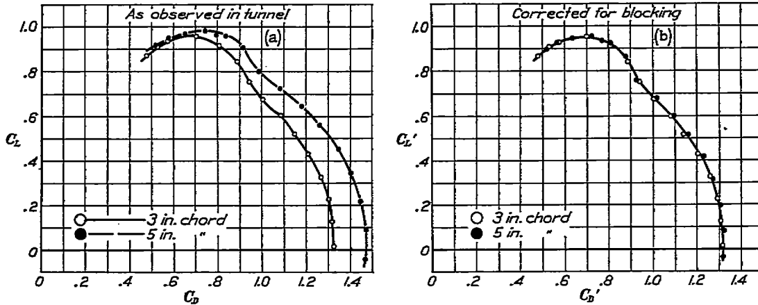
FIGURE 60.—Clark Y wings. A. R. 8. Polars
