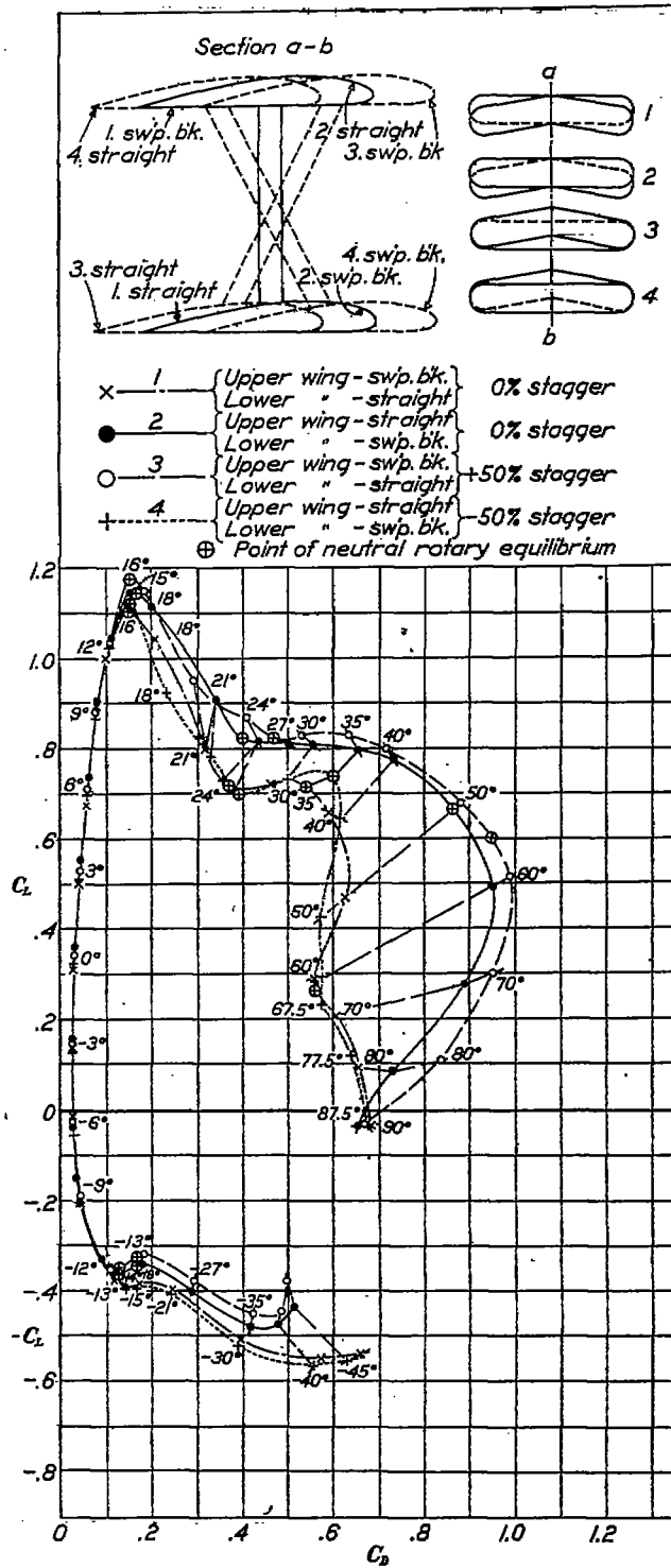
FIGURE 42.—Biplane wings. Sweep-back effect. Polars. Clark Y. Circular tips. 5-inch chord. A. R. 6. Gap/chord=1. Decalage, 0°
