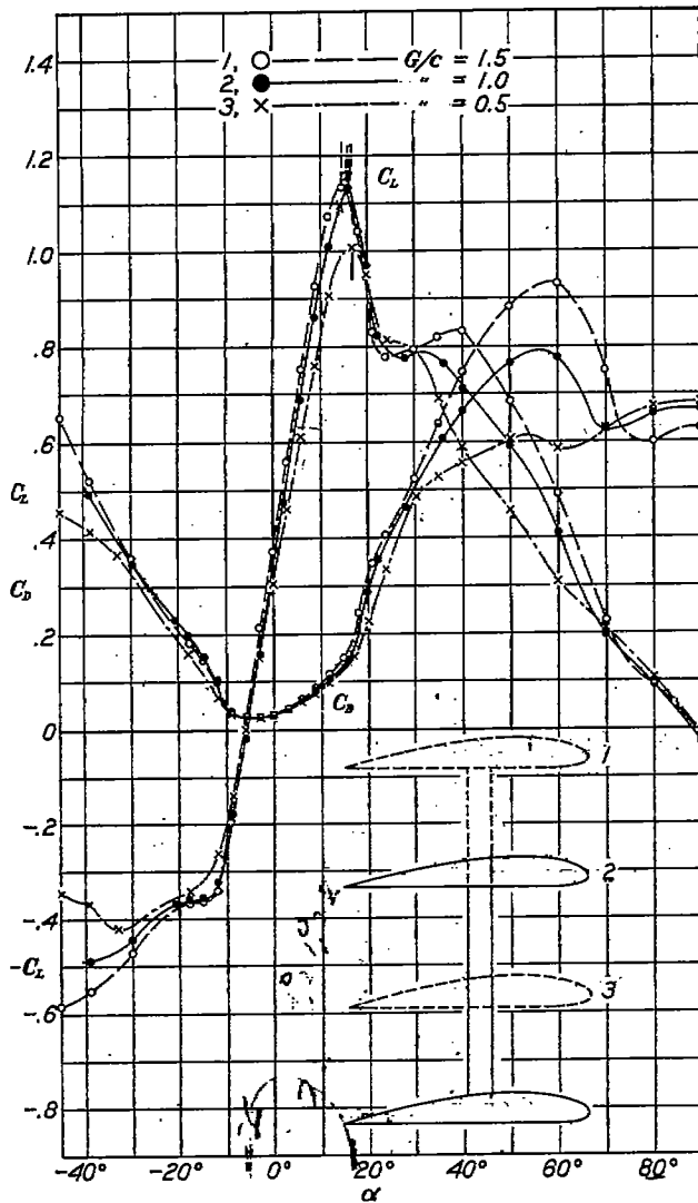
FIGURE 31.—Biplane wings. Gap effect. Clark Y. Circular tips. 5-inch chord. A. R. 6. Decalage, 0°. Stagger, 0
