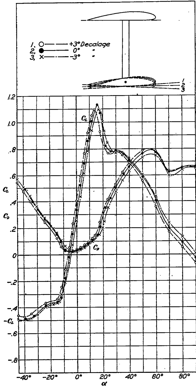
FIGURE 36.—Biplane wings. Decalage effect. Clark Y. Circular tips. 5-inch chord. A. R. 6. Gap/chord=1. Stagger, 0
