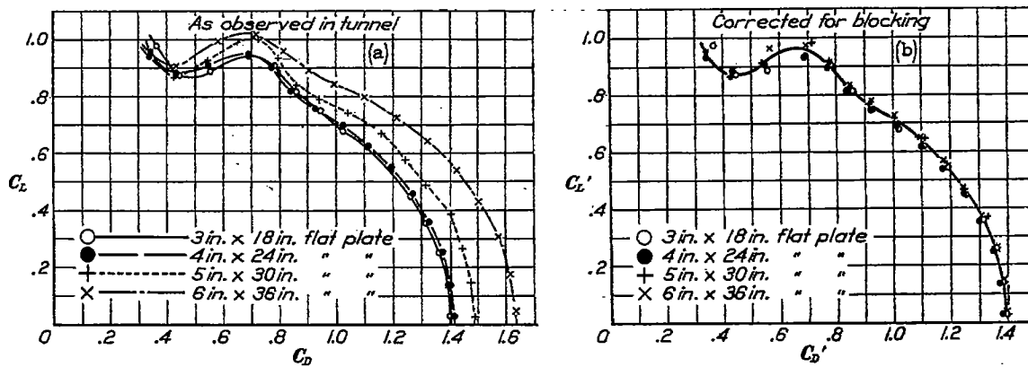
FIGURE 58.—Flat plates. A. R. 6. Polars
