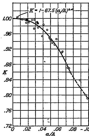
FIGURE 56.—Blocking correction versus area ratio
