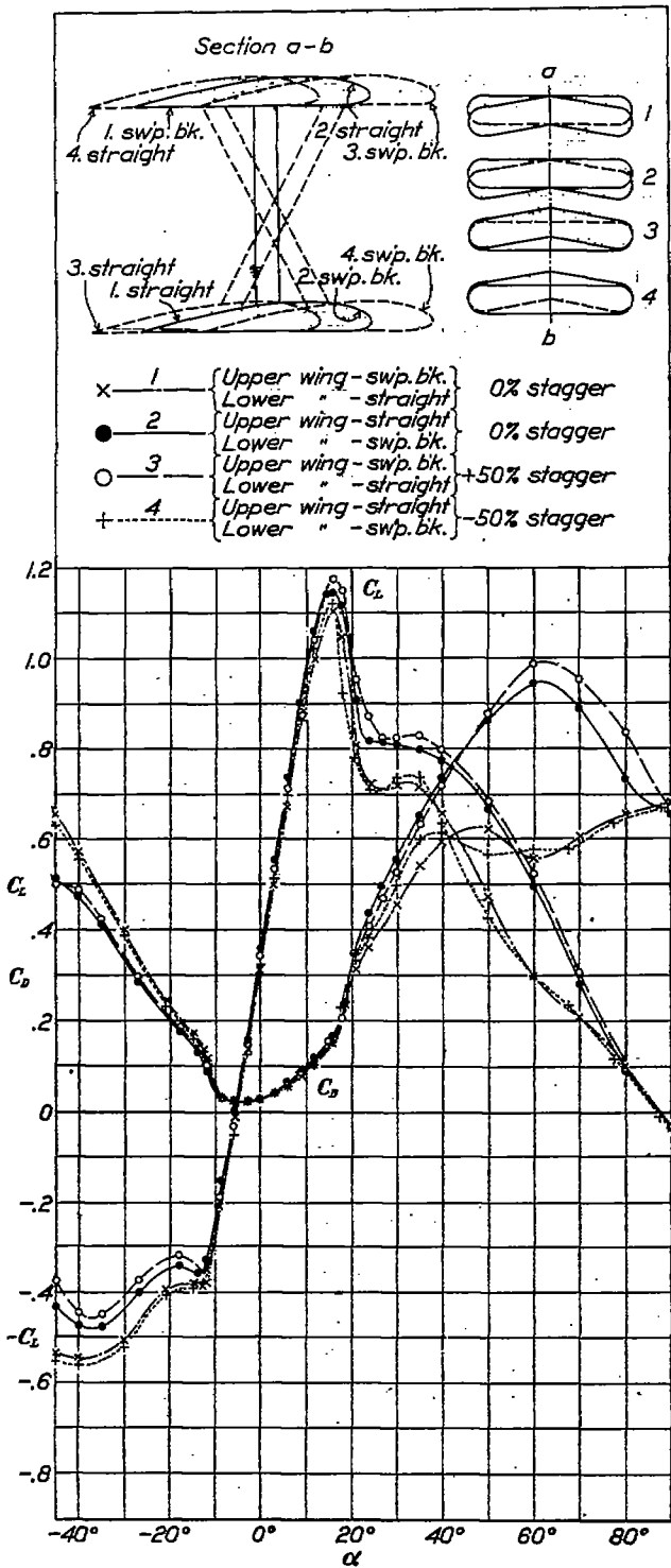
FIGURE 41.—Biplane wings. Sweep-back effect. Clark Y. Circular tips. 5-inch chord. A. R. 6. Gap/chord=1. Decalage, 0°
