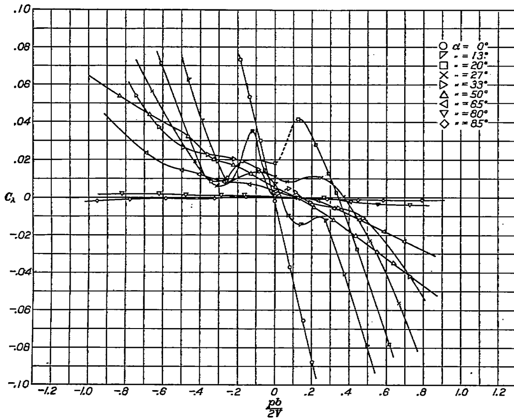
FIGURE 20.—Rolling moment coefficient vs. \frac{pb}{2V} for Clark Y monoplane wing model. Yaw=5°
