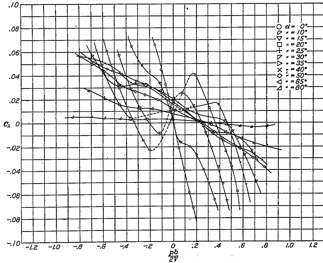
FIGURE 25.—Rolling moment coefficient vs. \frac{pb}{2V} for N. A. O. A. 86-M monoplane wing model. Yaw= 10^\circ
