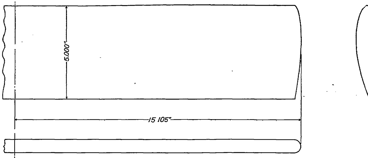
FIGURE 3.—Monoplane wing model—N. A. C. A. 84
