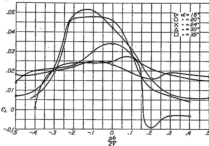
FIGURE 12.—Rolling moment due to yaw vs. \frac{pb}{2V} for N. A. C. A. 84 monoplane wing model. Yaw=10°
