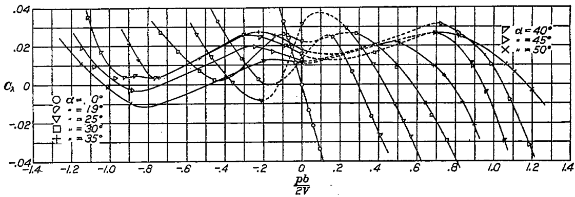
FIGURE 17.—Rolling moment coefficient vs. \frac{pb}{2V} for Clark Y biplane wing model. Yaw=10°
