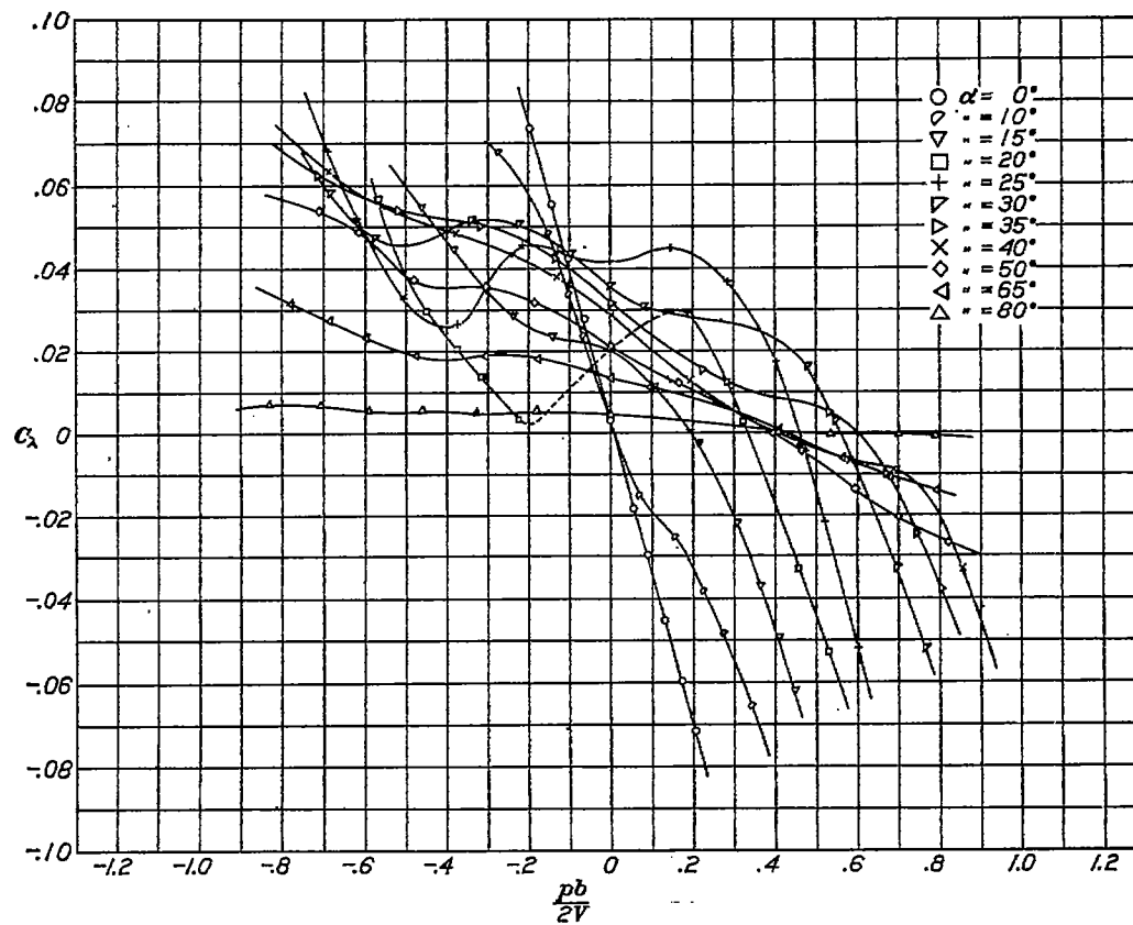
FIGURE 26.—Rolling moment coefficient vs. \frac{pb}{2V} for N. A. O. A. 86-M monoplane wing model. Yaw= 20^\circ
