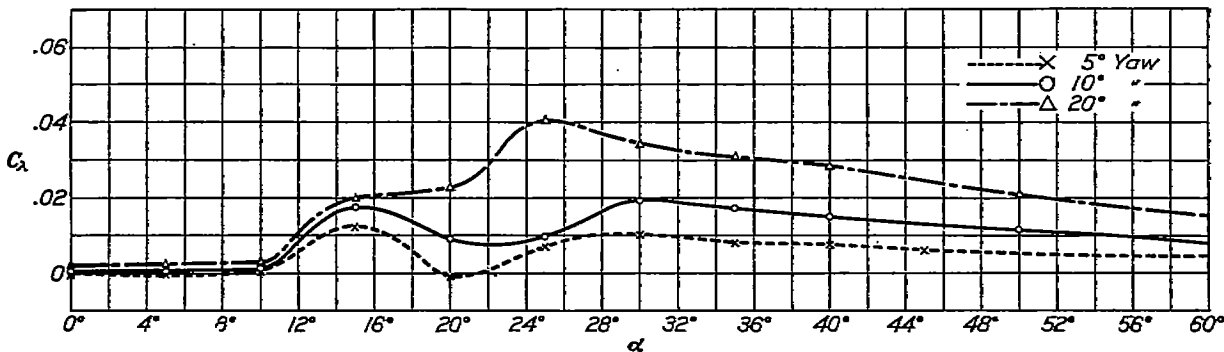
FIGURE 29.—Rolling moment due to yaw vs. angle of attack for N. A. C. A. 36-M monoplane. Yaw=5°, 10°, 20°. \frac{pb}{2V} = 0
