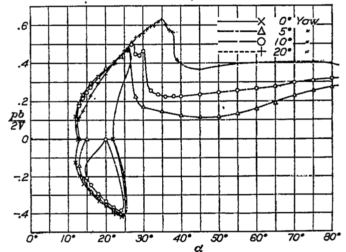
FIGURE 33.— \frac{pb}{2V} vs. angle of attack for N. A. O. A. 86-M monoplane wing model. Yaw=0°, 5°, 10°, 20°
