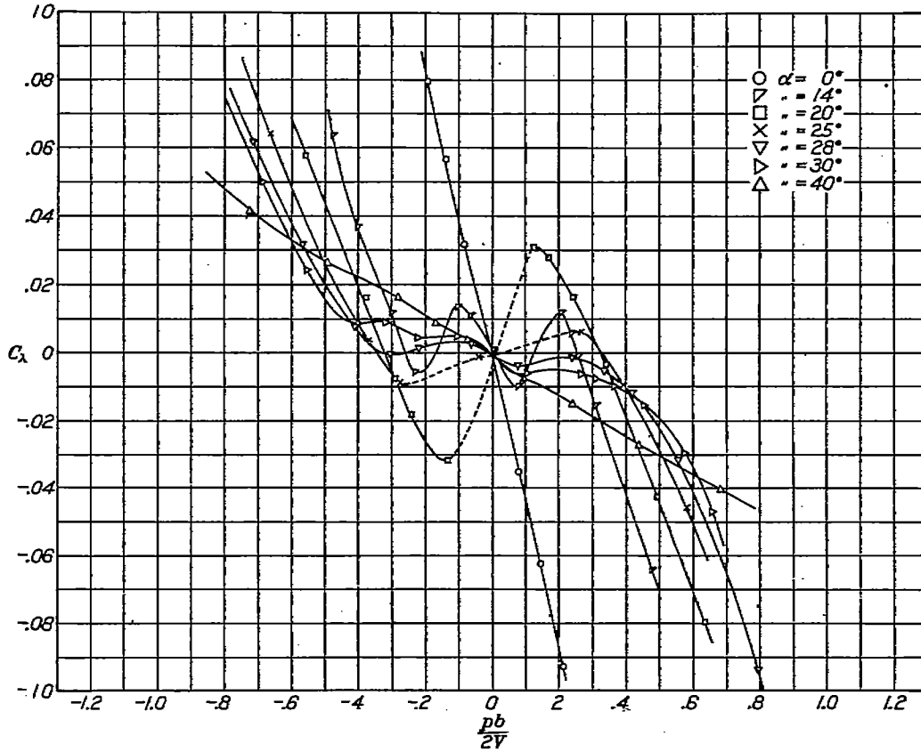
FIGURE 19.—Rolling moment coefficient vs. \frac{pb}{2V} for Clark Y monoplane wing model. Yaw=0°
