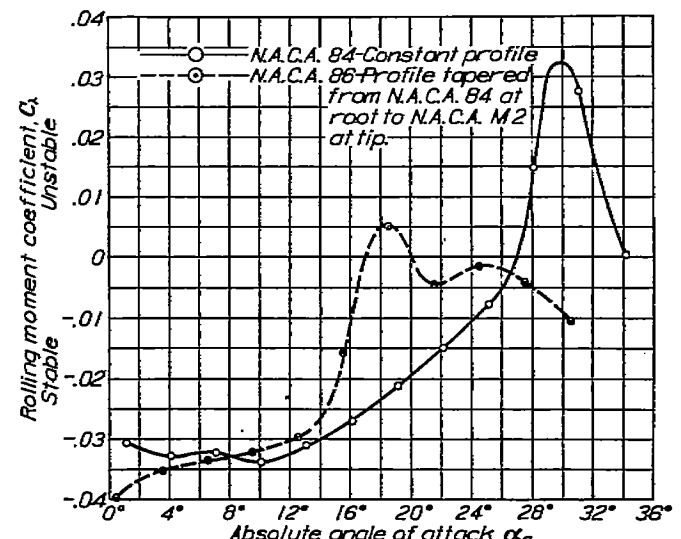
FIGURE 5.—Effect of variation in profile along the span on rolling moment due to roll at \frac{pb}{2V} = 0.05
