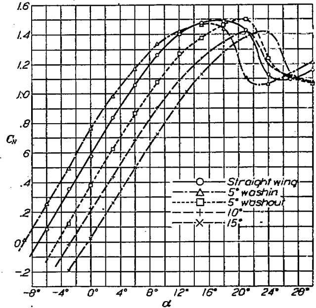
FIGURE 17.—N. A. C. A. 84 airfoil. Total normal force versus angle of attack. Effect of twist
