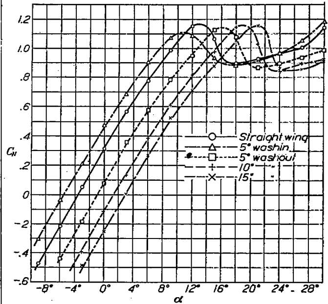
FIGURE 18.—N. A. C. A. 86 airfoil. Total normal force versus angle of attack. Effect of twist
