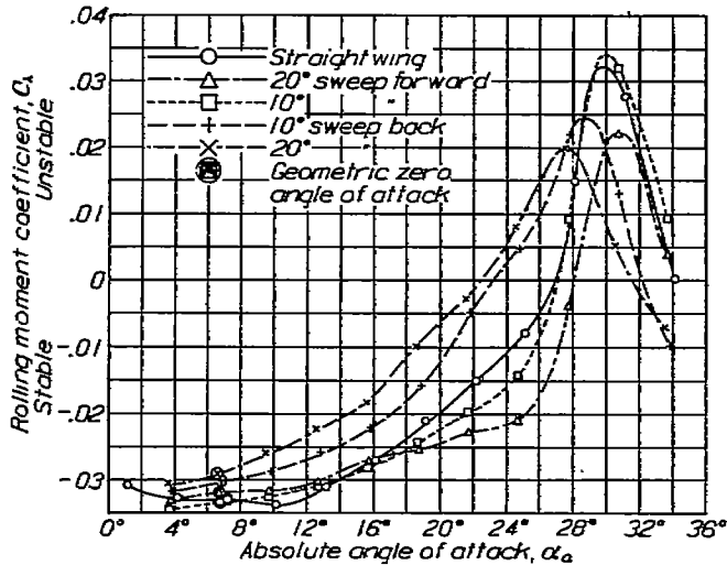
FIGURE 12.—N. A. C. A. 84 airfoil. Effect of sweepback on rolling moment due to roll at \frac{pb}{2V^2} = 0.05
