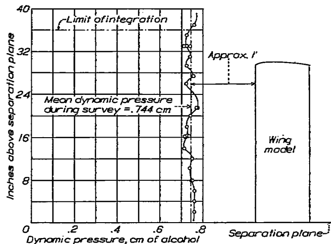
FIGURE 4.—Dynamic pressure distribution
