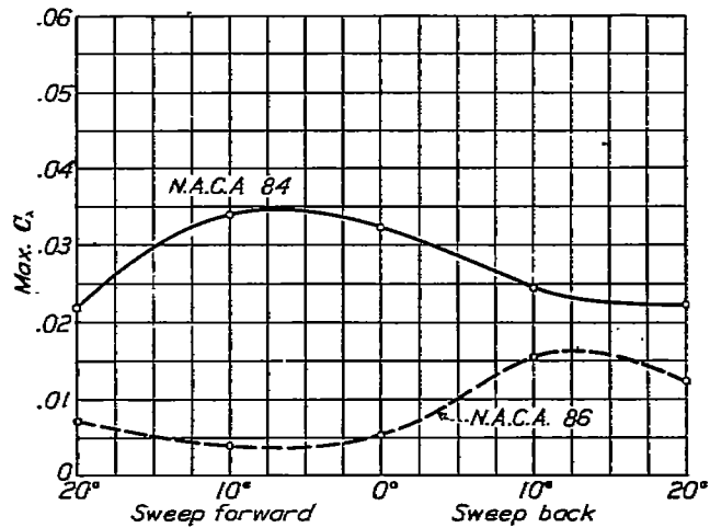
FIGURE 14.—Maximum lateral instability versus sweepback
