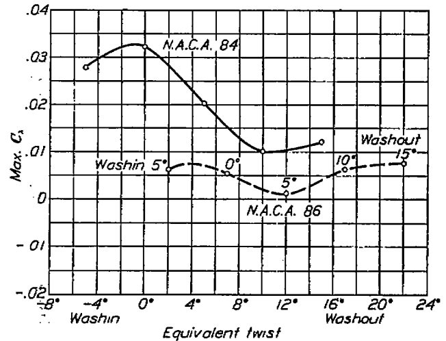
FIGURE 10.—Maximum lateral instability versus equivalent twist
