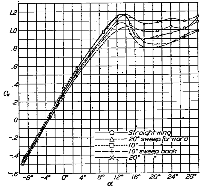
FIGURE 20.—N. A. C. A. 86 airfoil. Total normal force versus angle of attack. Effect of sweep
