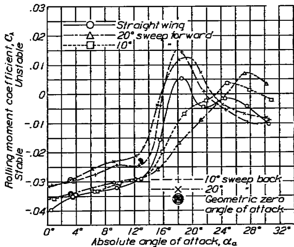
FIGURE 13.—N. A. C. A. 86 airfoil. Effect of sweepback on rolling moment due to roll at \frac{pb}{2V^2} = 0.05
