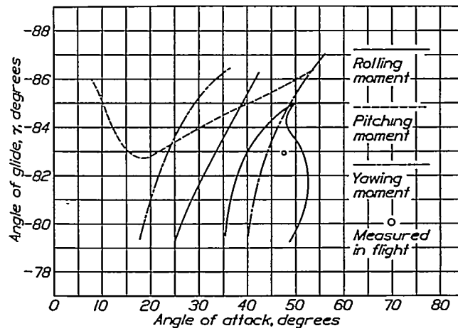
FIGURE 15.—Equilibrium of three moments, elevator down 25^\circ , ballast at c. g.
