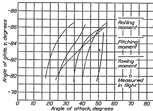
FIGURE 14.—Equilibrium of three moments, elevator up 33^\circ , ballast at c. g.
