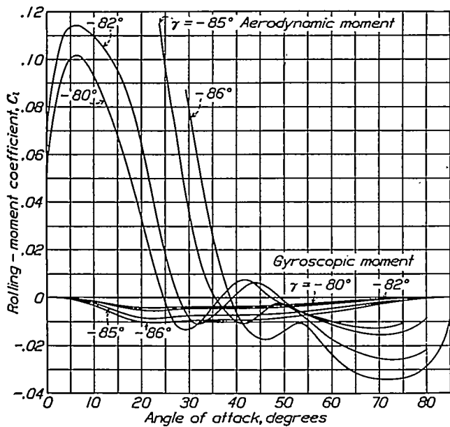
FIGURE 11.—Computed aerodynamic and gyroscopic rolling-moment coefficients, elevator up 33^\circ , ballast at c. g.
