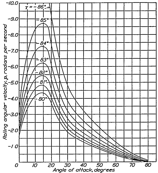
FIGURE 8.—Computed rolling angular velocity, elevator up 33°, ballast at c. g.
