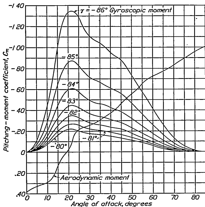
FIGURE 12.—Computed aerodynamic and gyroscopic pitching-moment coefficients, elevator up 33^\circ , ballast at c. g.
