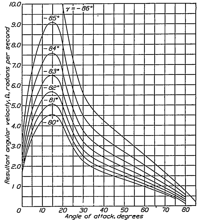
FIGURE 6.—Computed resultant angular velocity, elevator up 33°, ballast at c. g.
