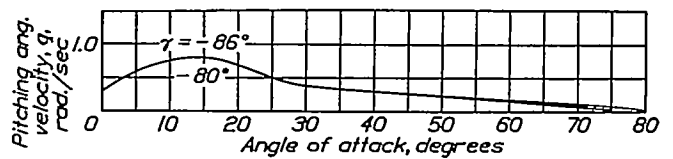
FIGURE 9.—Computed pitching angular velocity, elevator up 33°, ballast at c. g.
