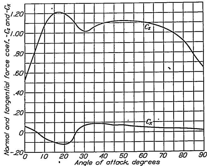
FIGURE 4.—Normal-force and tangential-force curves for the 1/12-scale model NY-1 wing cellule alone
