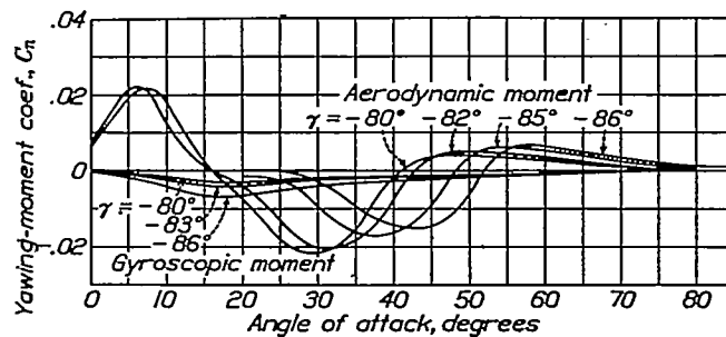
FIGURE 13.—Computed aerodynamic and gyroscopic yawing-moment coefficients, elevator up 33^\circ , ballast at c. g.
