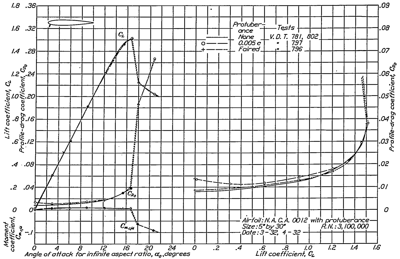
FIGURE 16.—Effect of fairing 0.005c protuberance on lower surface, 0.05c behind leading edge (position indicated by arrow)
