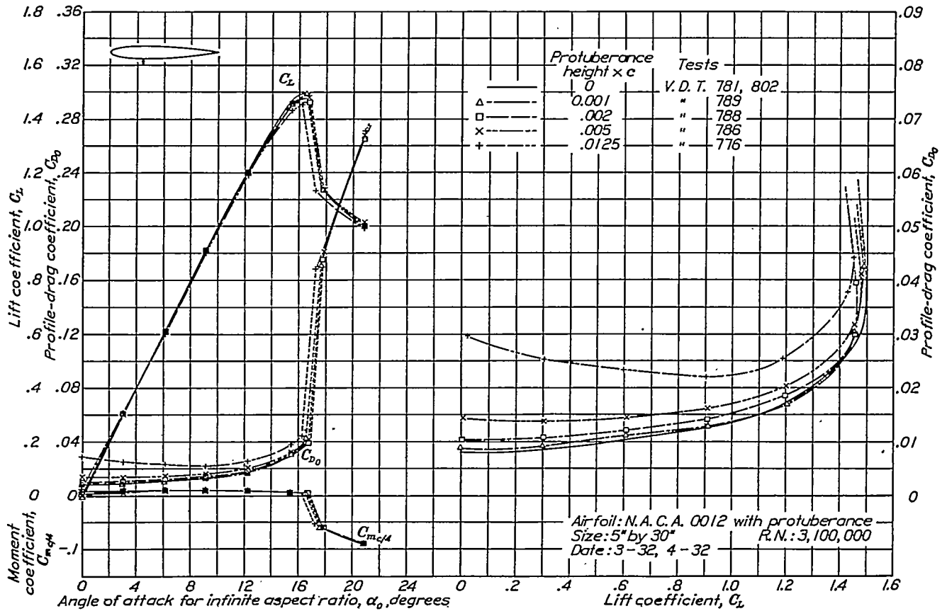
FIGURE 5.—Section characteristics for various protuberance heights. Protuberance on lower surface, 0.30c behind leading edge (position indicated by arrow)
