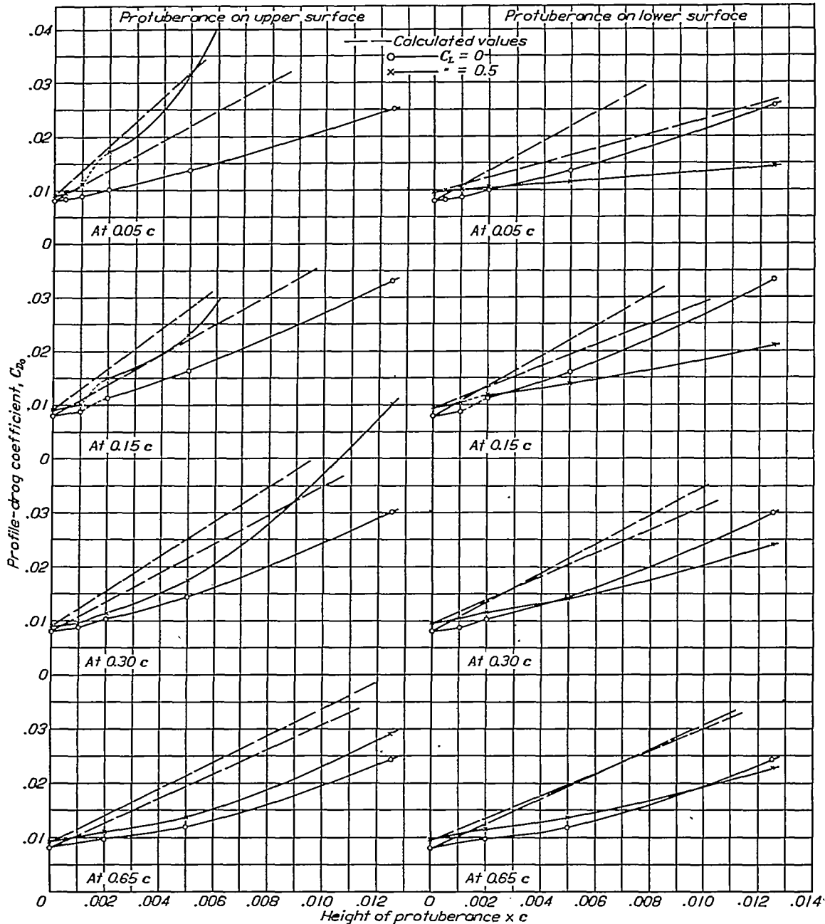
FIGURE 12.—Variation of drag with protuberance height
