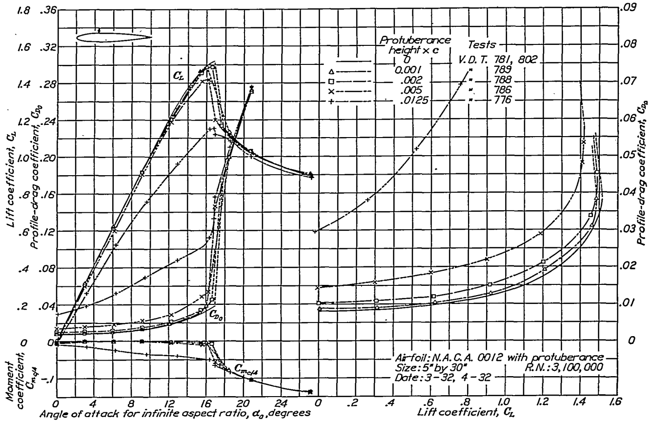
FIGURE 8.—Section characteristics for various protuberance heights. Protuberance on upper surface, 0.30c behind leading edge (position indicated by arrow)
