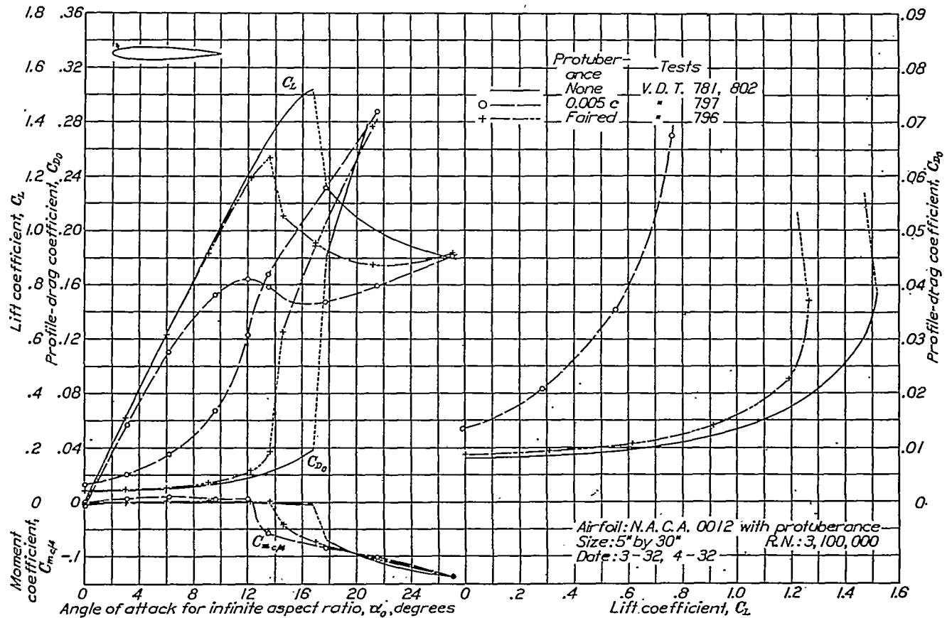
FIGURE 23.—Effect of fairing 0.005c protuberance on upper surface, 0.05c behind leading edge (position indicated by arrow)
