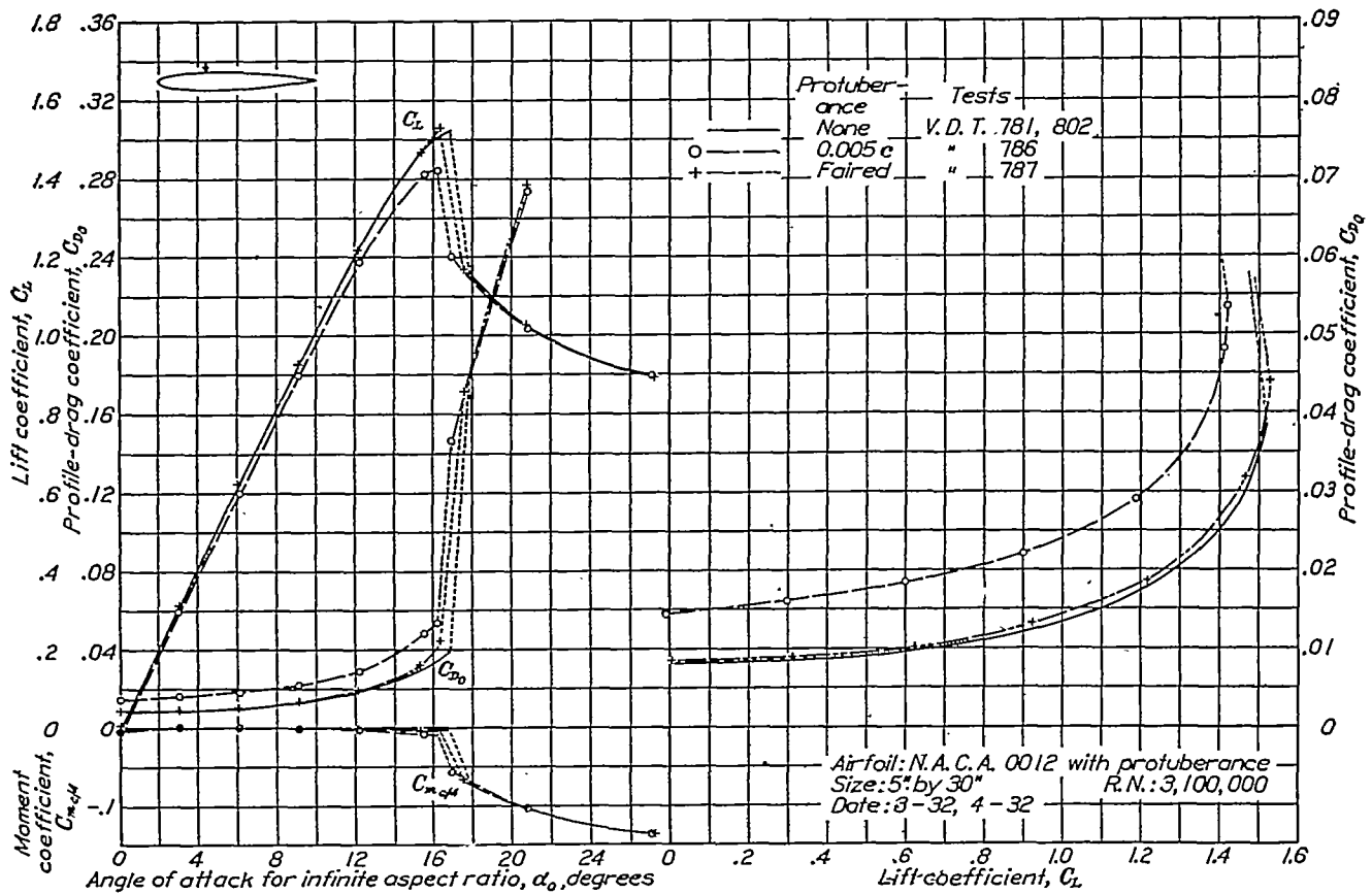
FIGURE 21.—Effect of fairing 0.005c protuberances on upper surface, 0.30c behind leading edge (position indicated by arrow)
