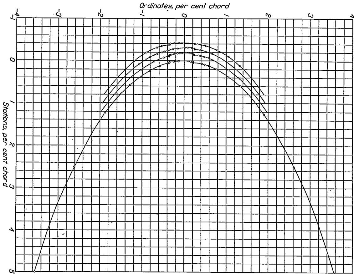
FIGURE 14.—Nose profile, measured at four representative stations along span, showing 0.004c protuberance at leading edge
