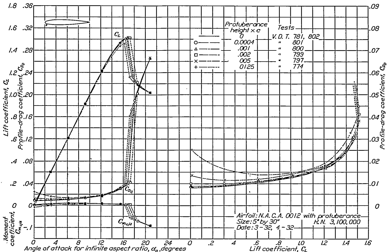
FIGURE 3.—Section characteristics for various protuberance heights. Protuberance on lower surface, 0.05c behind leading edge (position indicated by arrow)
