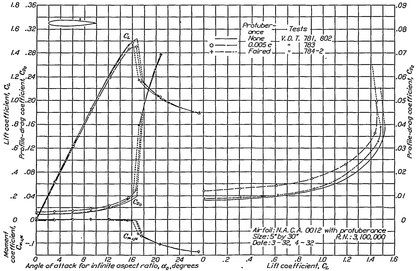
FIGURE 20.—Effect of fairing 0.005c protuberances on upper surface, 0.65c behind leading edge (position indicated by arrow)
