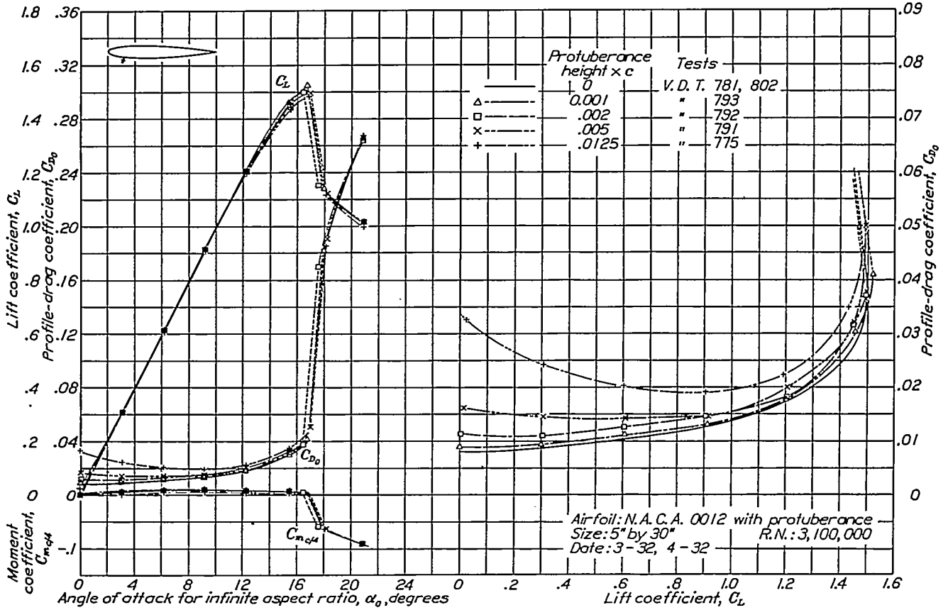
FIGURE 4.—Section characteristics for various protuberance heights. Protuberance on lower surface, 0.15c behind leading edge (position indicated by arrow)
