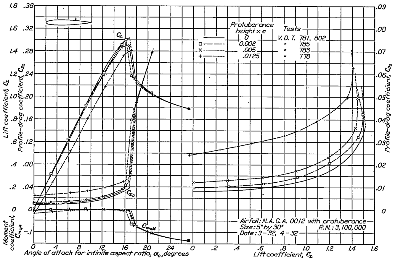
FIGURE 7.—Section characteristics for various protuberance heights. Protuberances on upper surface 0.65c behind leading edge (position indicated by arrow)
