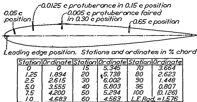
FIGURE 1.—N. A. C. A. 0012 airfoil showing protuberances
