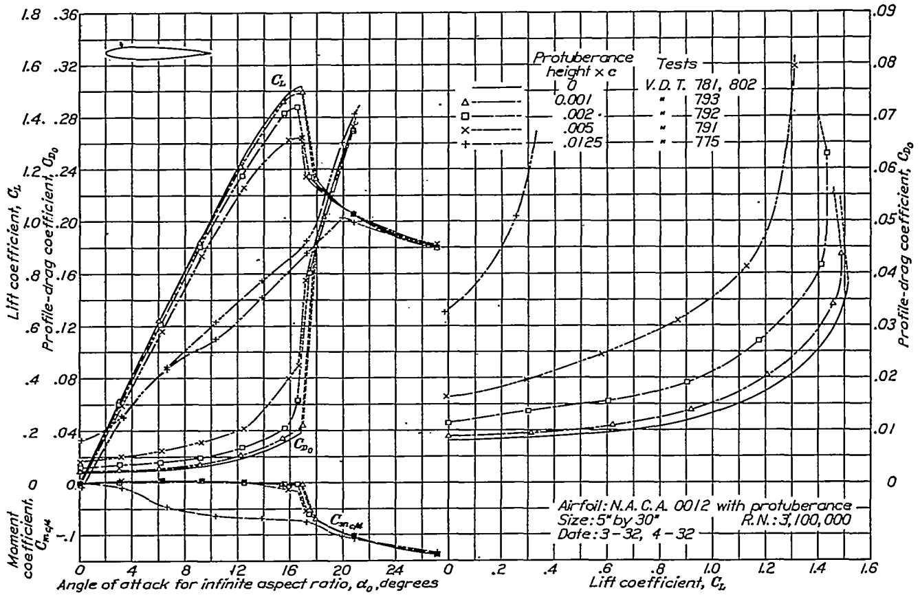
FIGURE 9.—Section characteristics for various protuberance heights. Protuberance on upper surface, 0.15c behind leading edge (position indicated by arrow)
