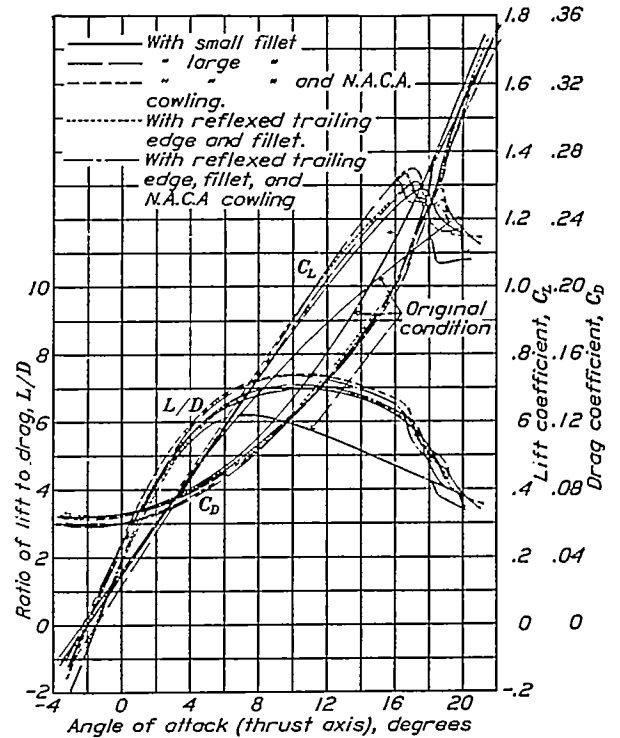
FIGURE 12.—Lift and drag of McDonnell airplane with various fillets. Corrected for tunnel effects. Power off.
