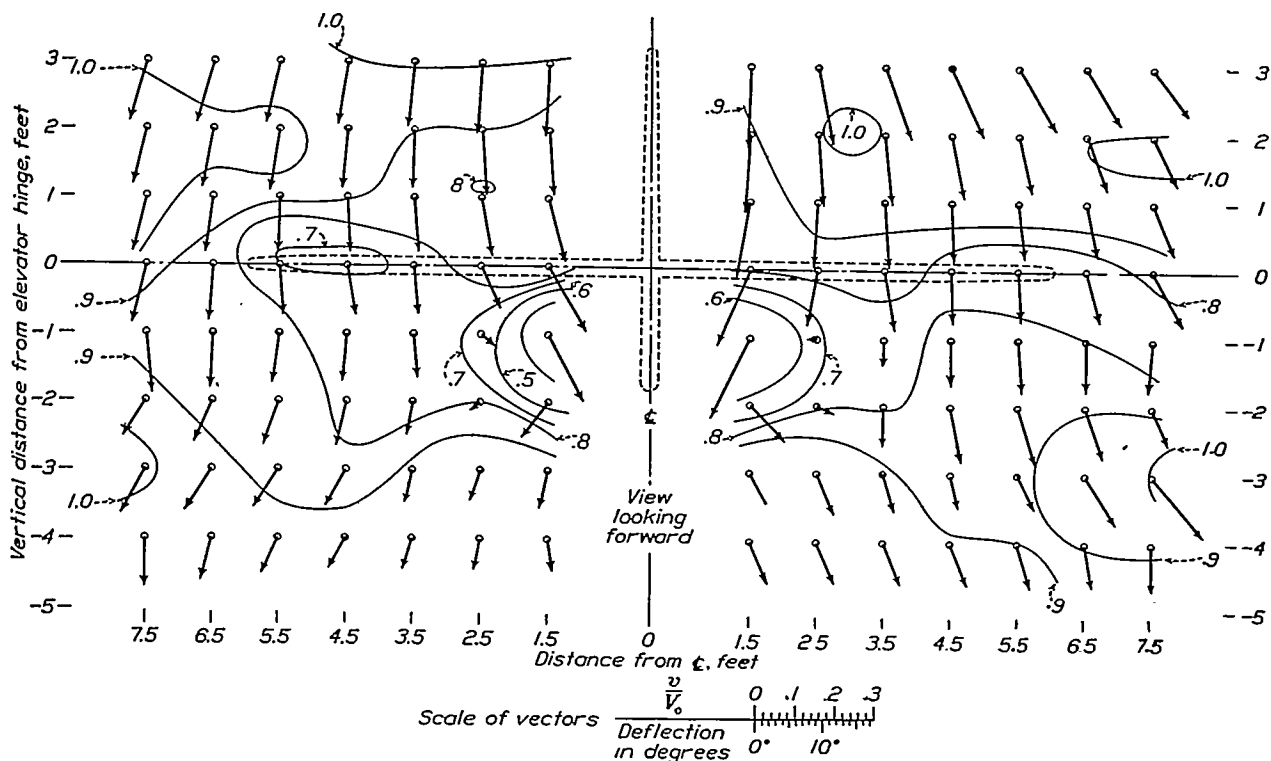
FIGURE 32.—Air flow at tail of McDonnell airplane with N.A.O.A. cowling, power off. Survey in vertical plane through elevator hinge line. The contours show the ratio of the dynamic pressure behind the airplane to the dynamic pressure in the free air stream. The vectors show the components of the velocity in the plane of the survey. Angle of attack (thrust axis)=13.9° (corrected for tunnel effects). Lift coefficient=1.153.
