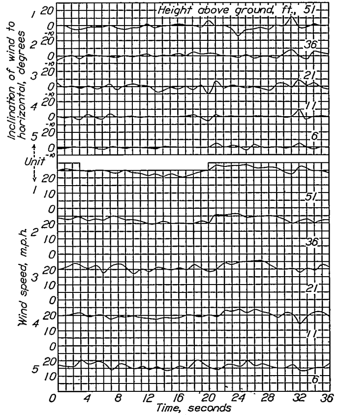
FIGURE 9.—Wind speed and inclination fluctuations for an average ground wind of 16 miles per hour. Run 2, February 21, 1933.
