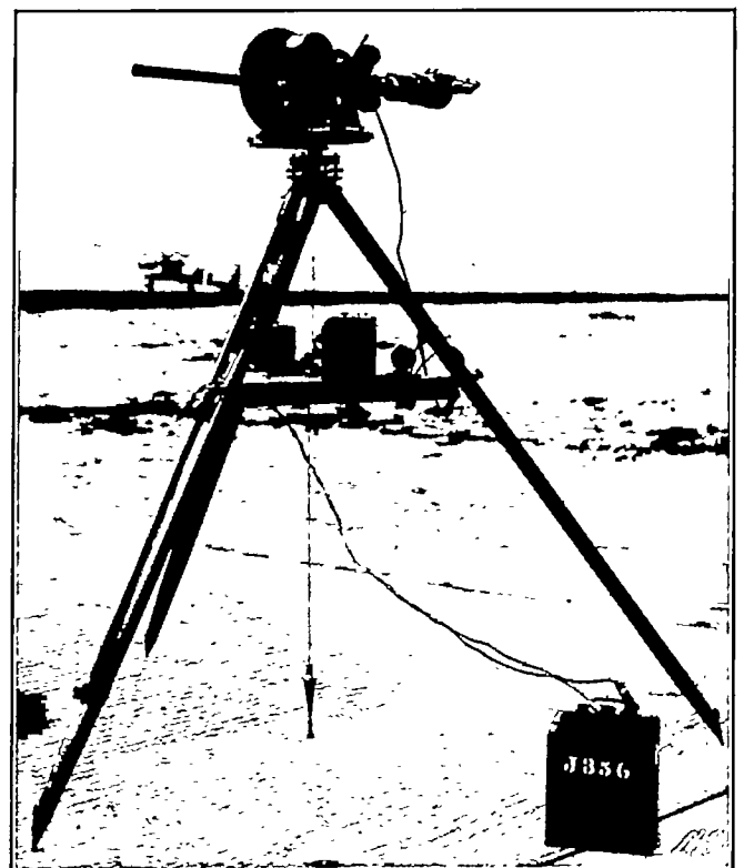
FIGURE 17.—Recording phototheodolite.
