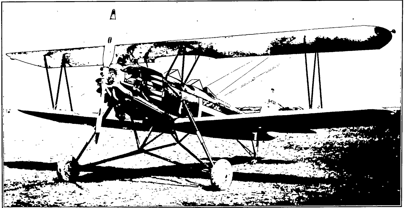
FIGURE 10.—Verville airplane modified for landing tests.
