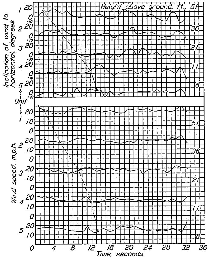
FIGURE 7.—Wind speed and inclination fluctuations for an average ground wind of 12 miles per hour. Run 4, April 13, 1932.
