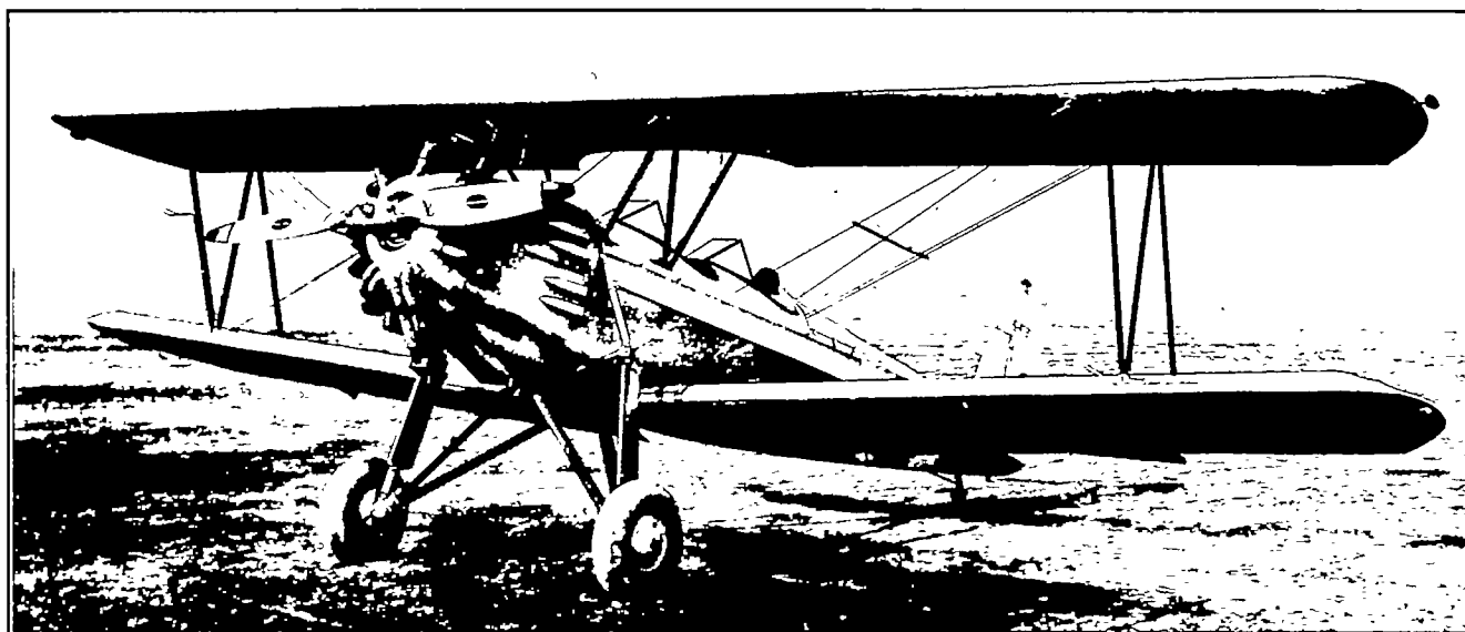
FIGURE 15.—Verville airplane with original landing gear.
