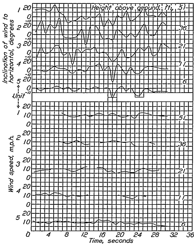
FIGURE 4.—Wind speed and inclination fluctuations for an average ground wind of 8 miles per hour. Run 3, April 6, 1932.
