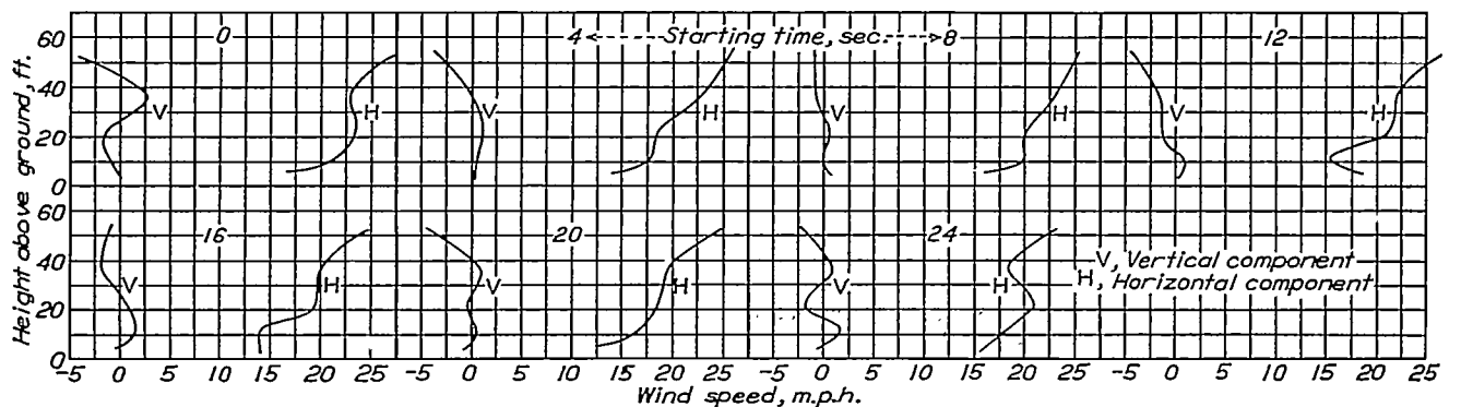
FIGURE 14.—Wind variations encountered along an assumed flight path. Run 1, February 21, 1933. (Average ground wind 16 miles per hour.) Negative wind is a descending vertical component.
