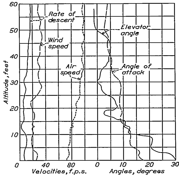
FIGURE 24.—Pancake landing in rough air.
