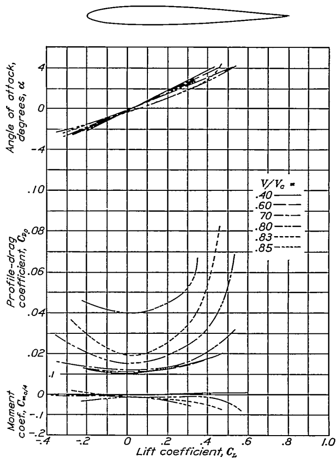
FIGURE 21.—Aerodynamic characteristics of the N.A.C.A. 0009-63 airfoil.
