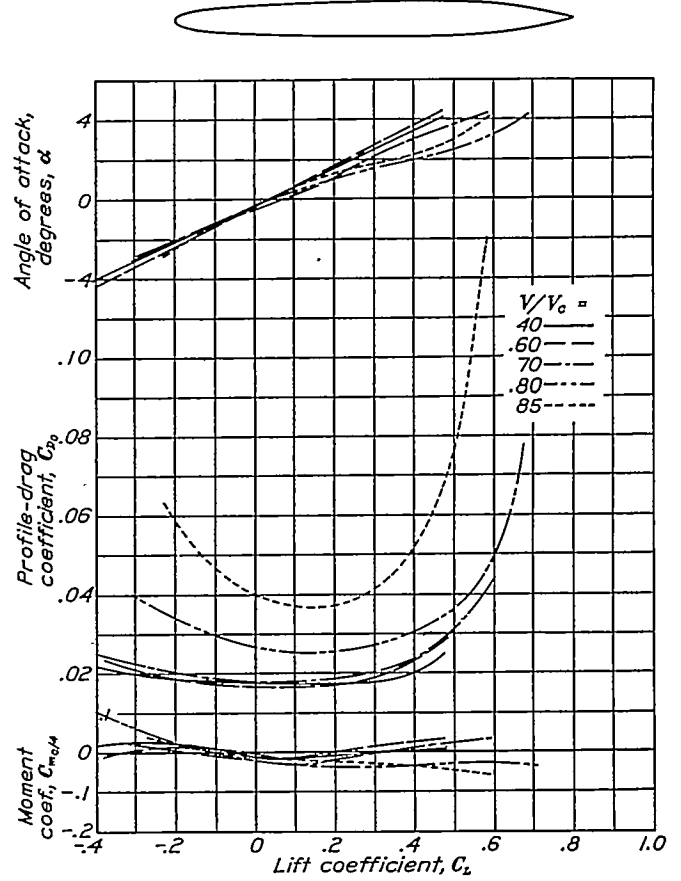
FIGURE 25.—Aerodynamic characteristics of the N.A.C.A. 0009-66 airfoil.
