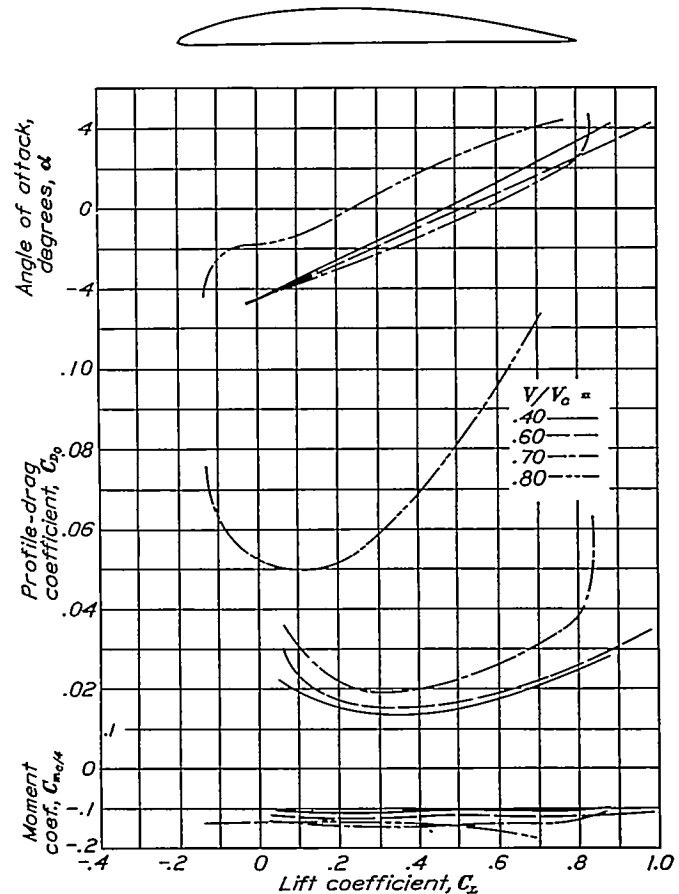
FIGURE 34.—Aerodynamic characteristics of the N.A.C.A. 4409-34 airfoil.
