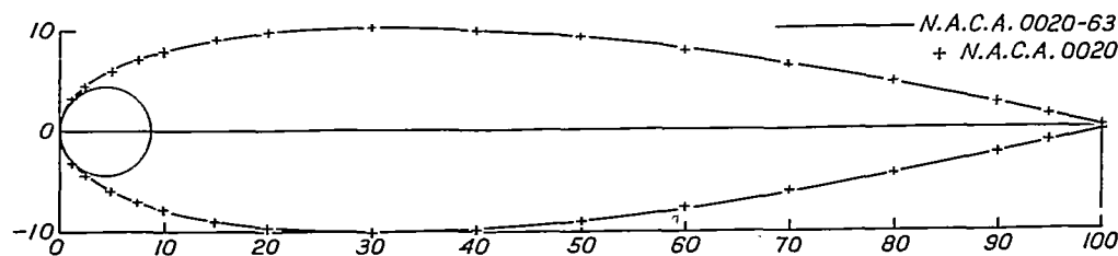
FIGURE 1.—Basic thickness distribution for airfoils tested in the high-speed wind tunnel (N.A.C.A. 0020-63) compared with basic thickness distribution for N.A.C.A. family airfoils (N.A.C.A. 0020, reference 2).
