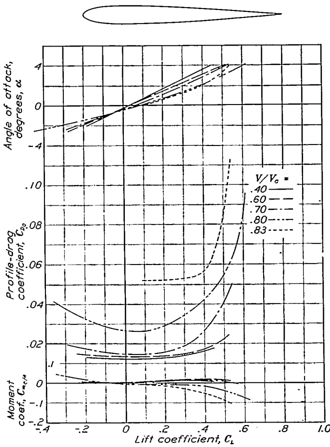
FIGURE 22.—Aerodynamic characteristics of the N.A.C.A. 0009-62 airfoil.
