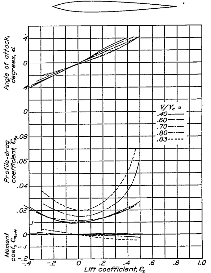
FIGURE 26.—Aerodynamic characteristics of the N.A.C.A. 0009-63 airfoil.
