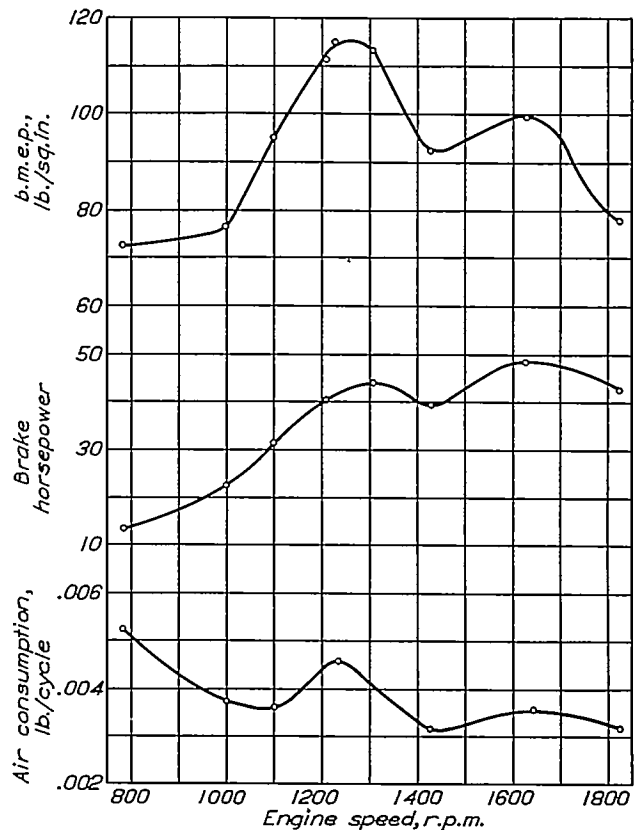
FIGURE 23.—Effect of speed on gross engine performance. Scavenging pressure 1 inch of mercury; maximum cylinder pressure, 1,000 pounds per square inch; fuel consumption, 0.50 pound per brake horse power-hour.
