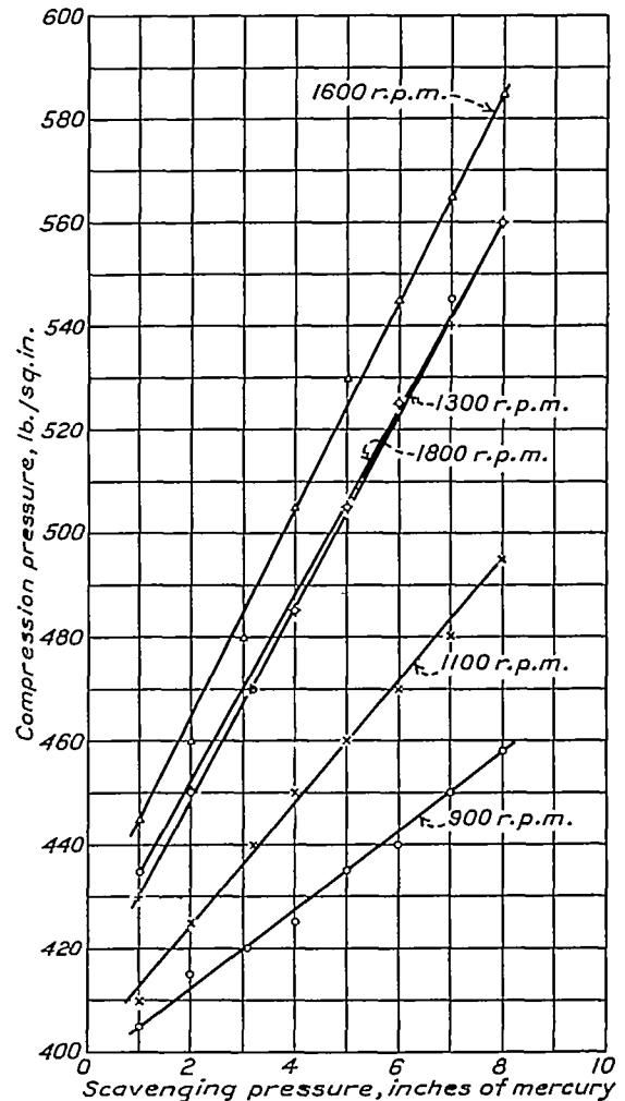
FIGURE 20.—Variation of compression pressure with engine speed and scavenging pressure.
