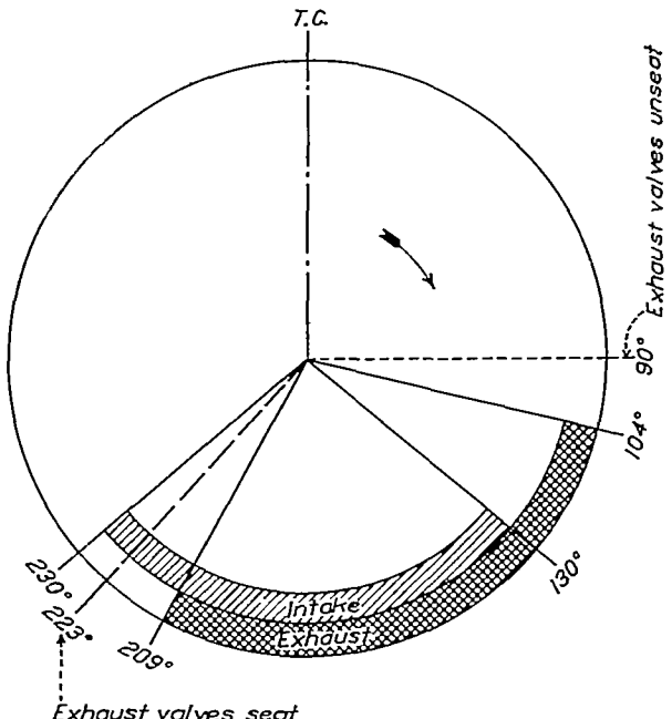
FIGURE 19.—Timing diagram of the water-cooled test engine with compression ignition.
