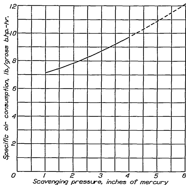
FIGURE 25.—Effect of scavenging pressure on specific air consumption. Engine speed, 1,270 r.p.m.; specific fuel consumption, 0.50 pound per brake horsepower-hour.
