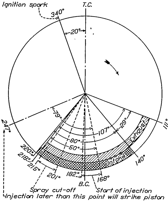
FIGURE 5.—Timing diagram of the air-cooled test engine.
