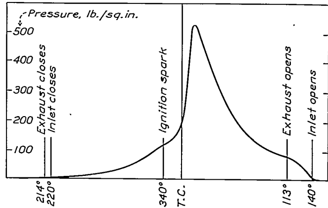
FIGURE 11.—Pressure-time card of the air-cooled test engine. Engine speed, 1,020 r.p.m.; scavenging pressure, 8 inches of mercury; l.m.a.p., 133 pounds per square inch.
