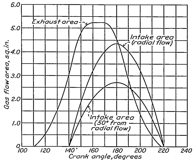
FIGURE 6.—Gas-flow area diagram of the air-cooled test engine.
