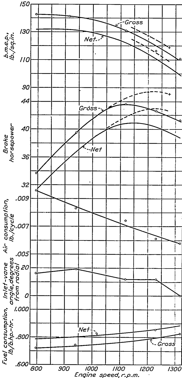
FIGURE 10.—Effect of speed on maximum power performance of the air-cooled test engine. Scavenging pressure, 8 inches of mercury; dotted line, exhaust opens 105° after top center.
