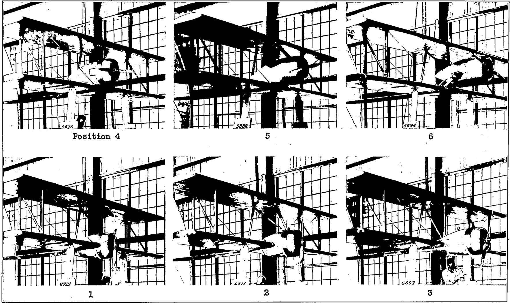
FIGURE 5.—Biplane-nacelle combinations with nacelle near lower wing.
