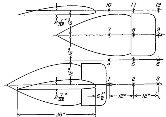
FIGURE 3.—Biplane-nacelle test locations.
