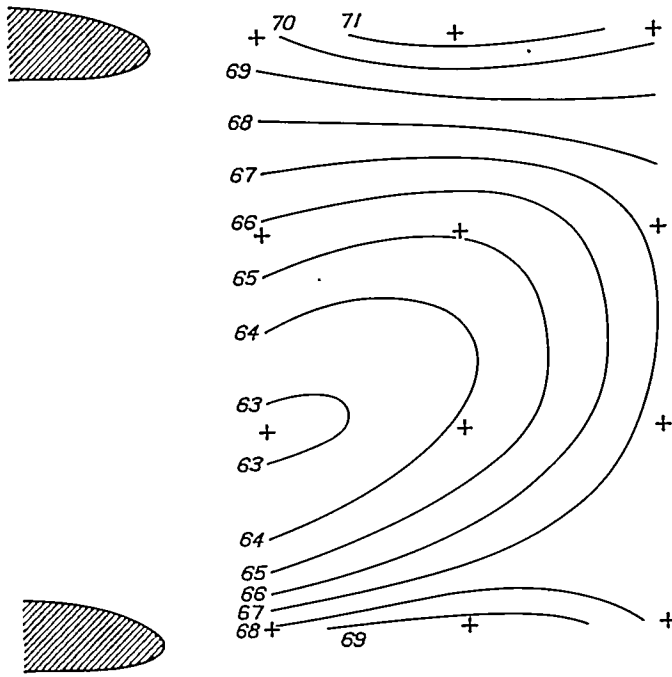
FIGURE 14.—Net efficiency (percent) for climbing condition. ( C_L=0.430 ; propeller set 17^\circ at 0.75 R ; \eta taken at V/nD=0.42 .)
