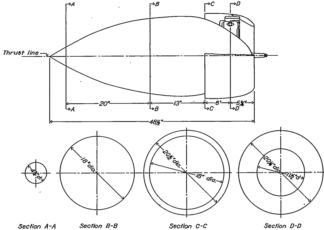
FIGURE 1.—N.A.C.A. cowled nacelle and engine assembly.
