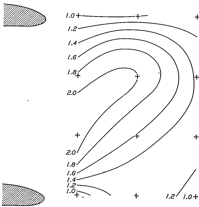
FIGURE 13.—Nacelle drag efficiency factor (percent) for climbing condition. ( C_L=0.430 ; propeller set 17^\circ at 0.75 R ; \eta taken at V/nD=0.42 .)
