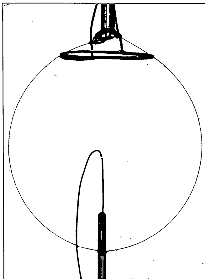
FIGURE 4.—Bubble suspended and ready to be fired.
