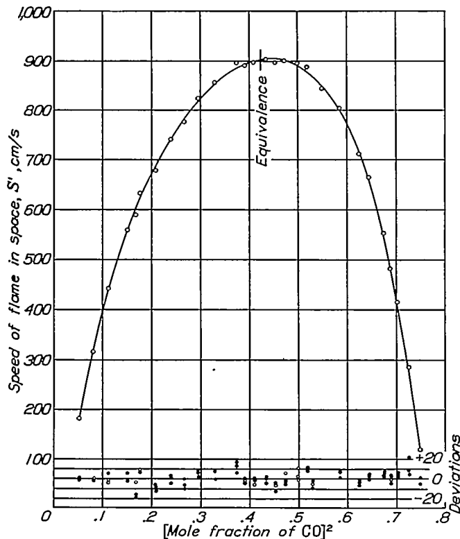
FIGURE 6.—Speed of flame in space by the bubble method (mole fraction of water=0.0331).
