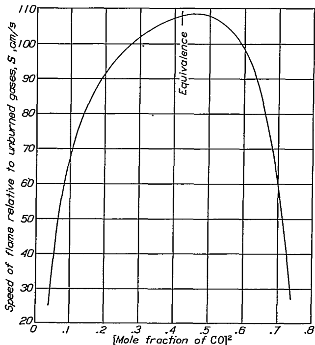
FIGURE 8.—Speed of flame relative to the active gases.
