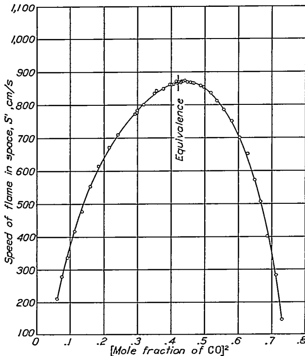
FIGURE 5.—Speed of flame in space by the constant-volume method (mole fraction of water=0.0269).
