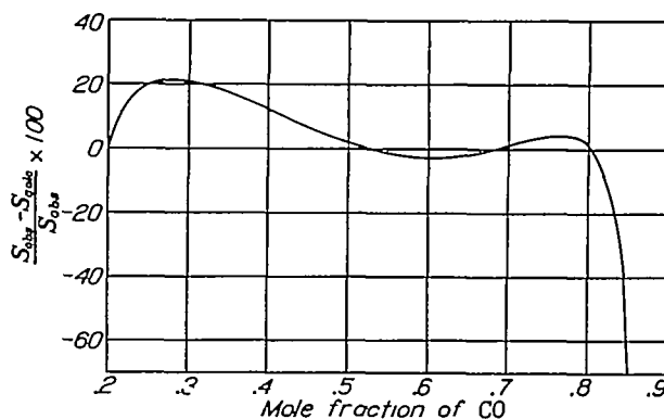
FIGURE 9.—Deviations of the observed values of S from the equation S = 820 [\text{CO}]^2 [\text{O}_2] .
