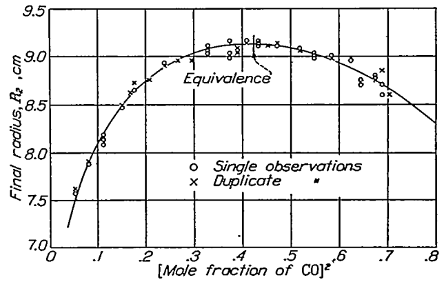
FIGURE 7.—Final radii by the bubble method.
