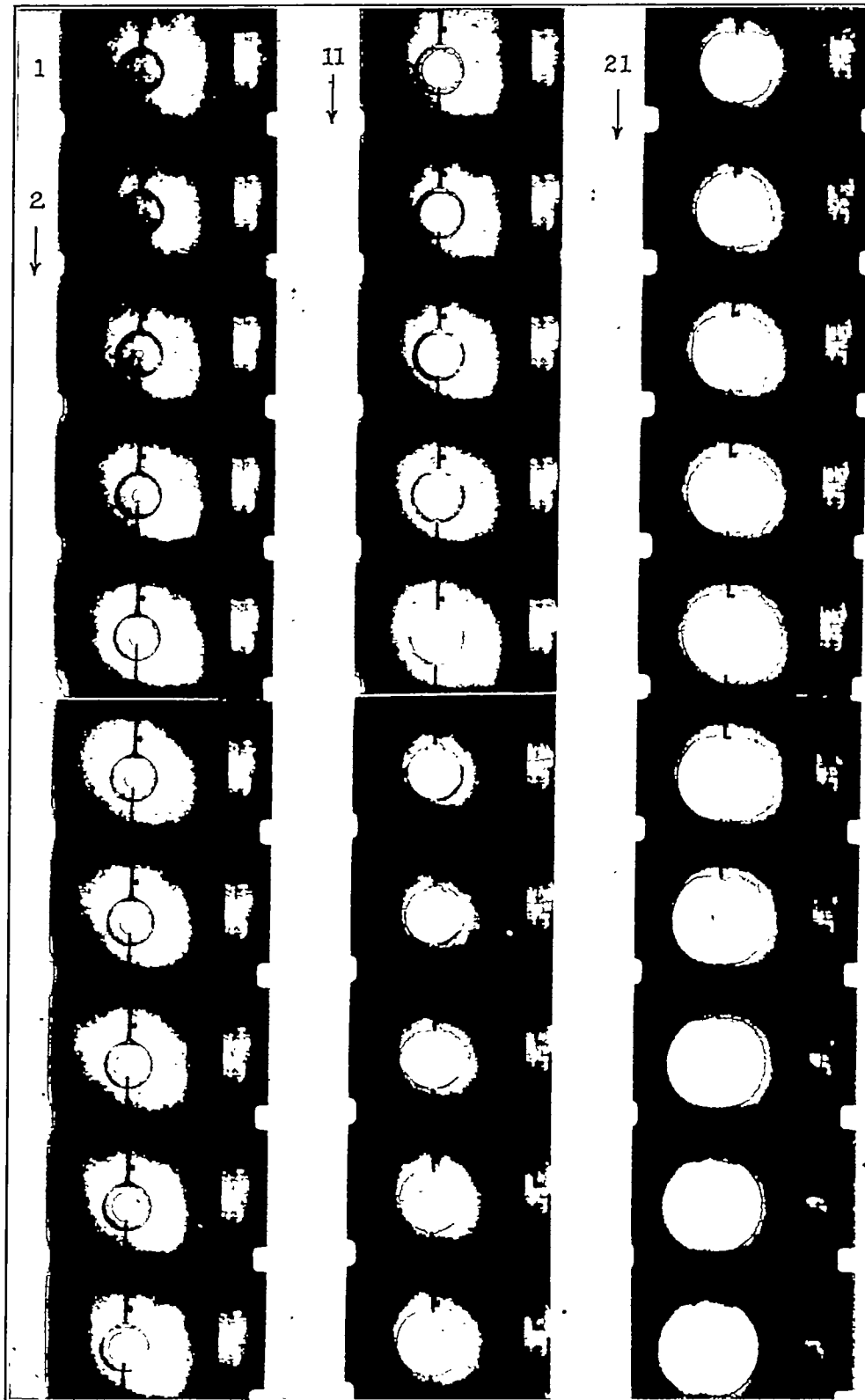
FIGURE 3.—High-speed motion-picture record of a bubble explosion (1,610 frames per second).
