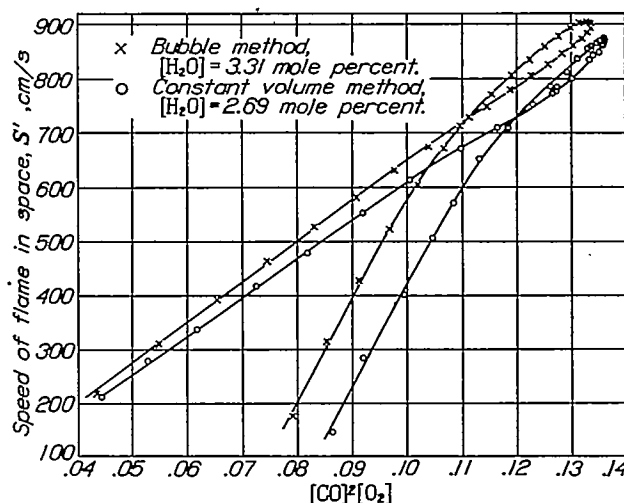
FIGURE 10.—Values of the speed of flame in space plotted against the mass action product.
