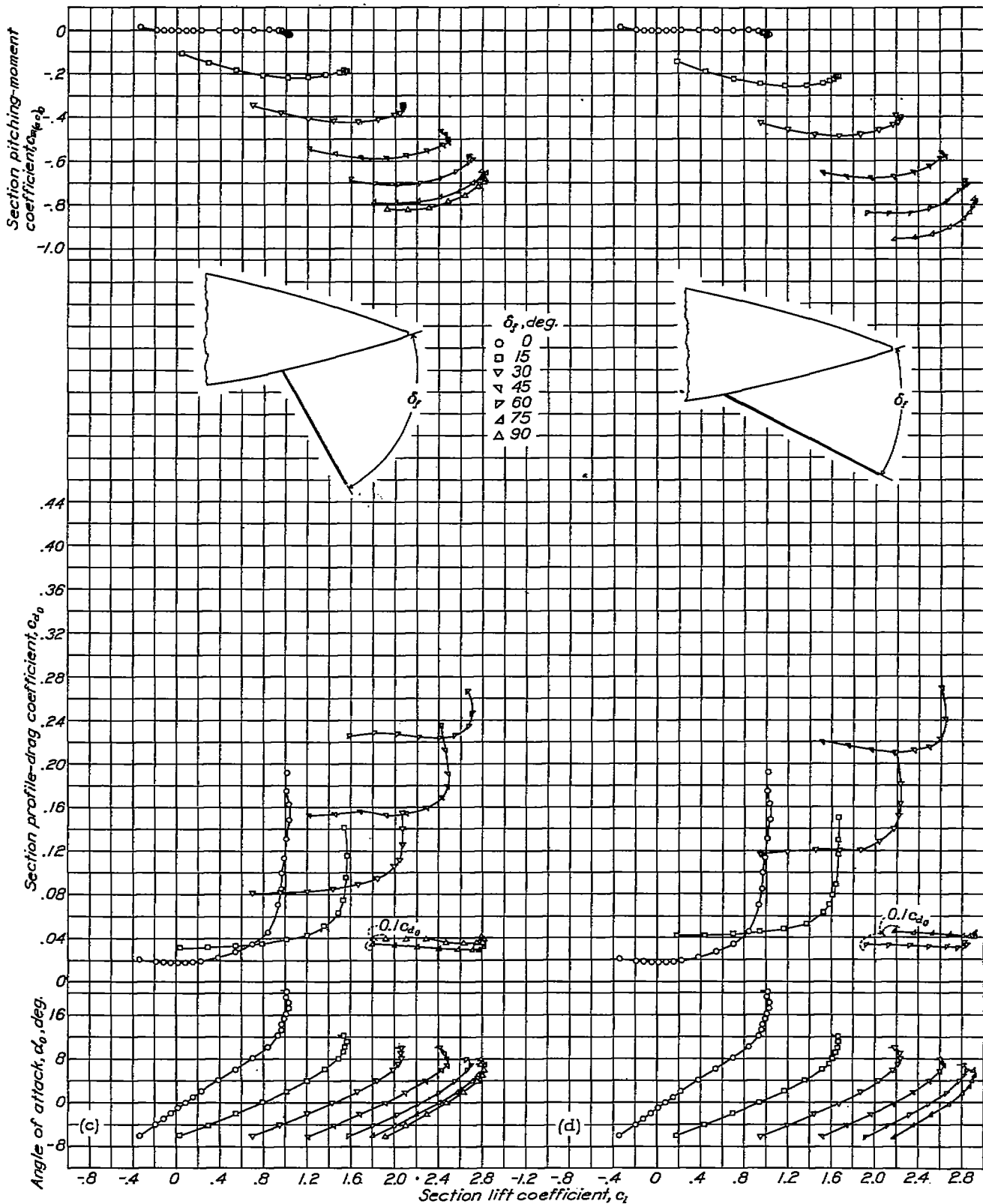
(c) The 0.30c m split flap.
