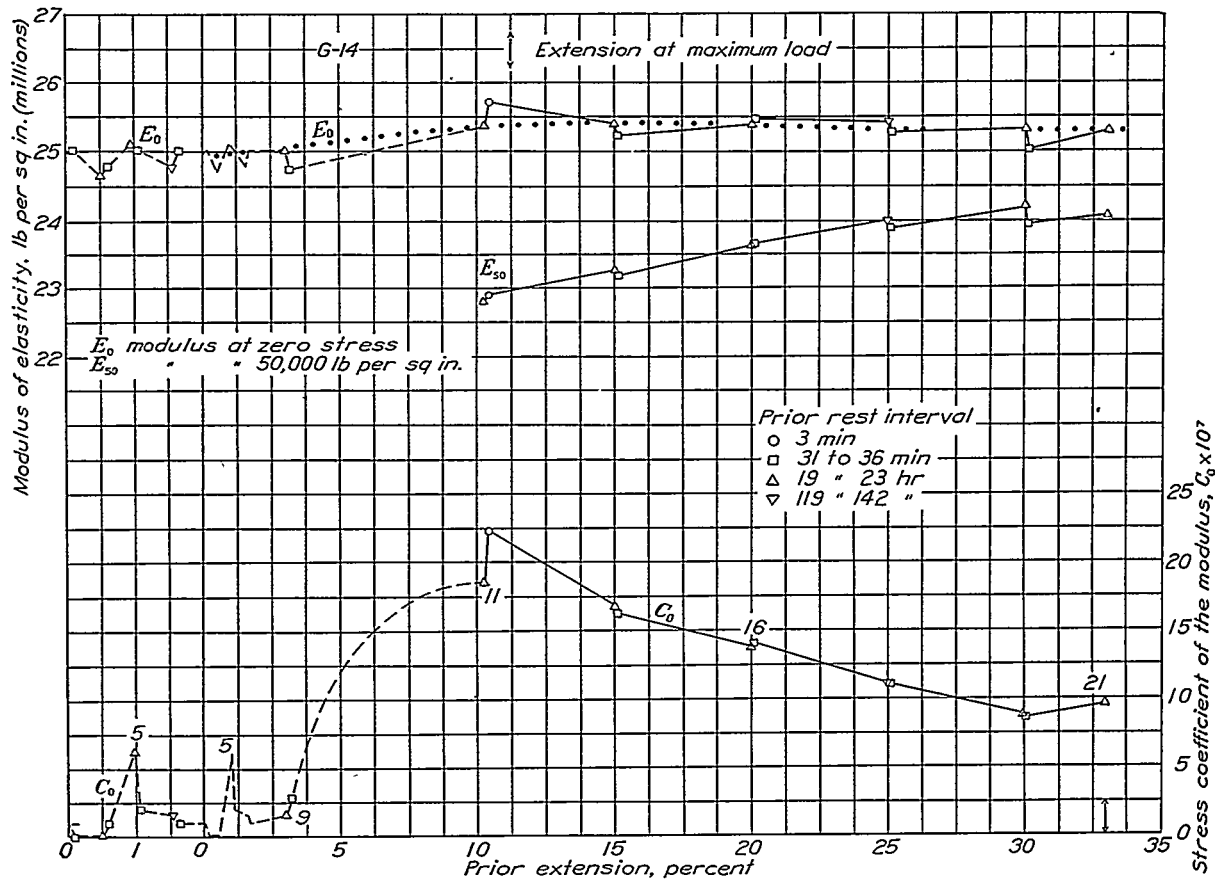
FIGURE 6.—Influence of prior plastic extension on the modulus of elasticity and on its stress coefficient for monel metal G-14; cold-drawn; annealed at 1,400° F
