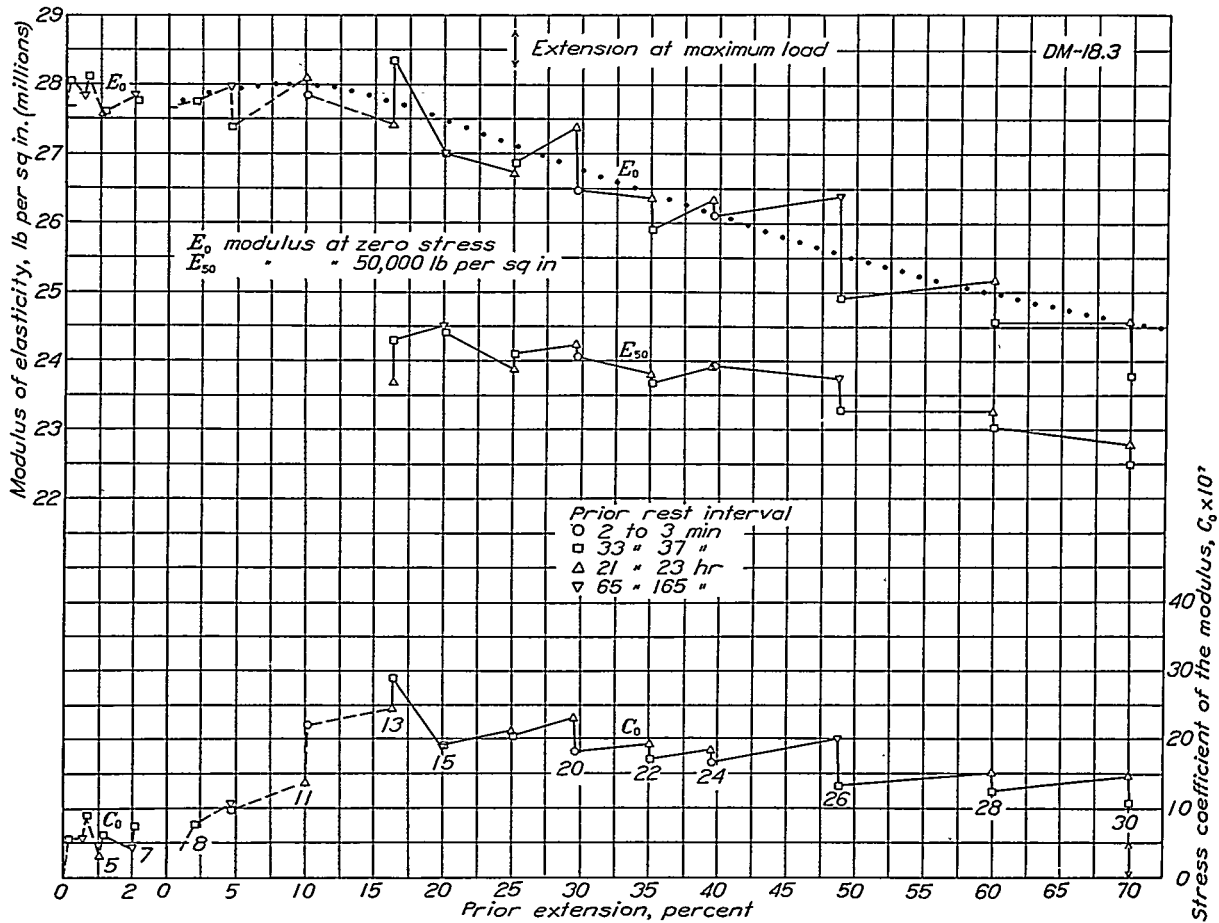
FIGURE 27.—Influence of prior plastic extension on the modulus of elasticity and on its stress coefficient for 18:8 chromium-nickel steel DM-18.3; cold-drawn; annealed at 1,830° F.
