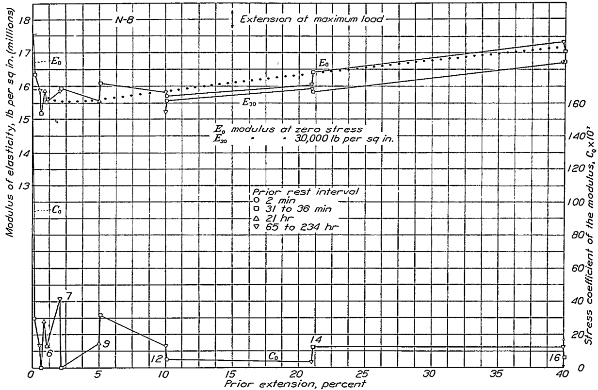
FIGURE 45.—Influence of prior plastic extension on the modulus of elasticity and on its stress coefficient for copper N-8; cold-rolled; annealed at 800° F.
