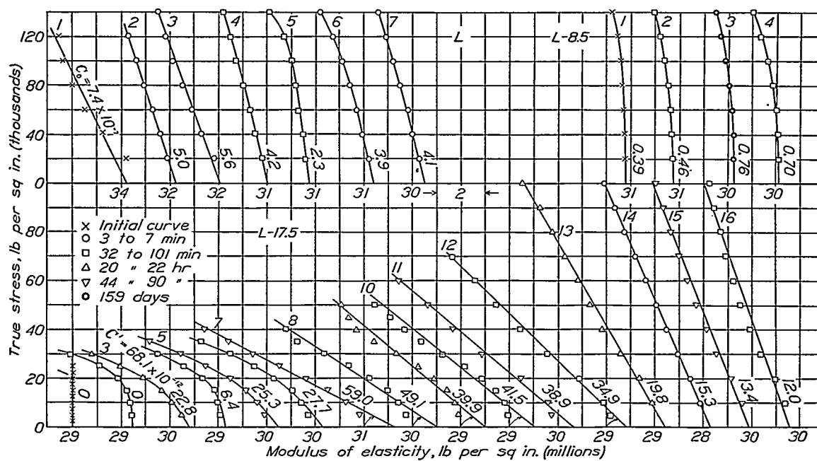
FIGURE 15.—Influence of prior plastic extension on the stress-modulus line for Inconel.
