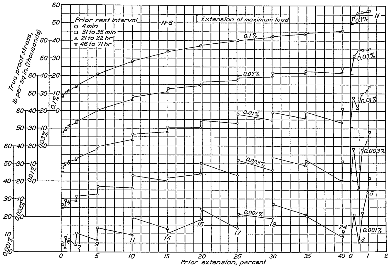
FIGURE 39.—Influence of prior plastic extension on stress-deviation and stress-set curves for copper N-6; cold-rolled; annealed at 600° F.
