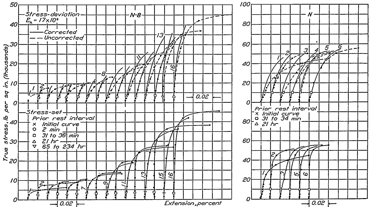
Copper N-8; cold-rolled; annealed at 800° F. Copper N; cold-rolled; as received.
