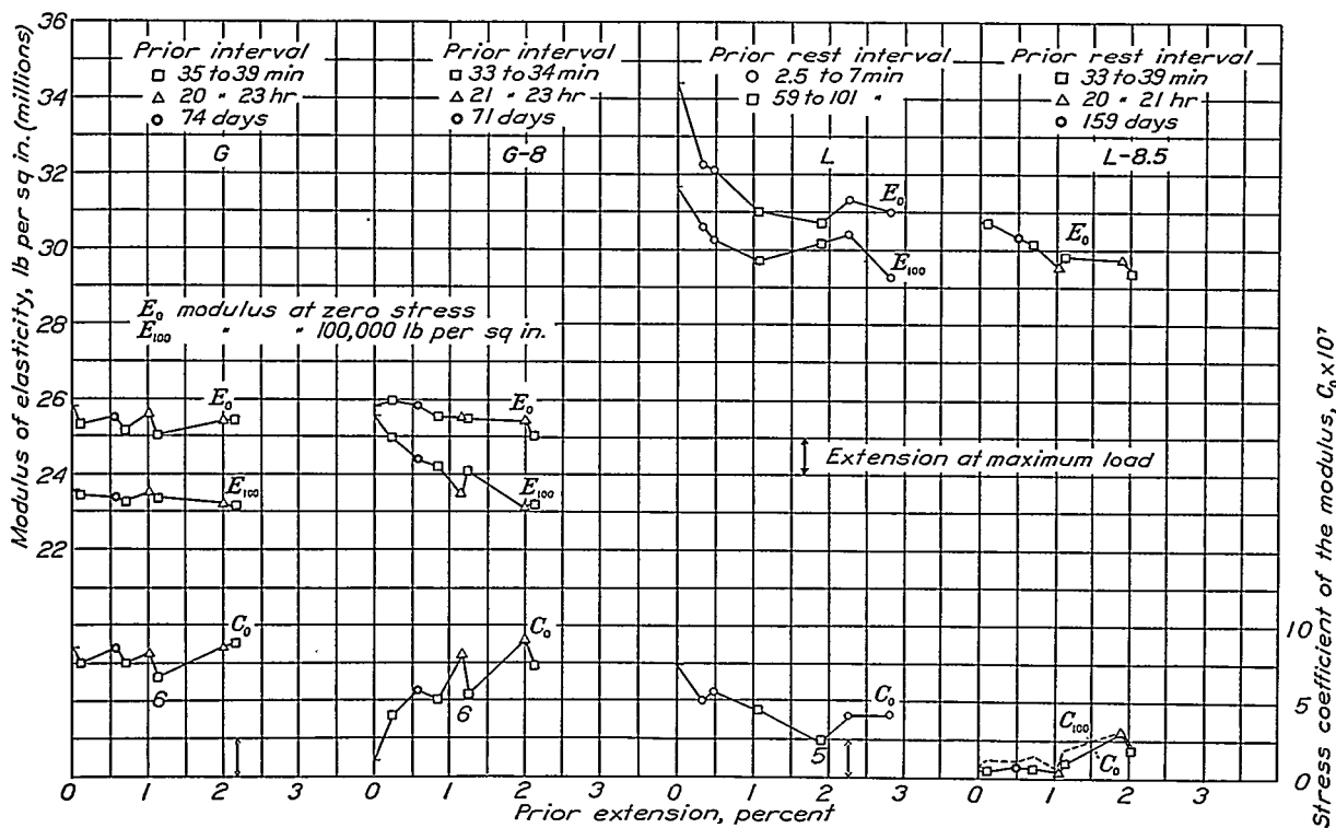
Monel metal G; cold-drawn; as received. Monel metal G-8; cold-drawn; annealed at 800° F. Inconel L; cold-drawn; as received. Inconel L-8.5; cold-drawn; annealed at 850° F. FIGURE 12. —Influence of prior plastic extension on the modulus of elasticity and on its stress coefficient for work-hardened monel metal and Inconel.
