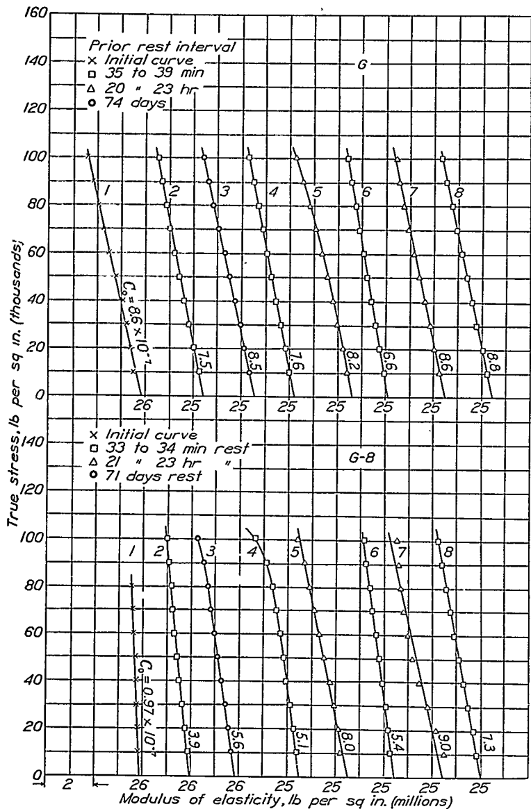
Monel metal G; cold-drawn; as received. Monel metal G-8; cold-drawn; annealed at 800° F. FIGURE 11. —Influence of prior plastic extension on the stress-modulus line for work-hardened monel metal.
