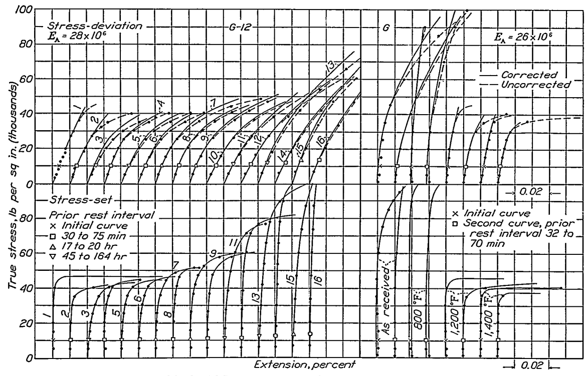
Monel metal G-12; cold-drawn; annealed at 1,200° F. Monel metal G; cold-drawn; annealed at indicated temperature.
