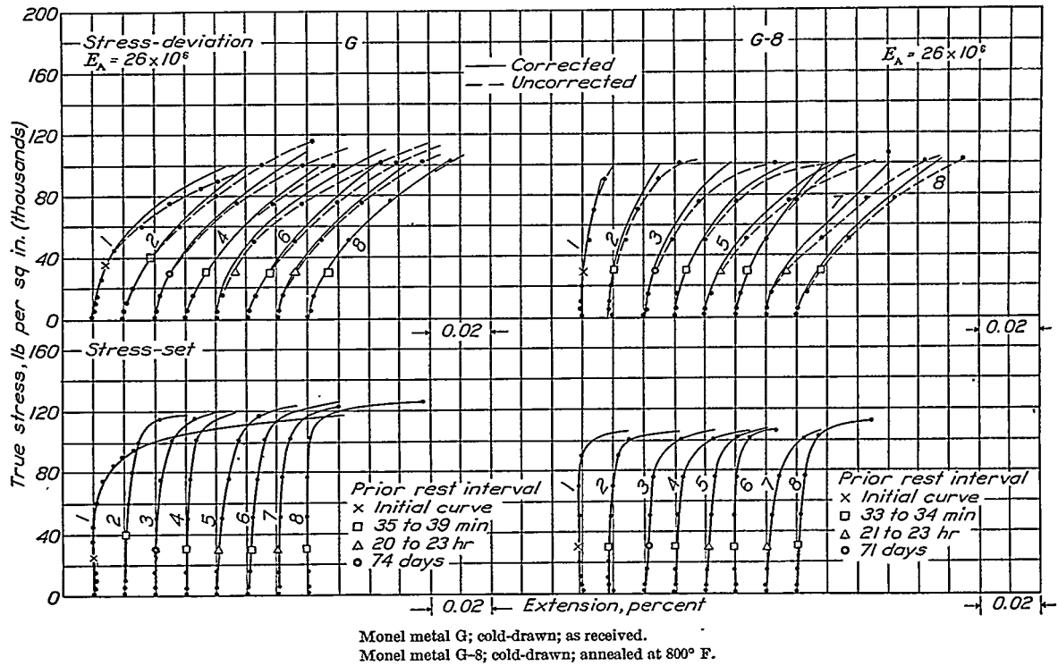
FIGURE 9.—Influence of prior plastic extension on stress-deviation and stress-set curves for work-hardened monel metal.
