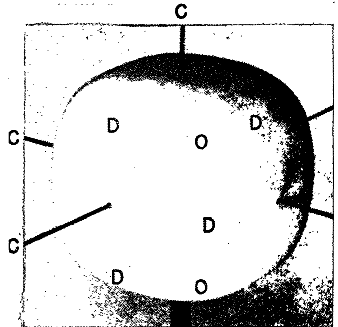
FIGURE 50.—Directional variation of the tensile modulus of elasticity of a crystal of aluminum.
