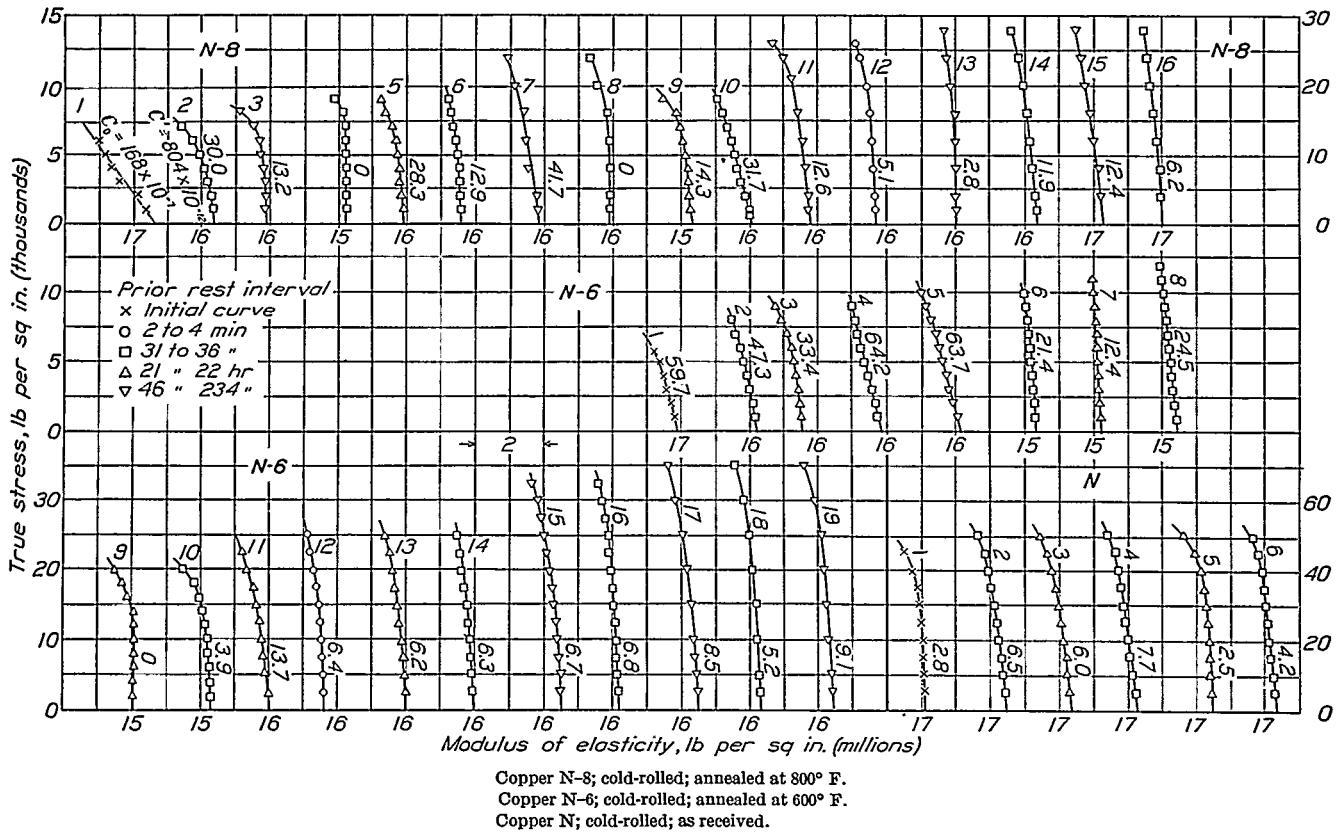
FIGURE 43.—Influence of prior plastic extension on the stress-modulus line for copper.
