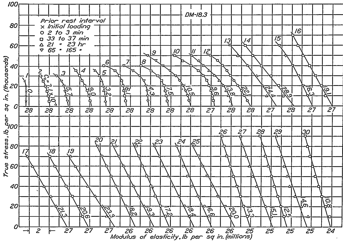
FIGURE 26.—Influence of prior plastic extension on the stress-modulus line for 18:8 chromium-nickel steel DM-18.3; cold-drawn; annealed at 1,830° F.
