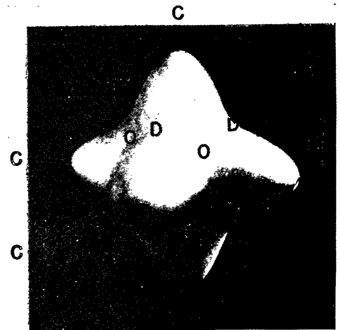
FIGURE 52.—Directional variation of the shear modulus of elasticity of a crystal of alpha iron.
