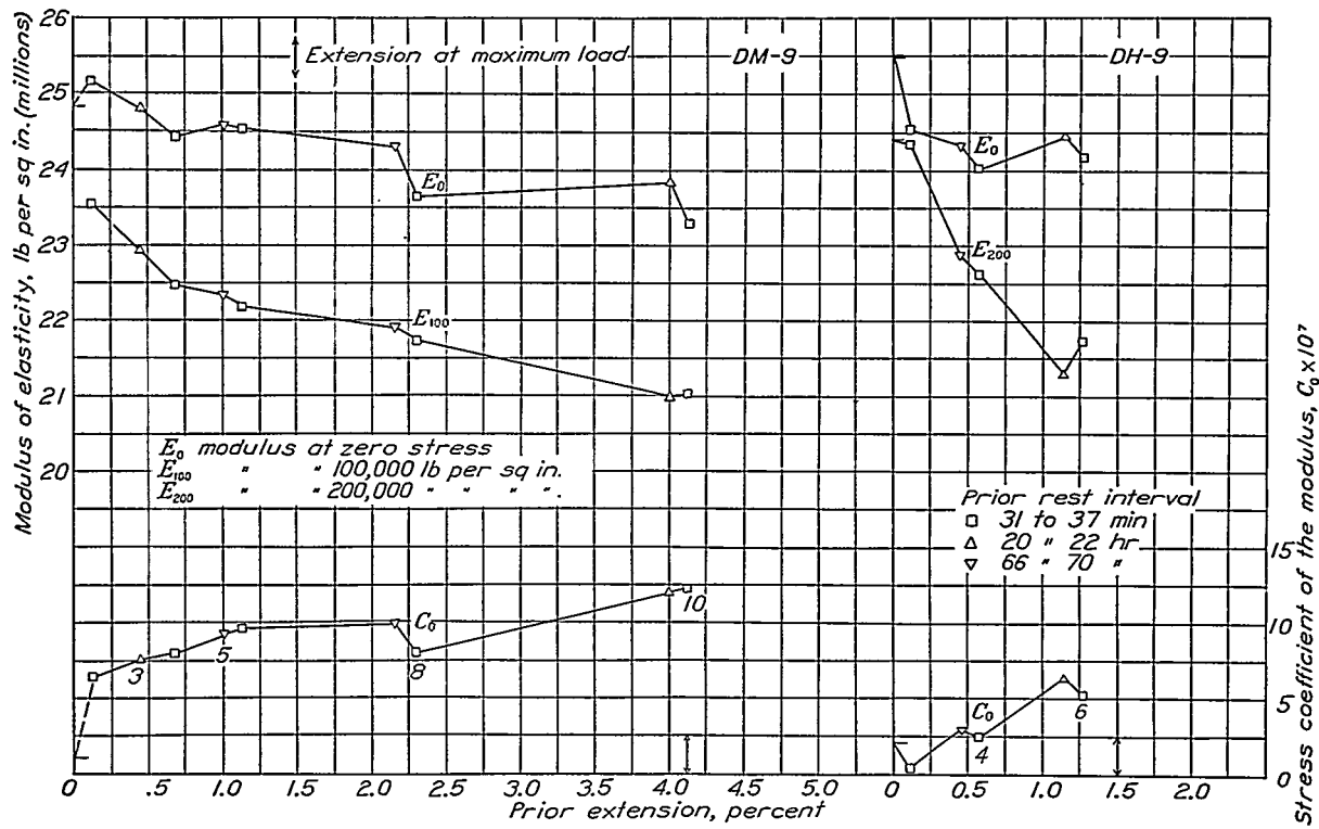
FIGURE 28.—Influence of prior plastic extension on the modulus of elasticity and on its stress coefficient for 18:8 chromium-nickel steel; cold-drawn; annealed at 900° F. for relief of internal stress.
