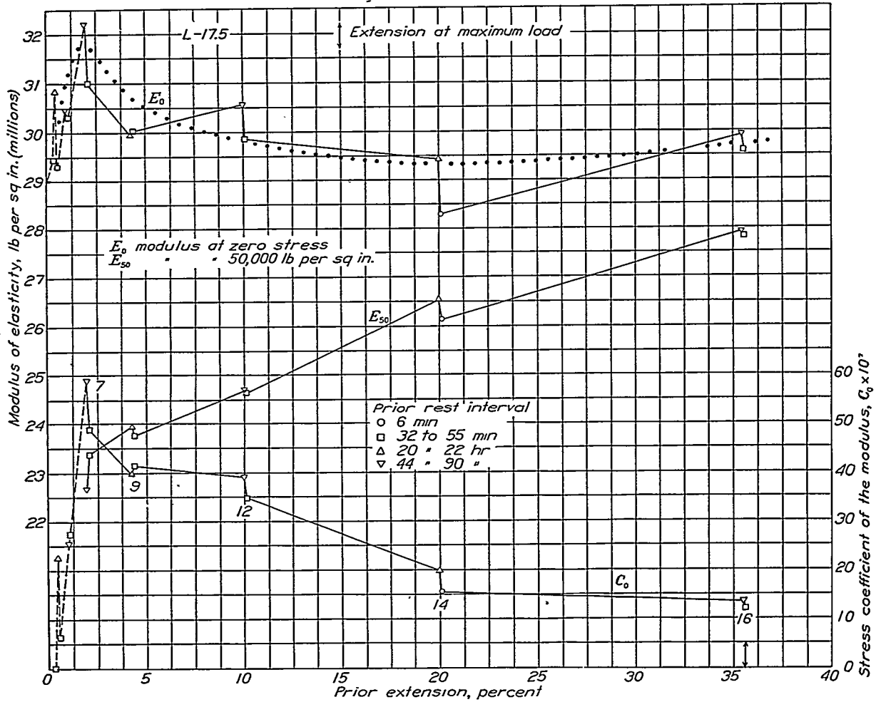
FIGURE 16.—Influence of prior plastic extension on the modulus of elasticity and on its stress coefficient for Inconel L-17.5; cold-drawn; annealed at 1,750° F.
