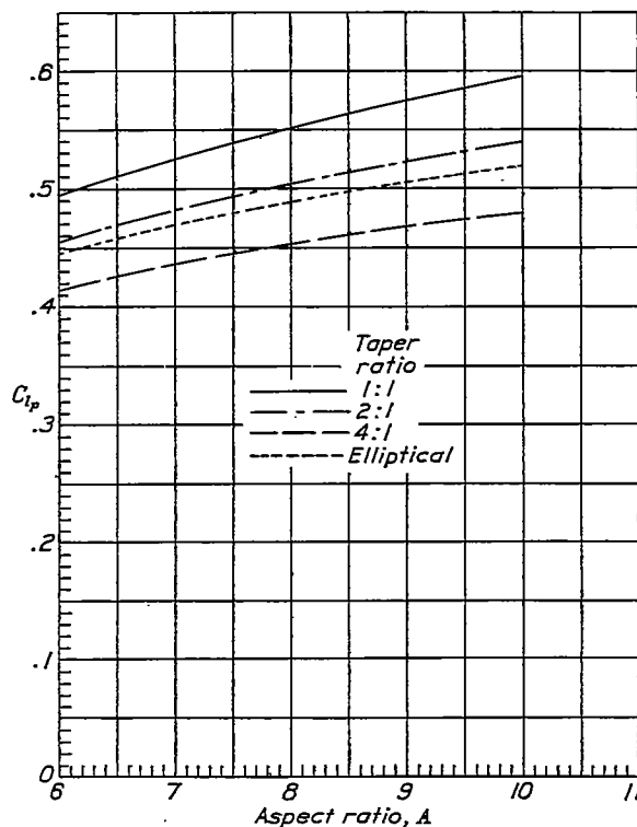
FIGURE 2.—Variation of C_{l_p} with aspect ratio and taper ratio (from reference 3).
