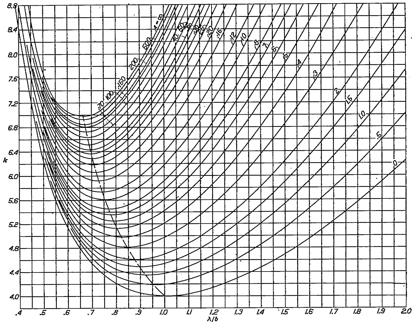
FIGURE 3.—General design chart giving values of k for equal restraint coefficients \epsilon on each side edge of the plate. f_{cr} = \frac{k\pi^2 E T^2}{12(1-\mu^2) b^2}
