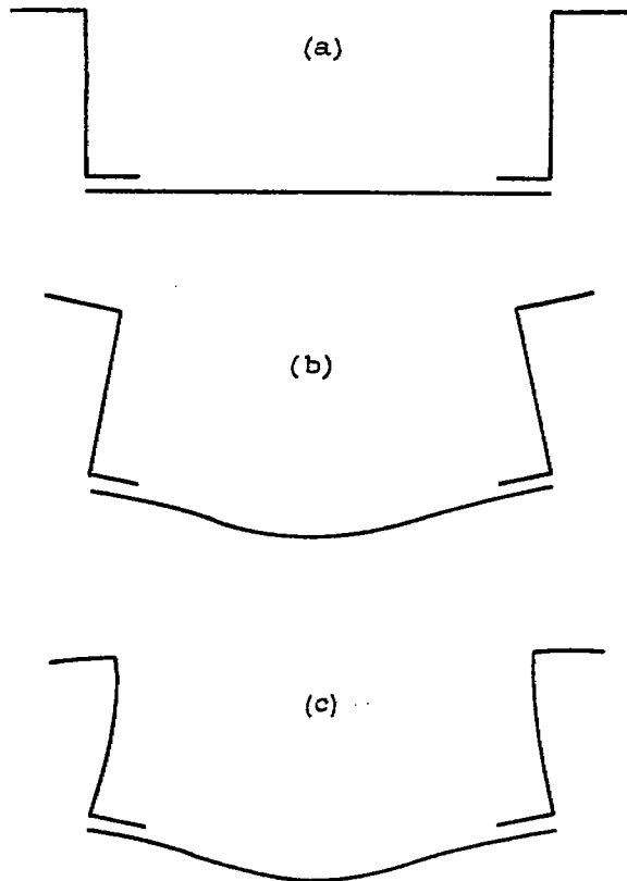
(a) Before buckling. (b) After buckling of plate when stiffeners are sturdy (no cross-sectional distortion of stiffeners). (c) After buckling of plate when stiffeners are frail (cross-sectional distortion of stiffeners).
