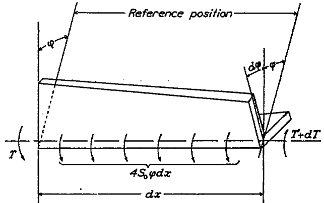
FIGURE 2.—Equilibrium of a sturdy-stiffener element dx .
