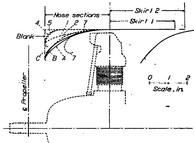
FIGURE 4.—Cowling profiles.
