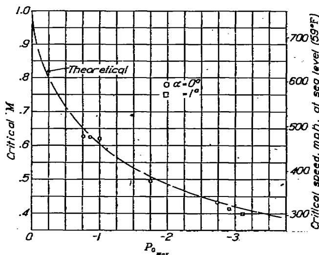
FIGURE 17.—Variation with peak pressure coefficient of critical speed.
