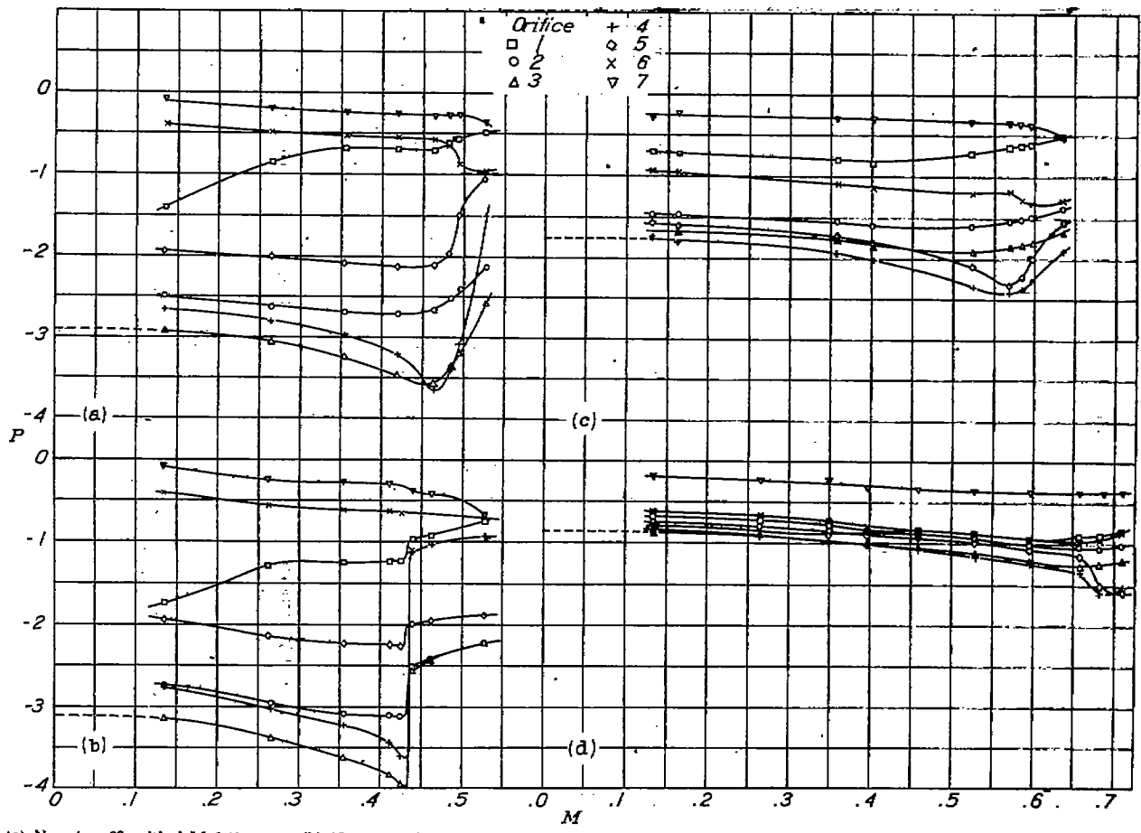
(a) Nose 4; \alpha = 0^\circ ; critical M, 0.41. (b) Nose 4; \alpha = 1^\circ ; critical M, 0.40. (c) Nose 7; \alpha = 0^\circ ; critical M, 0.40. (d) Nose B; \alpha = 0^\circ ; critical M, 0.02. FIGURE 11.—Variation with speed of pressures over top of cowlings.
