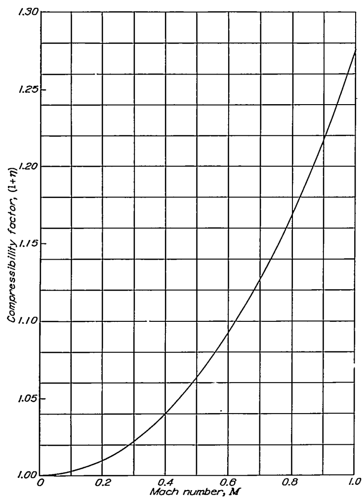
FIGURE 4.—Compressibility factor. (1+\eta) = 1 + \frac{M^2}{4} + \frac{M^4}{40} + \frac{M^6}{1600} + \dots
