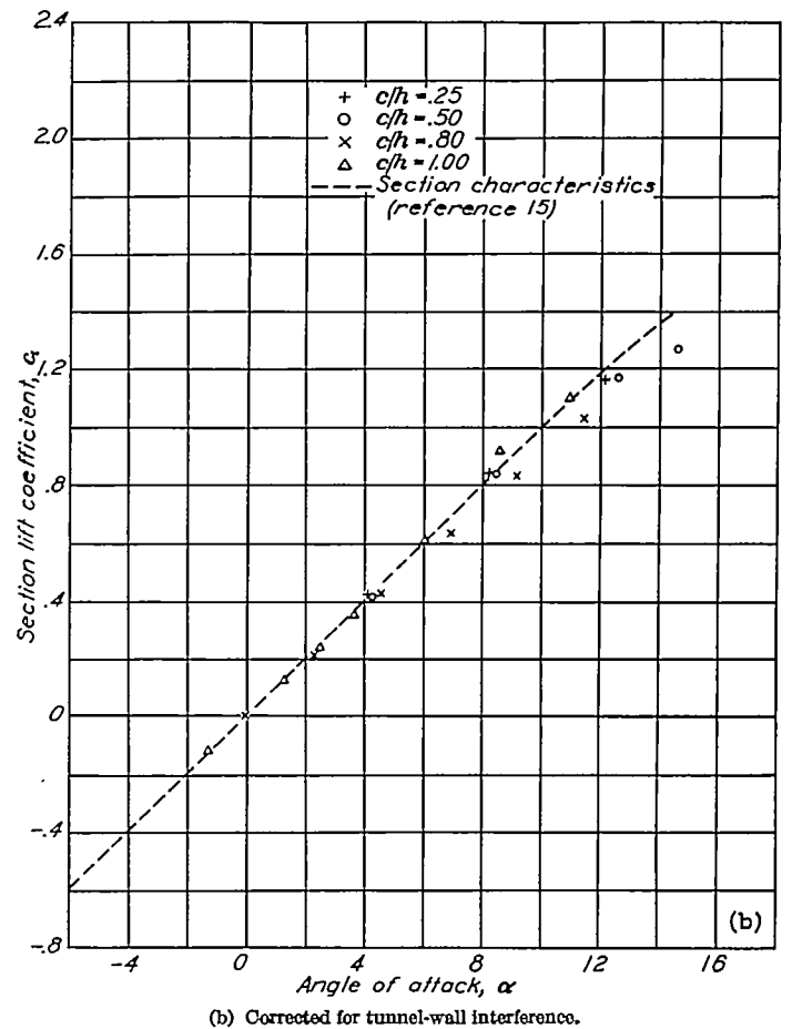
FIGURE 9.—Lift characteristics for NACA 0012 airfoil section.
