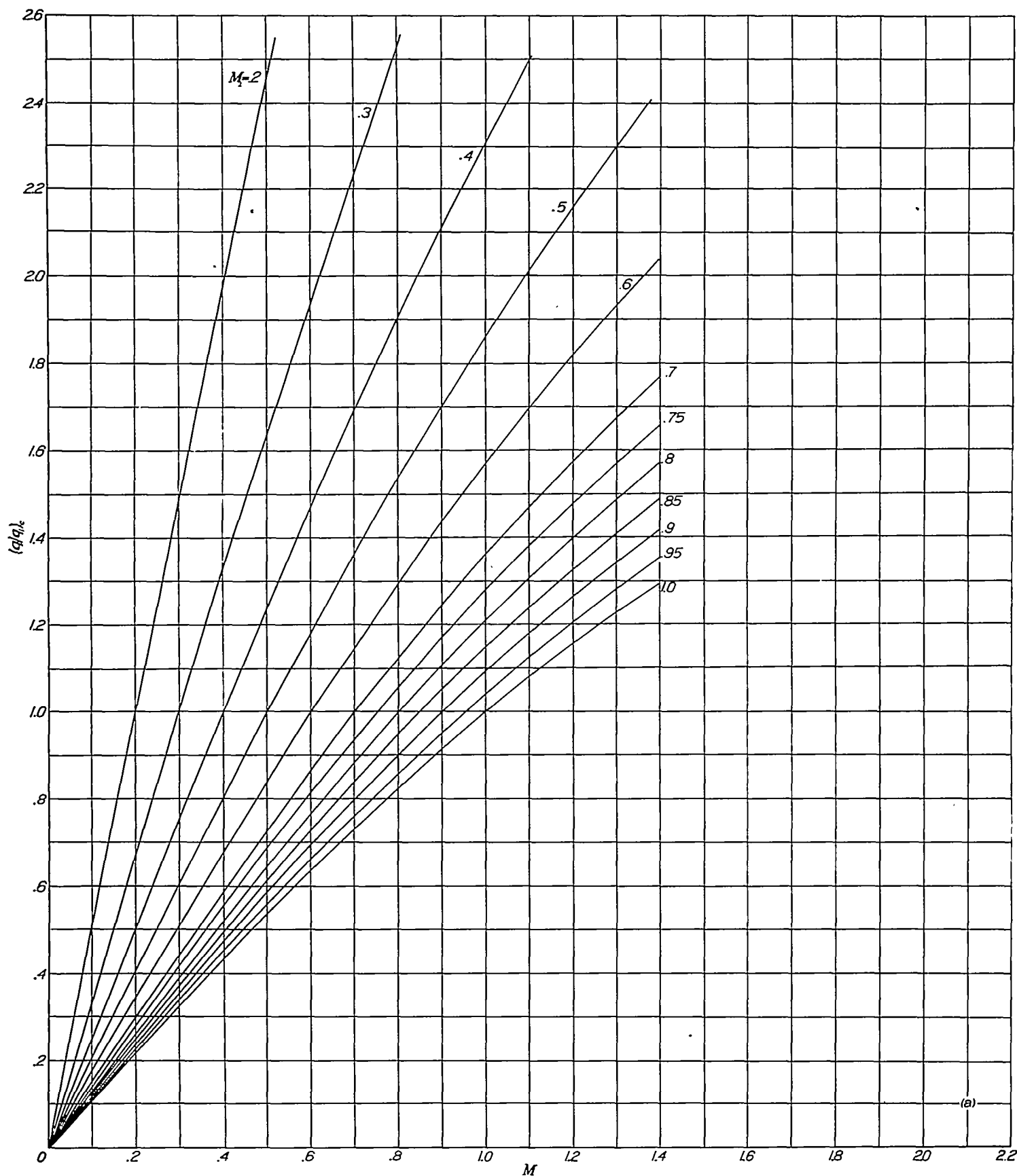
FIGURE 2.—Velocity ratios (q/q_1)_c , (q/q_1)_p , and (q/q_1)_c/(q/q_1)_p against local Mach number for various values of stream Mach number M_1 . Corresponding values of (q/q_1)_c and (q/q_1)_p in (a) and (b) are given by the same pair of values M, M_1 .
