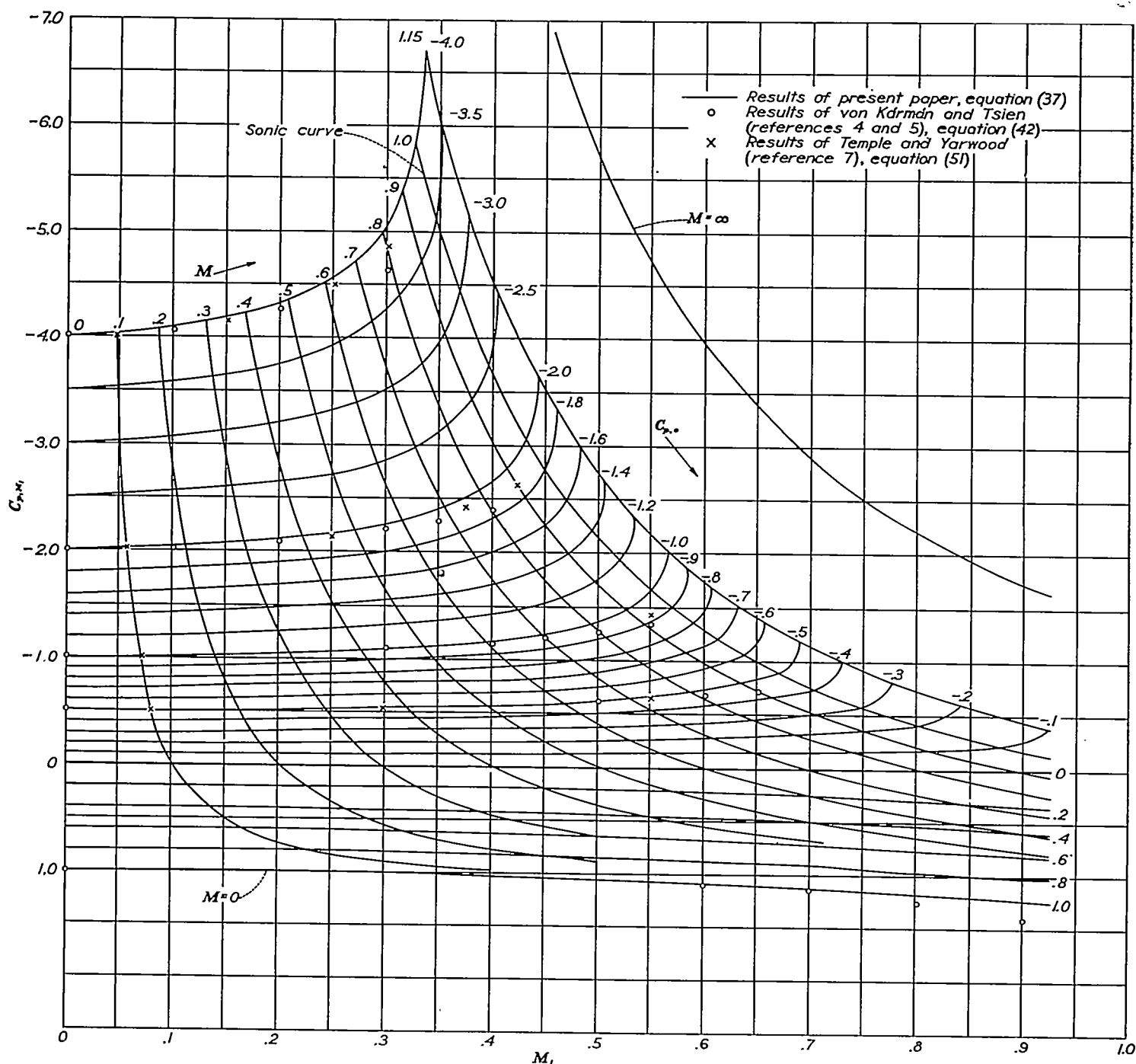
FIGURE 4.—Pressure coefficient C_{p, M_1} against stream Mach number M_1 with corresponding values of C_{p, \infty} and lines of constant local Mach number M .
