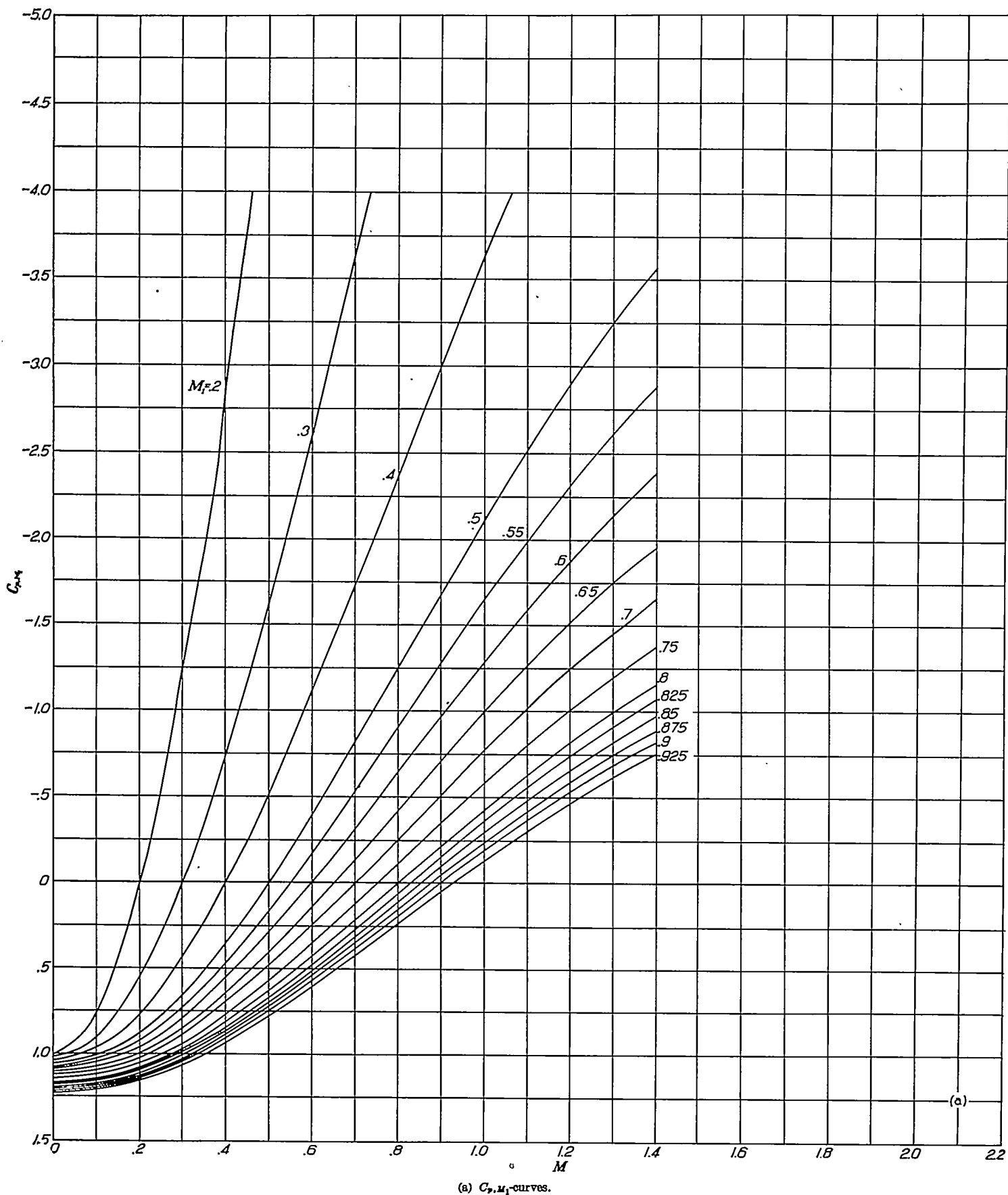
FIGURE 3.—Pressure coefficients C_{p, M_1} and C_{p, 0} against local Mach number M for various values of stream Mach number M_1 . Corresponding values of C_{p, M_1} and C_{p, 0} in (a) and (b) are given by the same pair of values M, M_1 .
