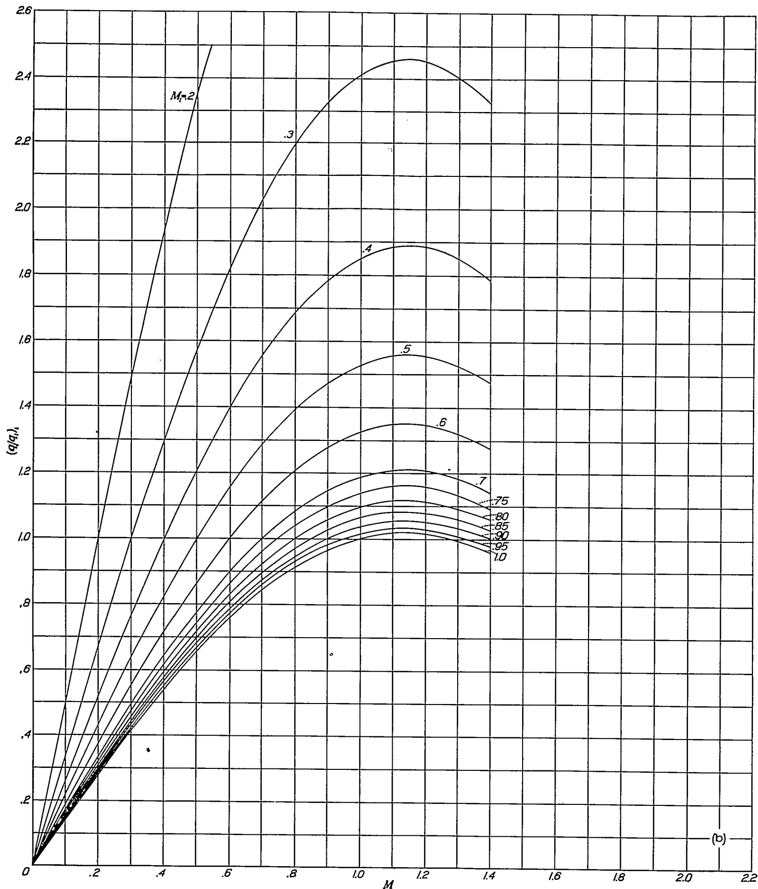
(b) (q/q_\infty)_0 , ratio of local velocity to stream velocity, incompressible.
