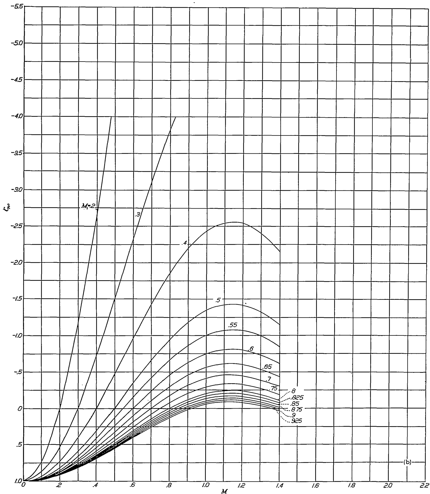
(b) C_{p,\delta} curves. FIGURE 3.—Concluded.
