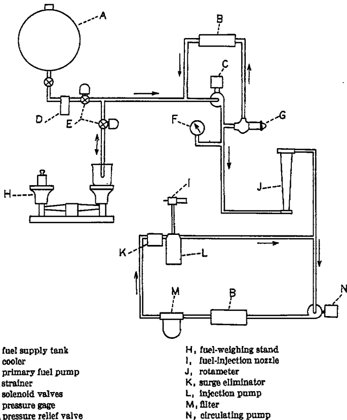
FIGURE 3.—Diagram of fuel system.
