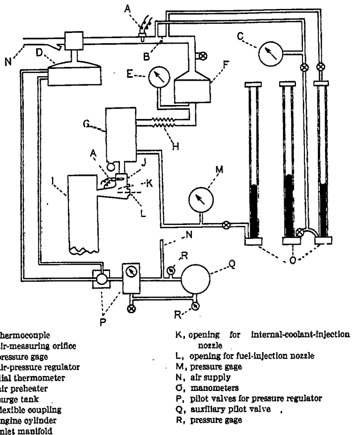
FIGURE 2.—Diagram of inlet-air system.
