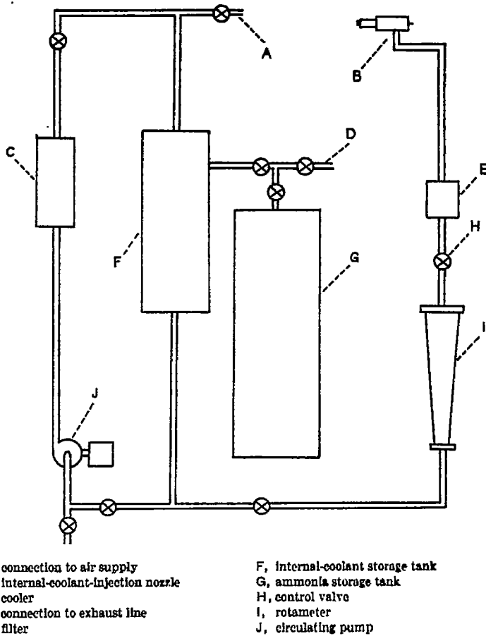
FIGURE 4.—Diagram of internal-coolant injection system.
