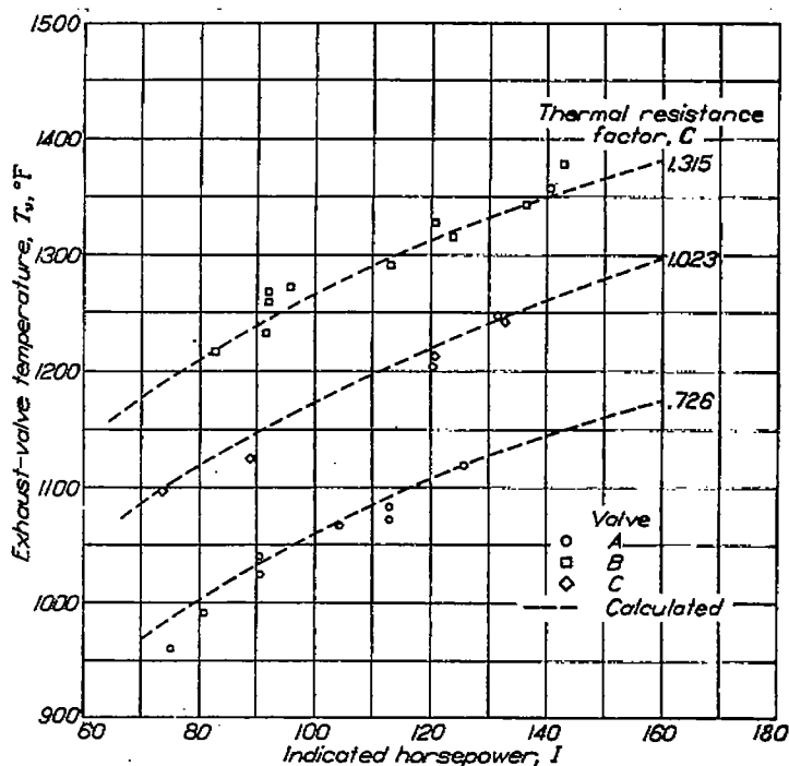
FIGURE 11.—Comparison of calculated and experimentally determined exhaust-valve temperatures in air-cooled cylinder. Engine speed, 2200 rpm; fuel-air ratio, 0.072; combustion-air temperature, 160° F; cooling-air pressure drop, 16 inches of water.
