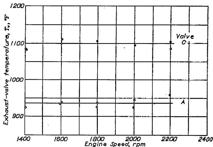
FIGURE 12.—Variation of exhaust-valve temperature with engine speed. Indicated horsepower, 71.5; fuel-air ratio, 0.072; combustion-air temperature, 150° F; cooling-air pressure drop, 16 inches of water.
