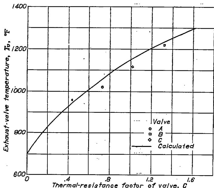
FIGURE 10.—Effect of thermal-resistance factor on exhaust-valve temperature. Engine speed, 2300 rpm; indicated horsepower, 128; fuel-air ratio, 0.09; combustion-air temperature, 160° F; rear-spark-plug-bushing temperature, 426° F.
