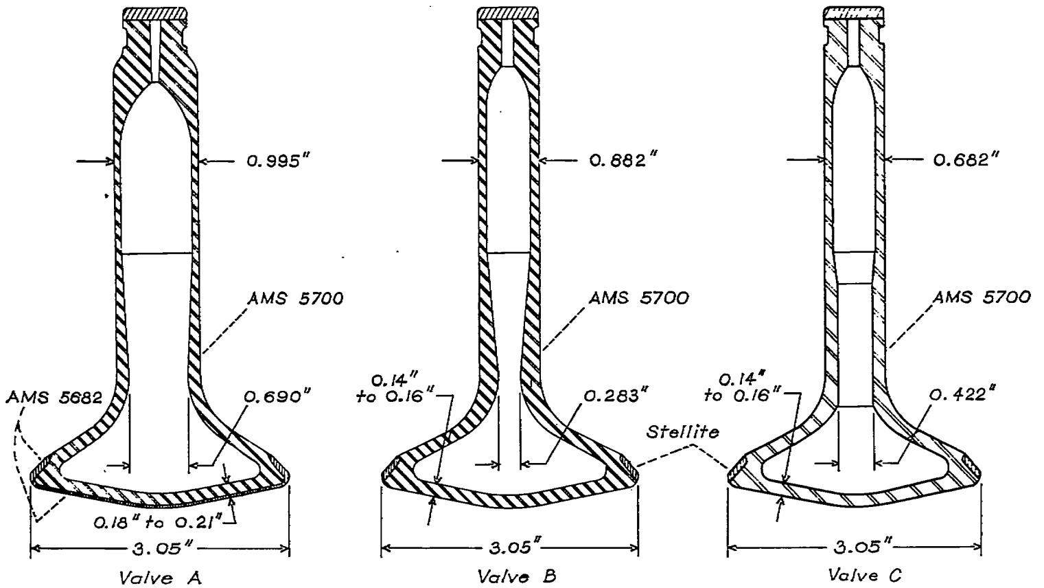
FIGURE 3.—Comparison of valve-design features.
