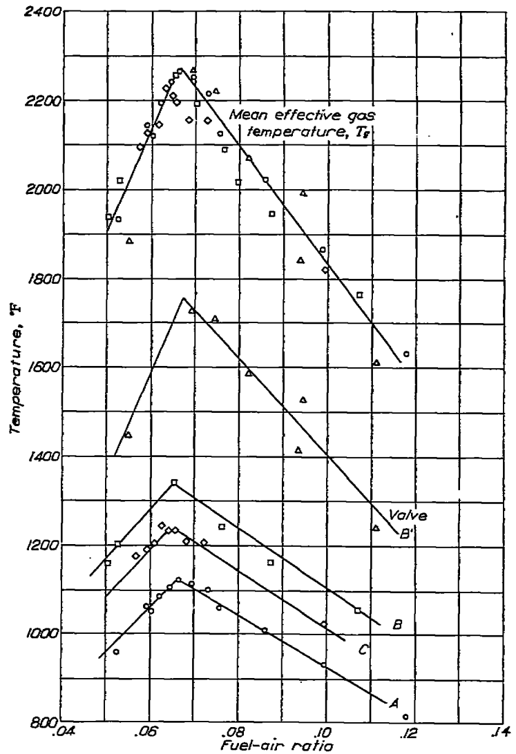
FIGURE 8.—Variation of mean effective gas temperature and valve temperature with fuel-air ratio. Engine speed, 2200 rpm; indicated horsepower, 117; combustion-air temperature, 116° F; cooling-air pressure drop, 16 inches of water; spark timing, 22½° B. T. C.
