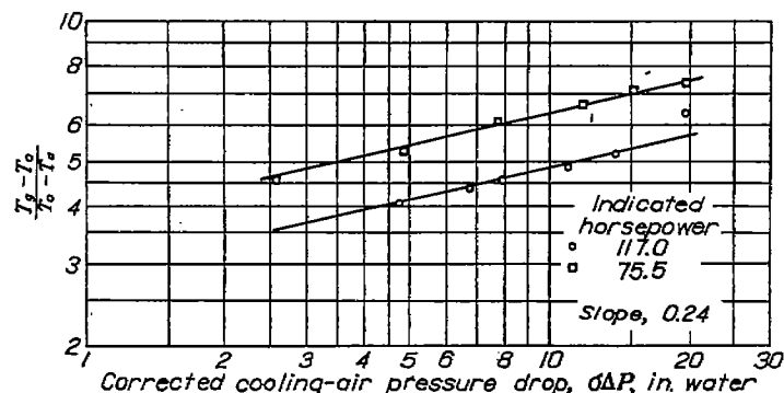
FIGURE 6.—Variation in \frac{T_g - T_o}{T_g - T_a} with cooling-air pressure drop across cylinder. Valve A; engine speed, 2200 rpm; fuel-air ratio, 0.072; combustion-air temperature, 150° F; spark timing, 22½° B. T. C.
