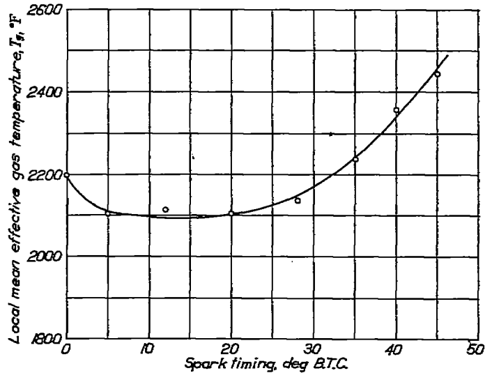
FIGURE 9.—Effect of spark timing on local mean effective gas temperature. Engine speed, 2200 rpm; indicated horsepower, 97; fuel-air ratio, 0.06; cooling-air pressure drop, 16 inches of water; combustion-air temperature, 150° F. (Data from reference 2, fig. 9.)
