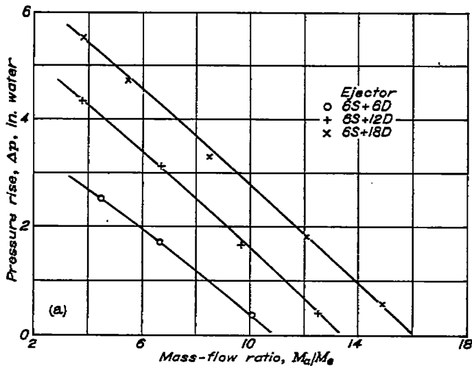
FIGURE 10.—Optimum combination of straight and diffuser sections for 24-inch over-all-length ejector. Area, 25 square inches; aspect ratio, 3; exhaust-gas mass-flow rate, 8 pounds per minute; exhaust-nozzle area, 2.6 square inches; fuel-air ratio, 0.08; indicated horsepower, 85. For further details see table I.
