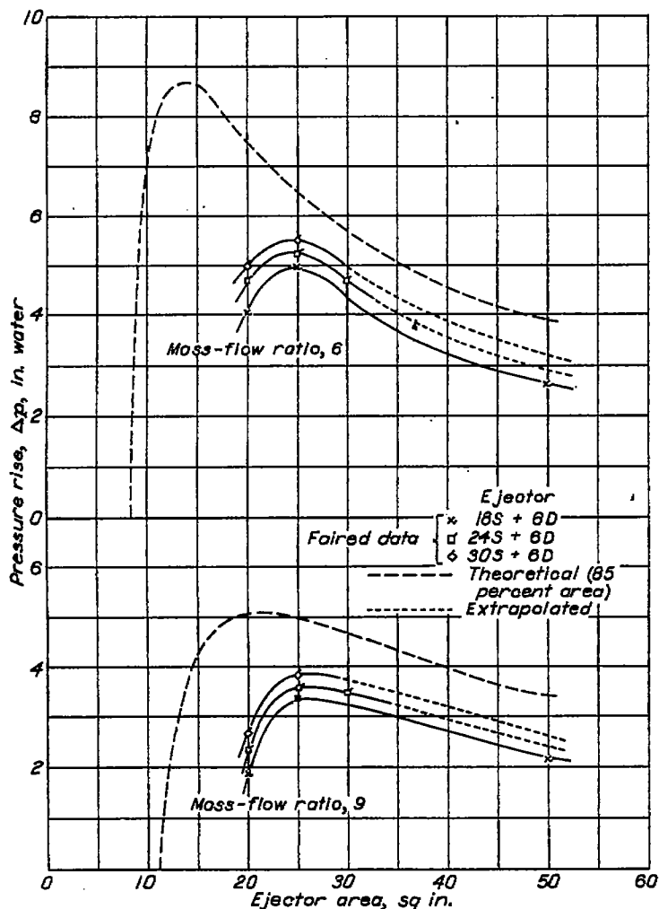
FIGURE 11.—Variation of pressure rise with ejector area for 6-inch diffuser ejectors actuated by exhaust of single-cylinder engine. Aspect ratio, 3; exhaust-gas mass-flow rate, 8 pounds per minute; exhaust-nozzle area, 2.6 square inches; fuel-air ratio, 0.08; indicated horsepower, 85.
