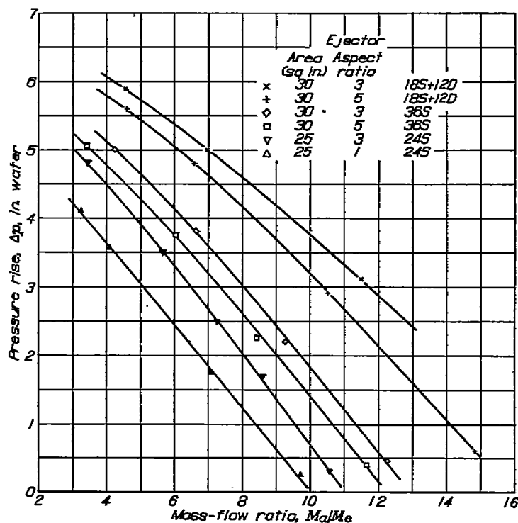
FIGURE 15.—Effect of mixing-section aspect ratio on performance of ejectors actuated by exhaust of single-cylinder engine. Exhaust-gas mass-flow rate, 8 pounds per minute; exhaust-nozzle area, 2.6 square inches; fuel-air ratio, 0.08; indicated horsepower, 85. For further details see table I.
