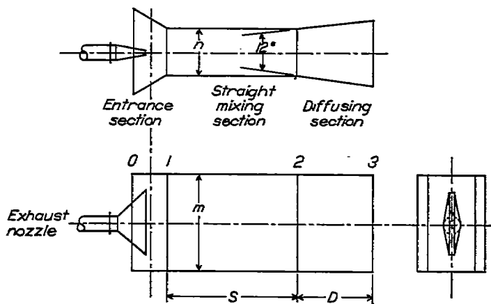
FIGURE 3.—Ejector details and terminology. Straight mixing-section area, square inches; aspect ratio of straight mixing section m/n ; length of straight mixing section S, inches; length of diffusing section D, inches. (For example, an ejector with a straight section of 24 in. and a diffusing section of 12 in. would be designated 24S+12D.)
