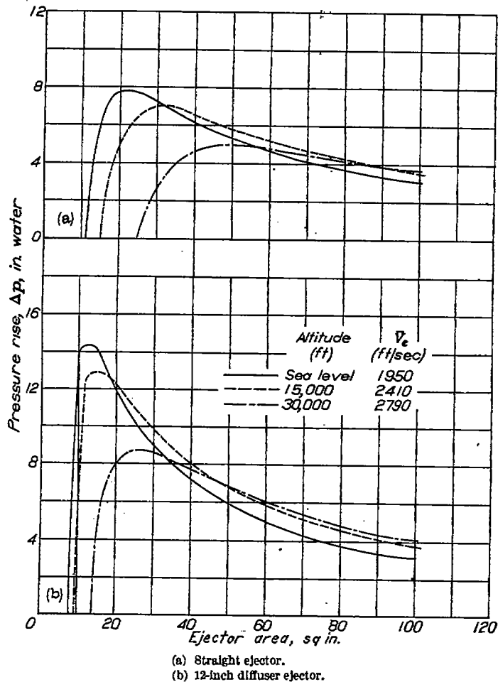
FIGURE 20.—Theoretical variation of pressure rise with ejector area at various altitudes. Mass-flow ratio, 6; exhaust-gas mass-flow rate, 12 pounds per minute; exhaust-gas temperature, 1500° F; air temperature, 75° F; exhaust-nozzle area, 2.6 square inches.
