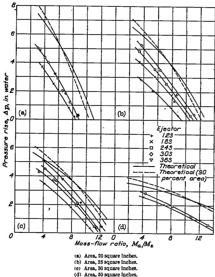
FIGURE 4.—Performance curves for straight ejectors actuated by exhaust of single-cylinder engine. Aspect ratio, 3; exhaust-gas mass-flow rate, 8 pounds per minute; exhaust-nozzle area, 2.6 square inches; fuel-air ratio, 0.08; indicated horsepower, 85. For further details see table I.
