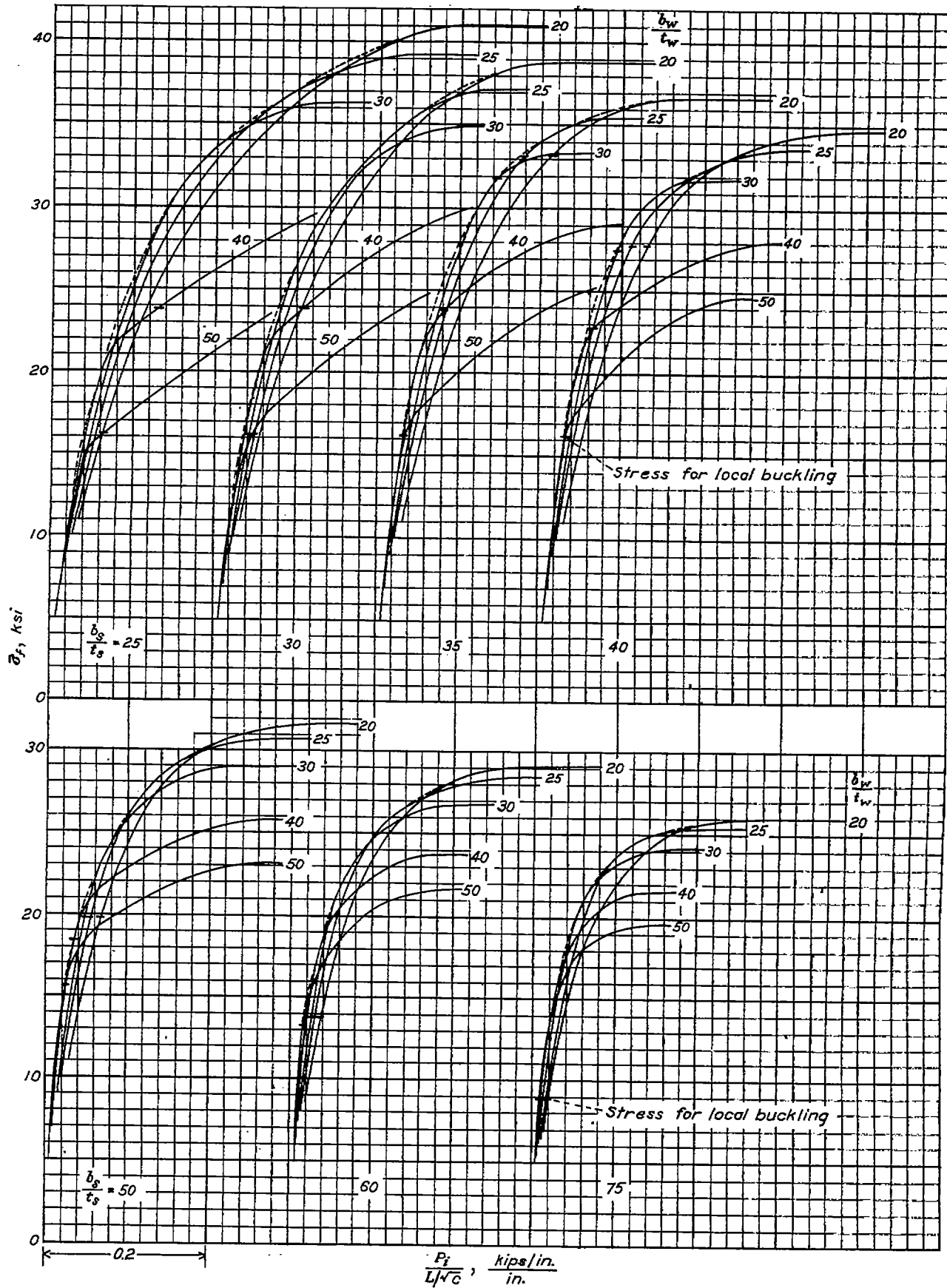
FIGURE 5.—Design chart for 24S-T aluminum-alloy flat panels with Z-section stiffeners; t_w/t_s = 1.00 ( b_s/t_s = 8.0 ; t_s/t_w = 3 ; t_w/t_s = 4 ; and b_w/t_w = 0.3 to 0.5 ).
