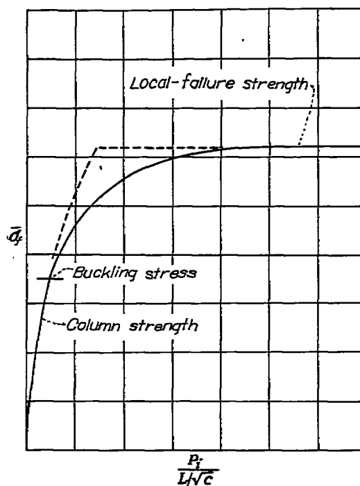
FIGURE 14.—Typical design curve for panels that buckle.
