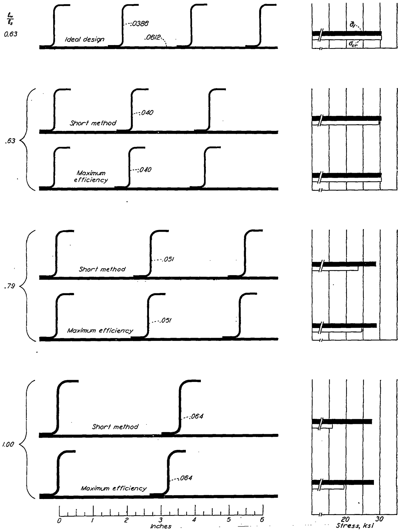
FIGURE 8.—Designs of 249-T aluminum-alloy panels 20 inches long with P_r = 3.0 kips per inch, c = 1 , and t_s = 0.064 inch.
