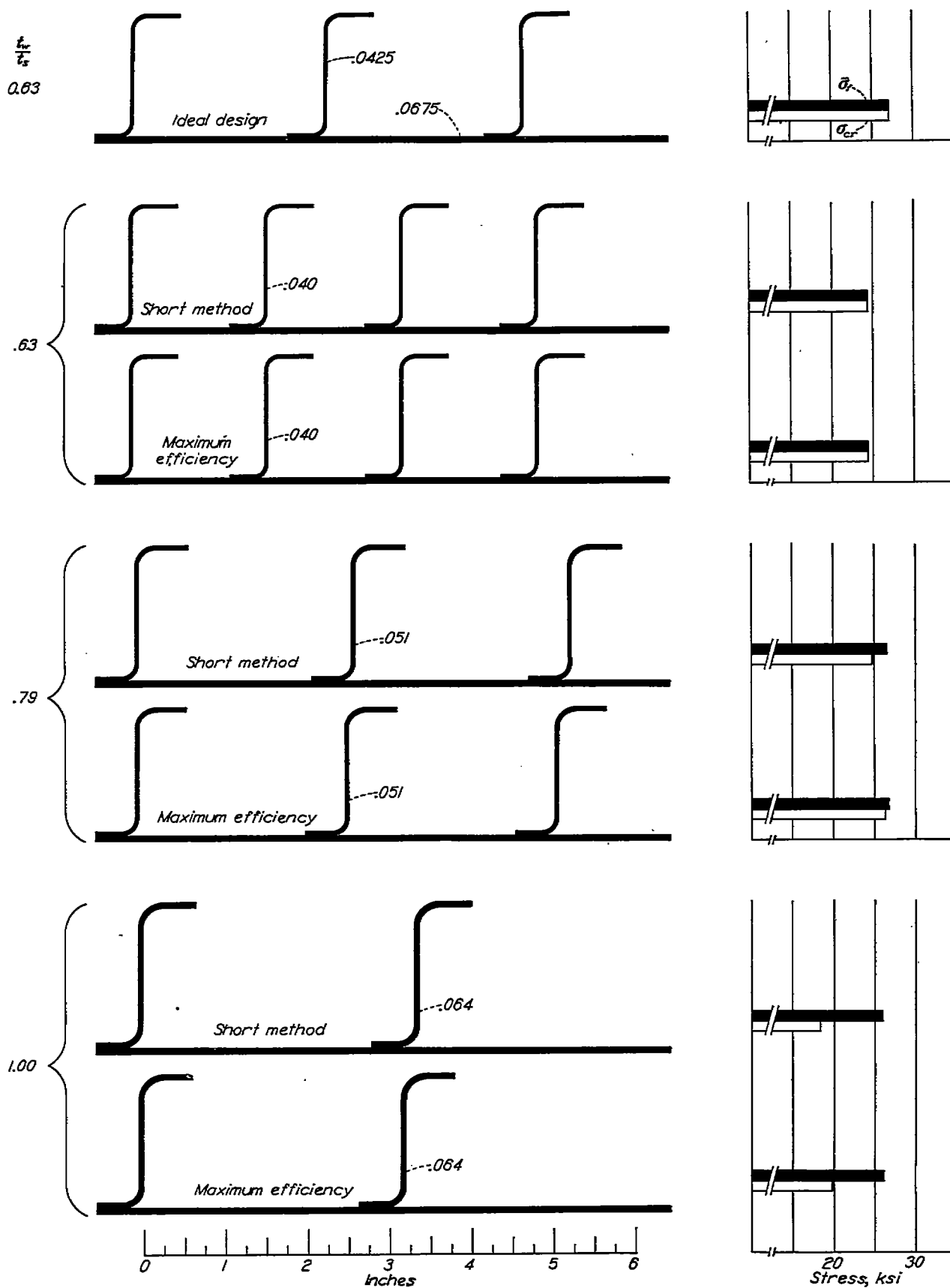
FIGURE 9.—Designs of 24S-T aluminum-alloy panels 30 inches long with P_c=3.0 kips per inch, c=1 , and s=0.064 inch.
