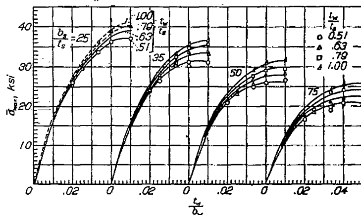
FIGURE 12.—Average stress at local failure for 24S-T aluminum-alloy flat compression panels with longitudinal Z-section stiffeners. b_r/b_w = 0.4 .
