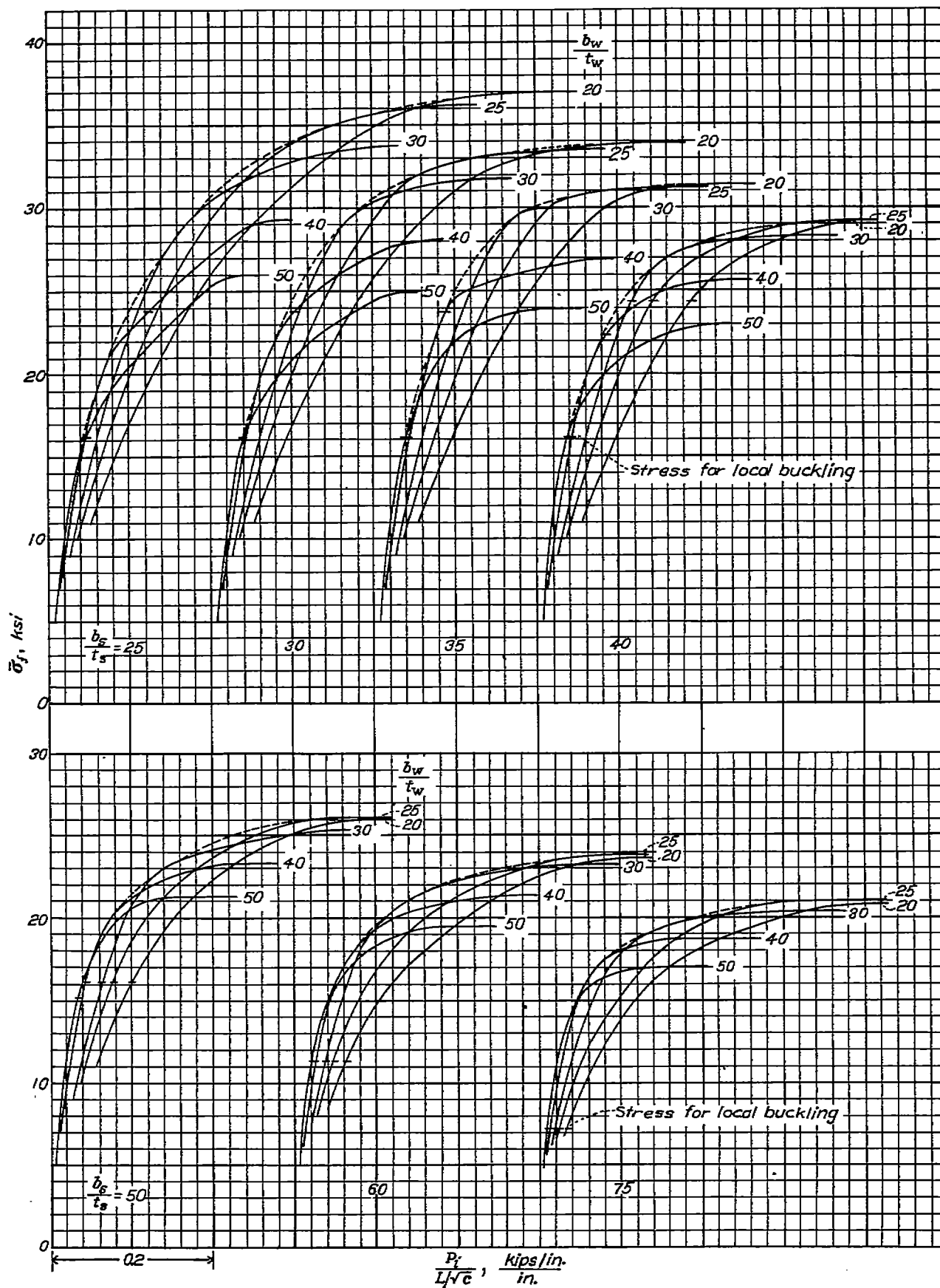
FIGURE 2.—Design chart for 24S-T aluminum-alloy flat panels with Z-section stiffeners; t_w/t_s = 0.51 ( b_s/t_s = 11.4 ; r_A/t_w = 3 ; r_F/t_w = 4 ; and b_F/b_w = 0.3 to 0.5 ).
