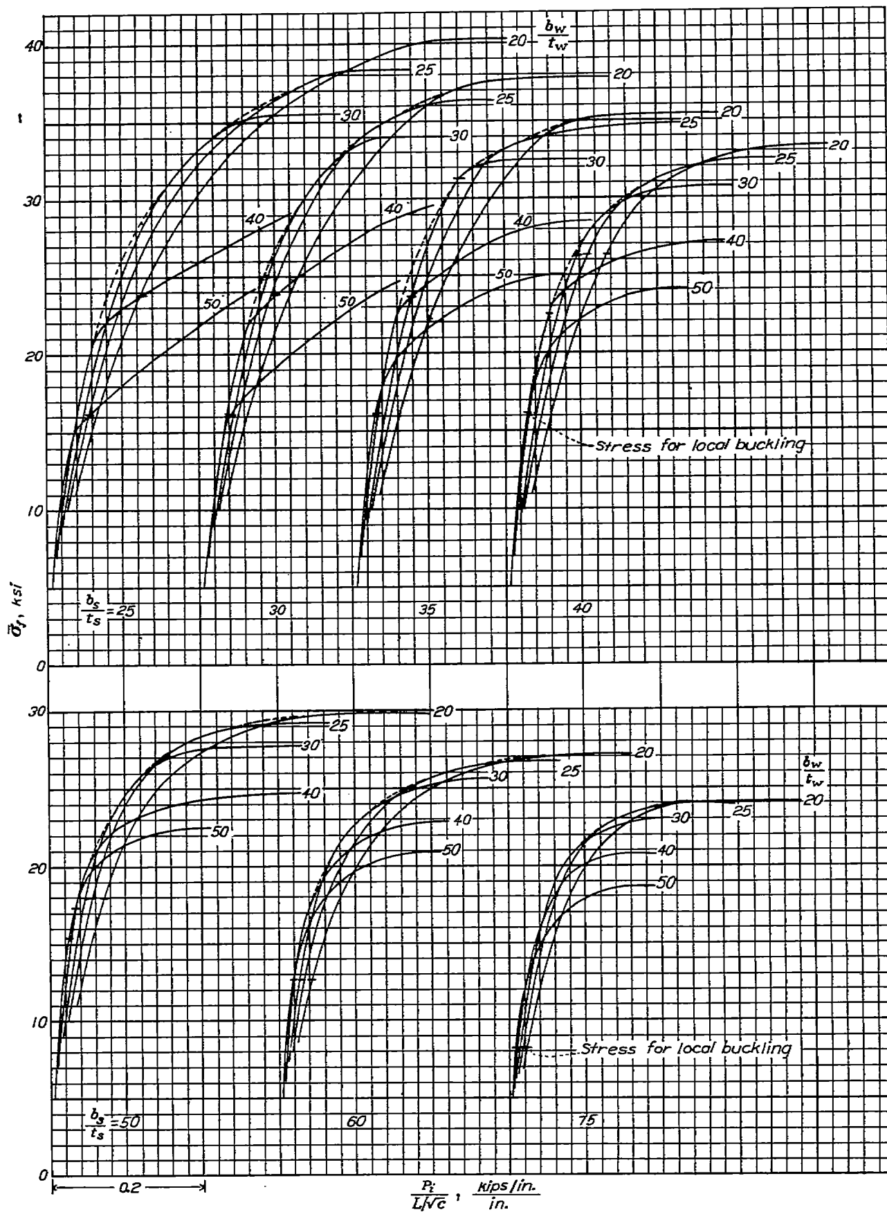
FIGURE 4.—Design chart for 24S-T aluminum-alloy flat panels with Z-section stiffeners; \frac{t_w}{t_s} = 0.70 ( \frac{b_s}{t_s} = 9.5 ; \frac{r_s}{t_s} = 3 ; \frac{r_w}{t_w} = 4 ; and \frac{b_w}{t_w} = 0.3 to 0.5 ).
