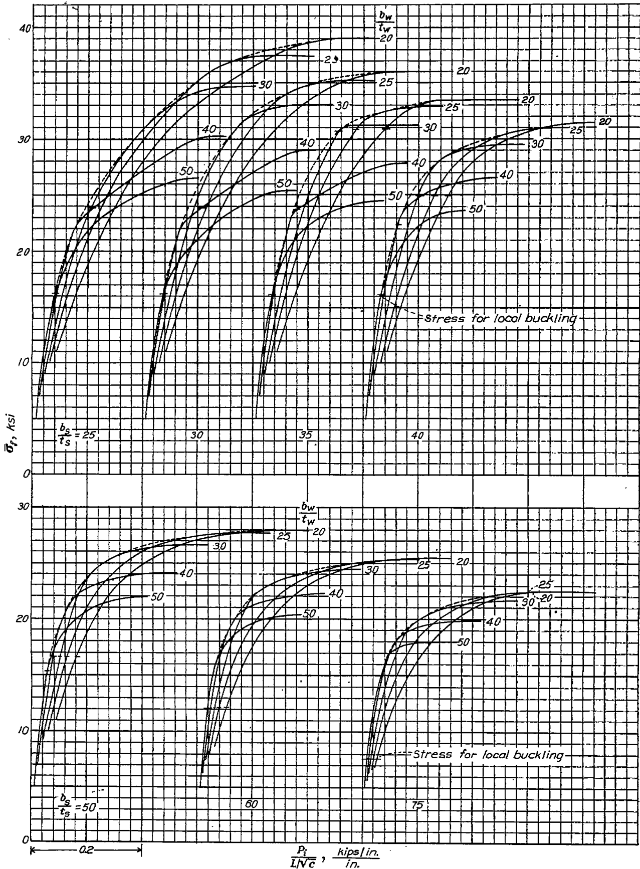
FIGURE 3.—Design chart for 24S-T aluminum-alloy flat panels with Z-section stiffeners; t_w/t_s = 0.63 ( b_s/t_s = 10.9 ; t_s/t_w = 3 ; r_x/r_y = 4 ; and b_w/t_w = 0.3 to 0.5 ).
