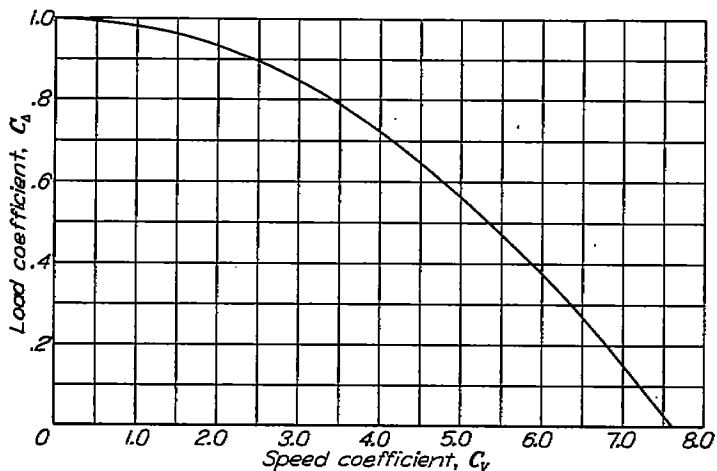
FIGURE 4.—Load curve based on constant lift coefficient.
