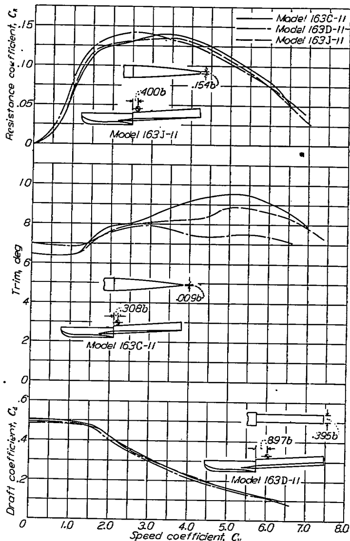
FIGURE 13.—Effect on free-to-trim characteristics of tapering afterbody.
