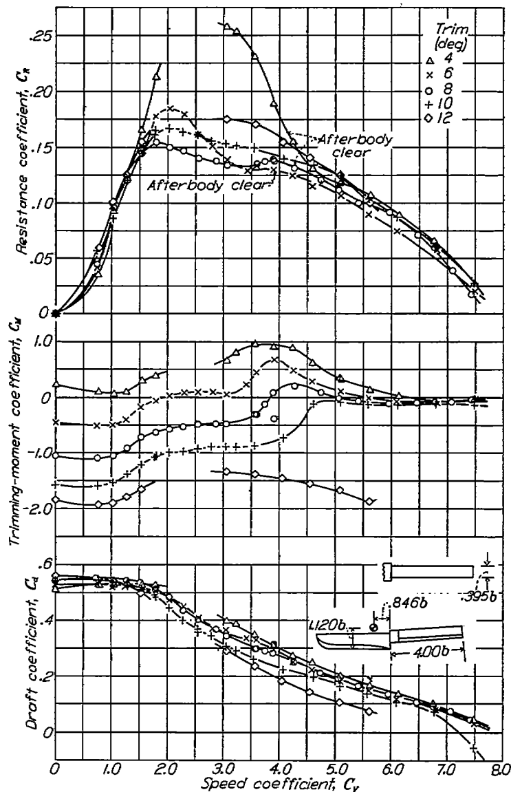
FIGURE 5.—Resistance, trimming-moment, and draft characteristics of model 163A-11 at fixed trim.
