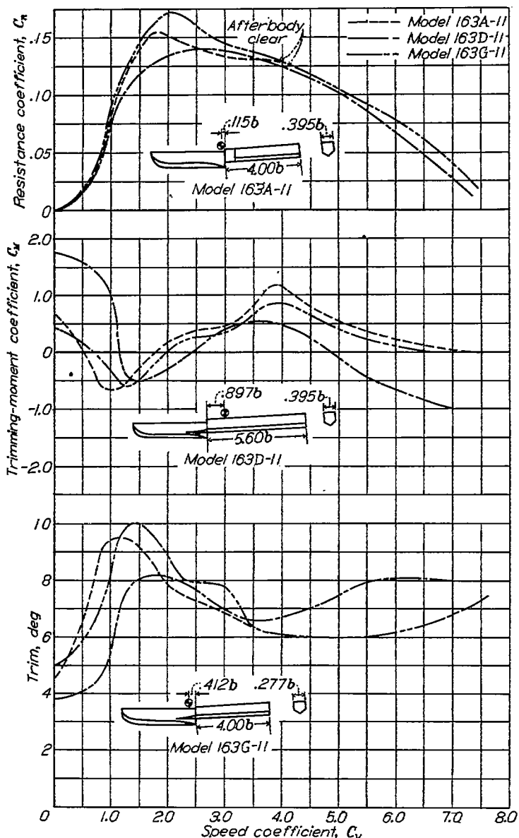
FIGURE 10.—Effect on best-trim characteristics of varying length and width of afterbody.
