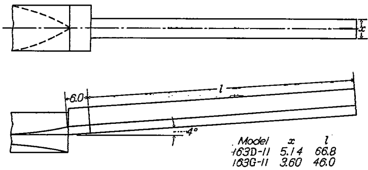
FIGURE 2.—Lines of rectangular afterbody. (All dimensions are in inches.)
