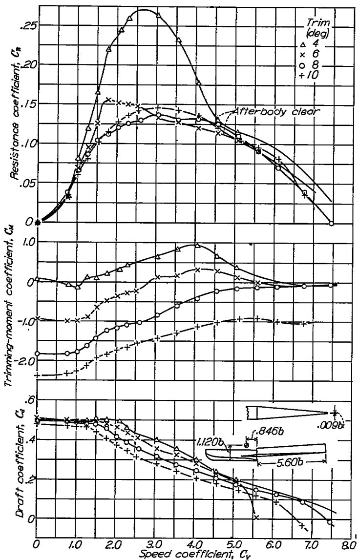
FIGURE 8.—Resistance, trimming-moment, and draft characteristics of model 163C-11 at fixed trim.
