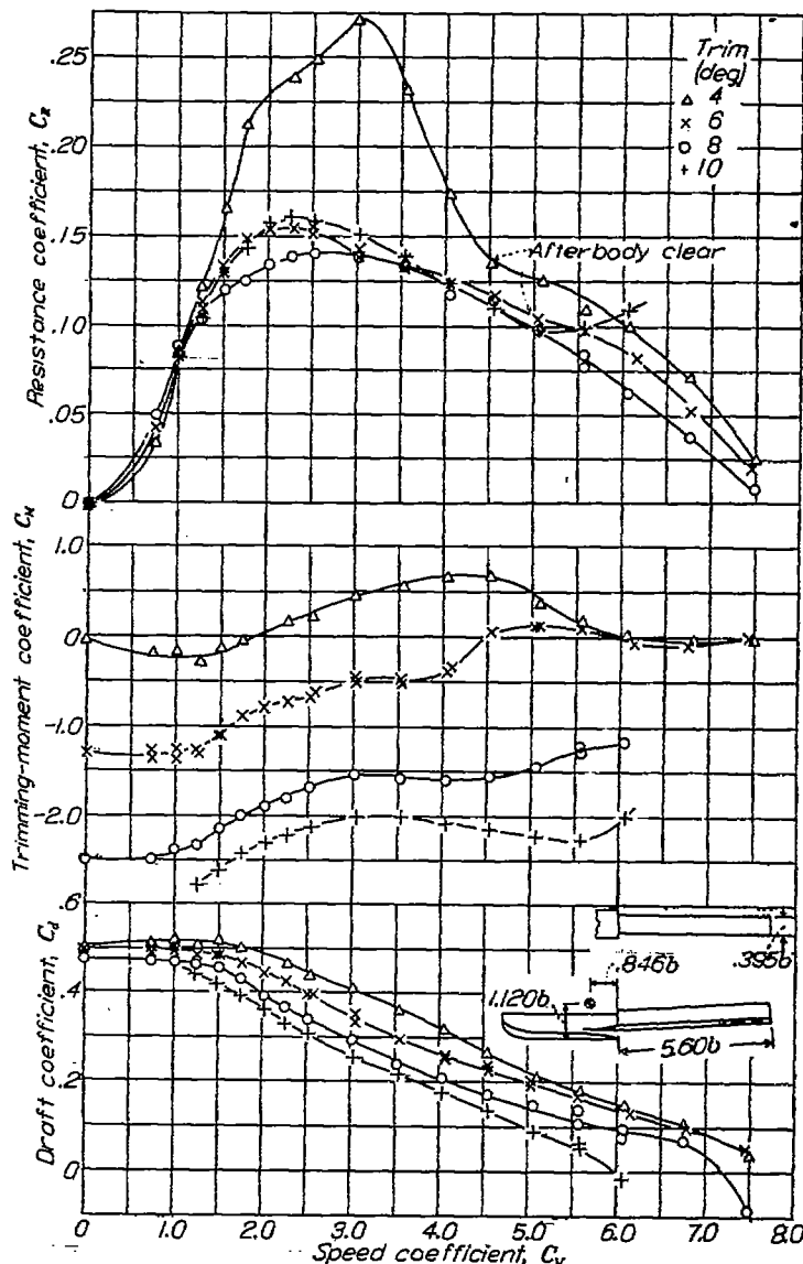
FIGURE 7.—Resistance, trimming-moment, and draft characteristics of model 163D-11 at fixed trim.
