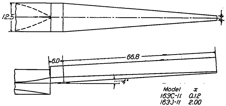
FIGURE 3.—Lines of tapered afterbody. (All dimensions are in inches.)
