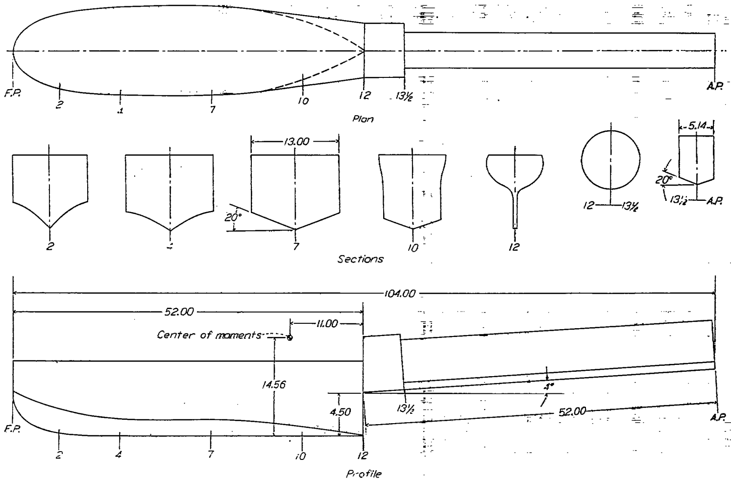
FIGURE 1.—Lines of Langley tank model 163A-11. (All dimensions are in inches.)
