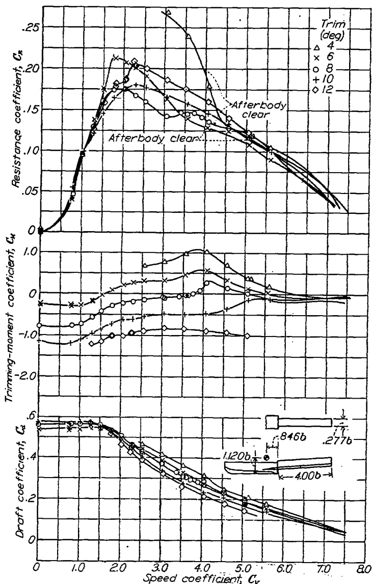
FIGURE 6.—Resistance, trimming-moment, and draft characteristics of model 163G-11 at fixed trim.
