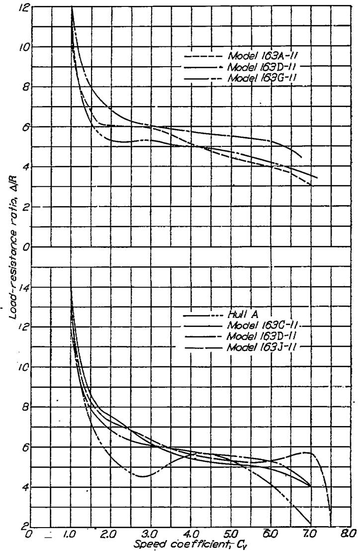
FIGURE 15.—Comparison of load-resistance ratios of planing-tail hulls and a conventional hull.
