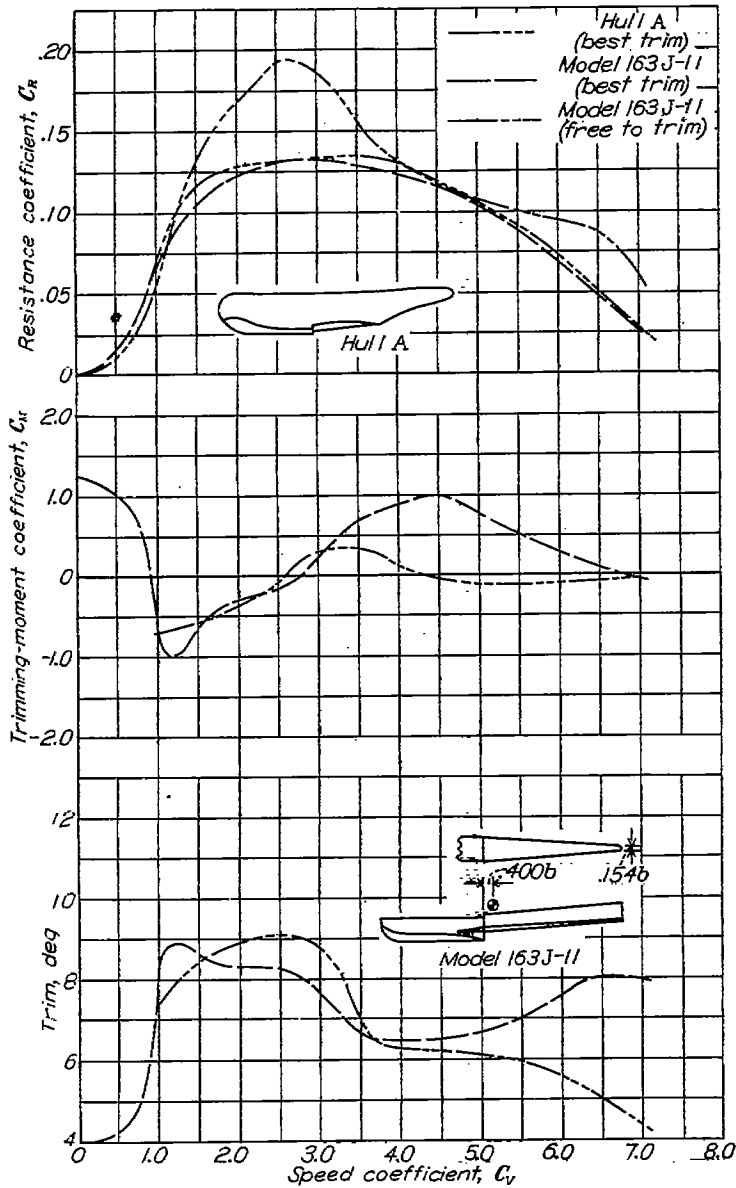
FIGURE 14.—Comparison of the resistance characteristics of a planing-tail hull with those of a conventional hull.
