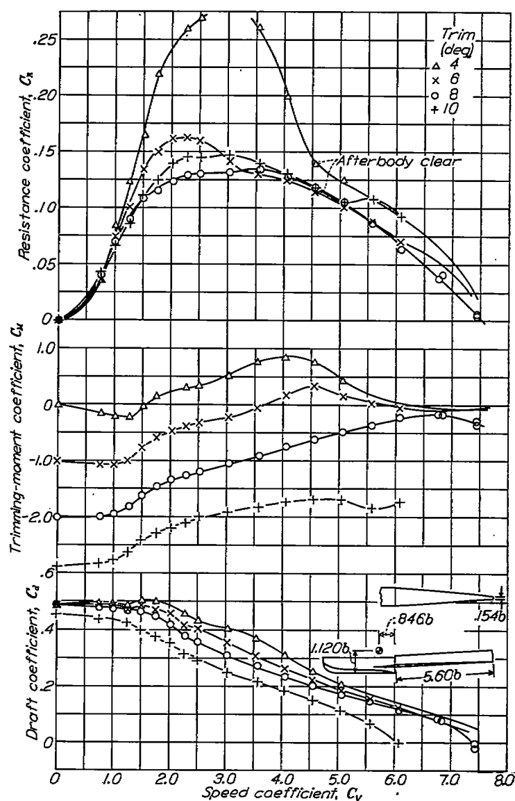
FIGURE 9.—Resistance, trimming-moment, and draft characteristics of model 163J-11 at fixed trim.
