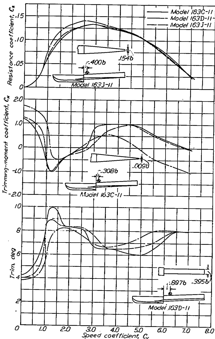
FIGURE 12.—Effect on best-trim characteristics of tapering afterbody.
