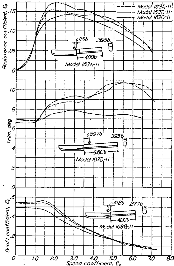
FIGURE 11.—Effect on free-to-trim characteristics of varying length and width of afterbody.
