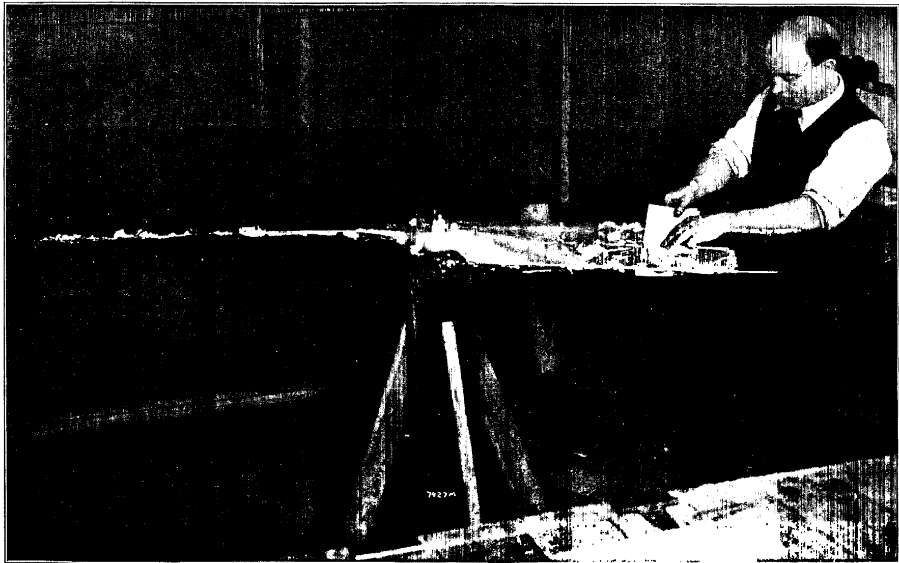
PLATE I.—METHOD OF APPLYING ALUMINUM LEAF TO PROPELLER.
