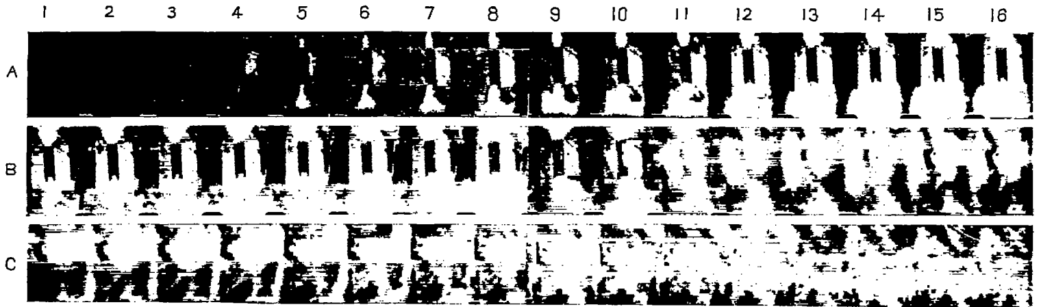
FIGURE 21.—Shot of exploding firecracker showing simultaneous rupture of side wall at two points, taken at 40,000 frames per second with the NACA high-speed motion-picture camera.
