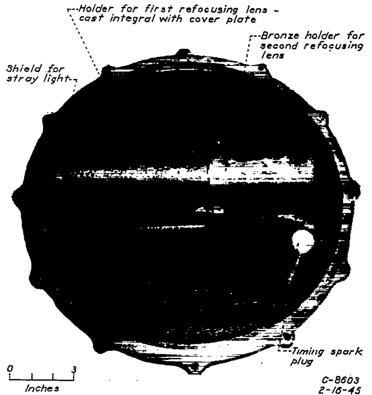
FIGURE 16.—Inner side of camera cover plate and lens holder.
