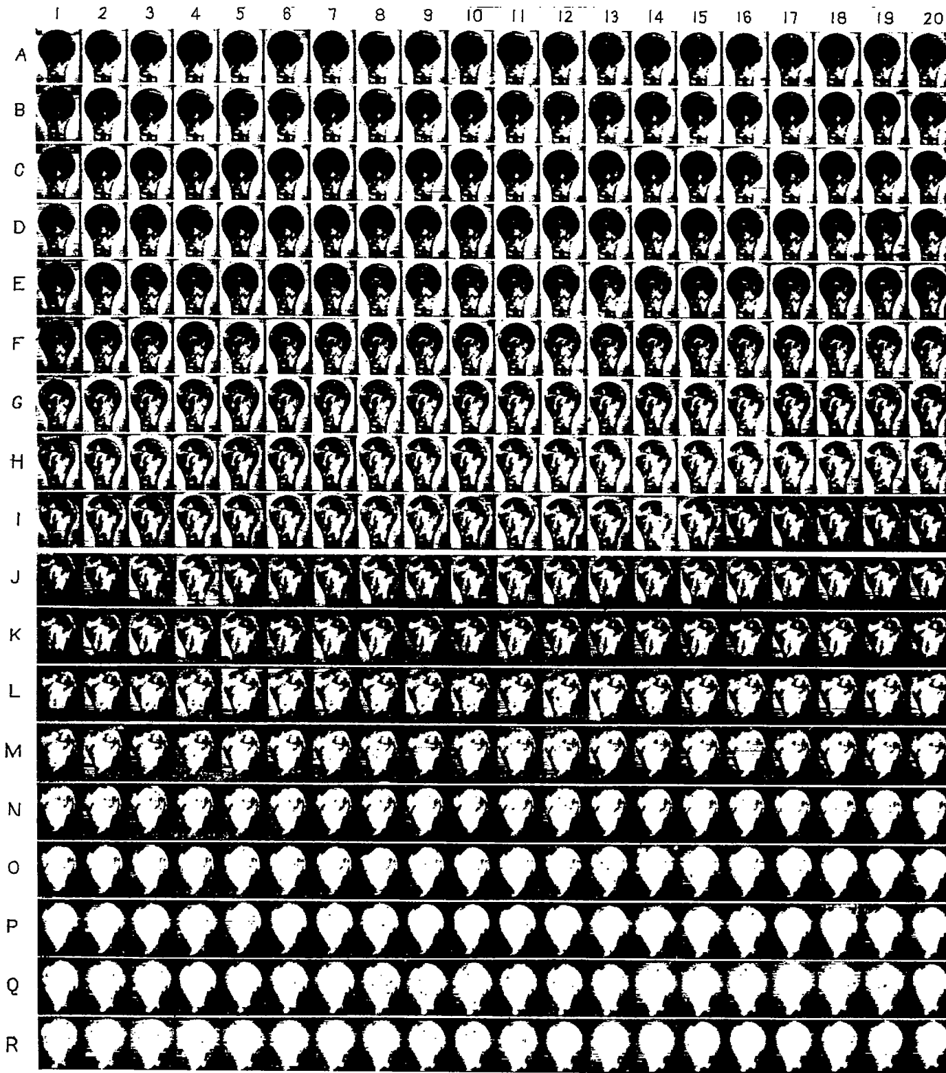
FIGURE 20.—Shot of combustion of an ordinary photoflash bulb taken at 40,000 frames per second with the NACA high-speed motion-picture camera.
