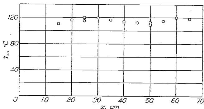
FIGURE 6.—Temperature distribution along heated plate.
