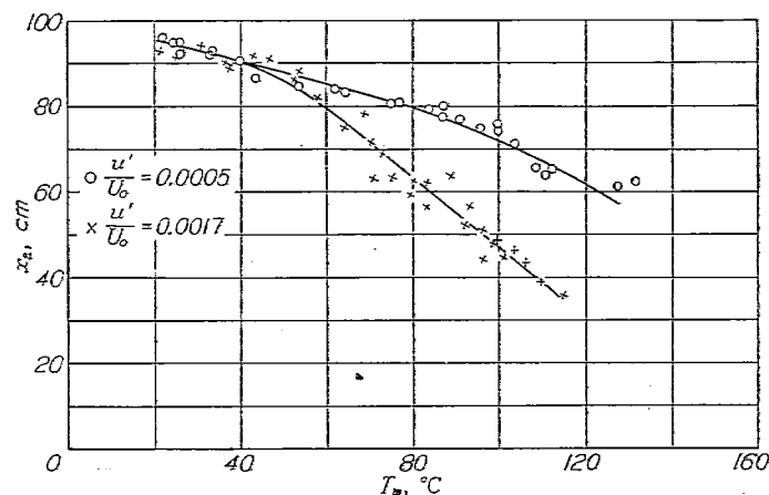
FIGURE 14.—Effect of plate temperature on transition.
