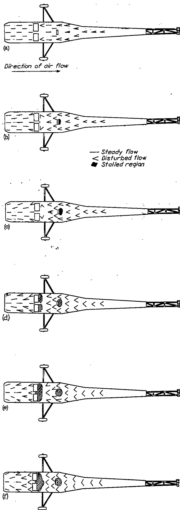
FIGURE 6.—Tuft observations on underside of helicopter fuselage. Tunnel airspeed, 62 miles per hour.
