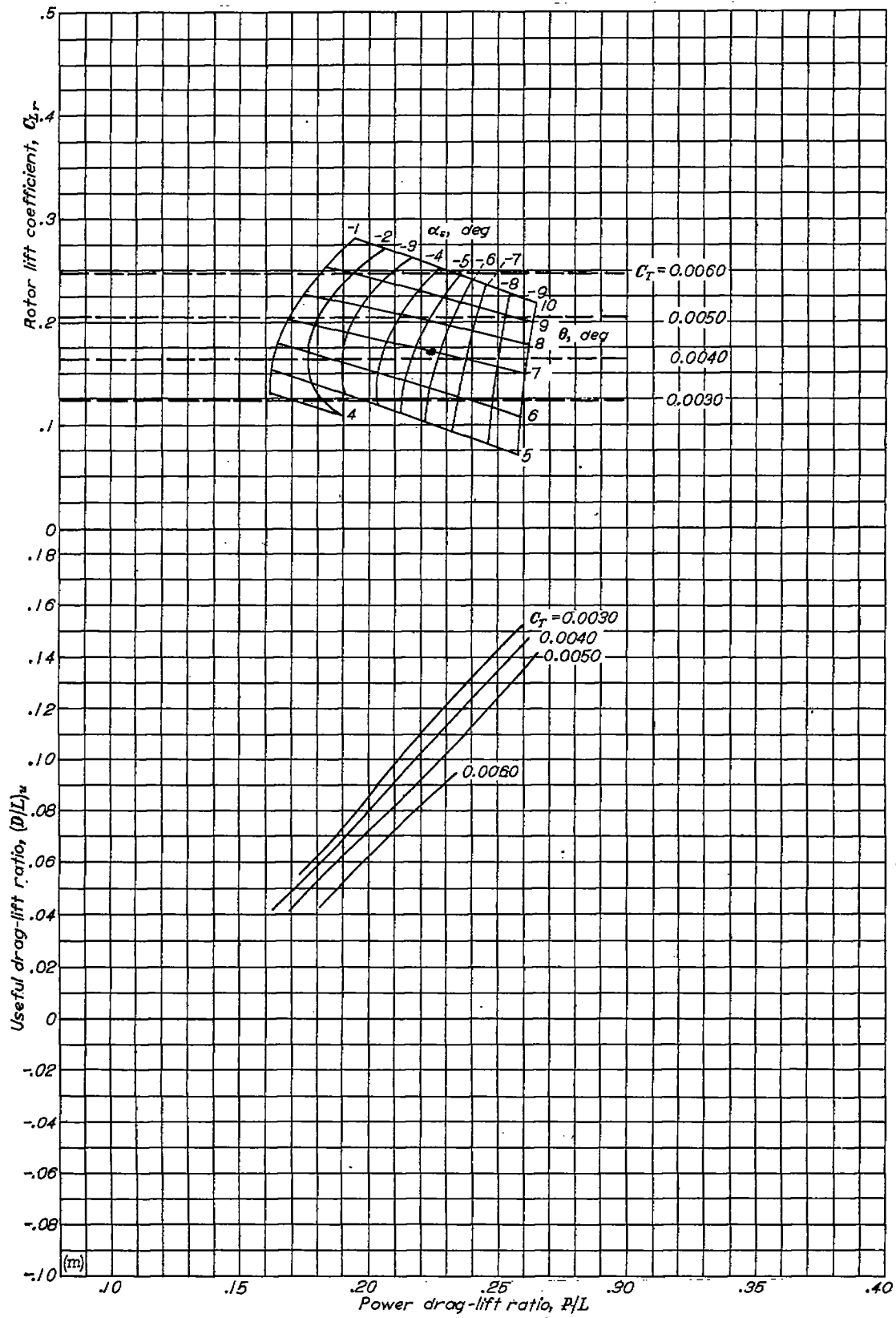
(m) \mu=0.22 , FIGURE 11.—Continued.
