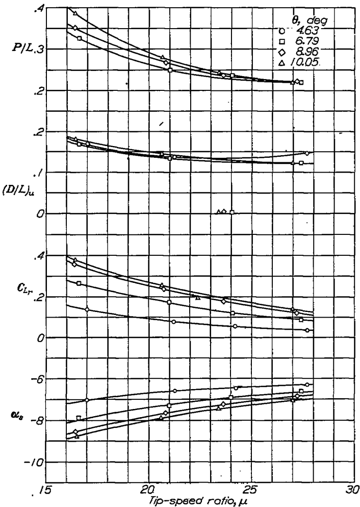
FIGURE 8.—Initial plot of main-rotor parameters. \alpha_T = -5.6^\circ .
