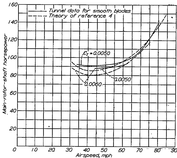
FIGURE 15.—A comparison of the experimentally determined forward-flight performance of the helicopter with that determined from theory. Gross weight, 2560 pounds; \frac{\rho}{\rho_0}=0.924 .
