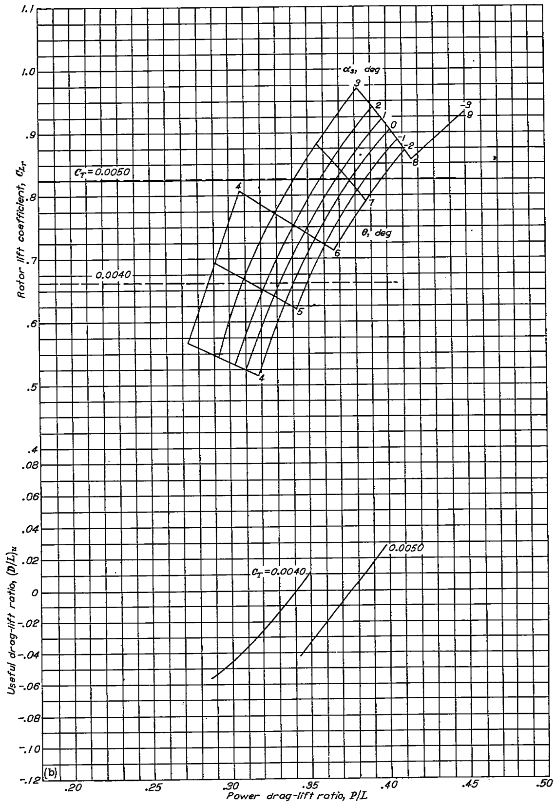
(b) \mu = 0.11 . FIGURE 11.—Continued.
