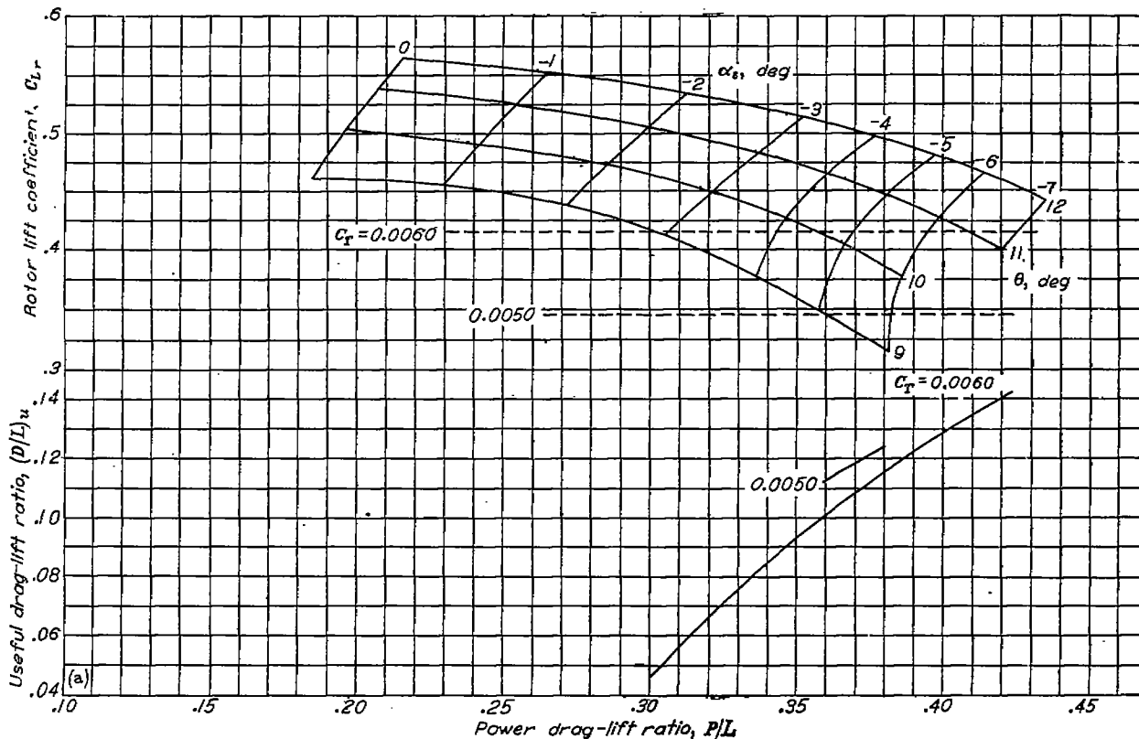
(a) \mu=0.17 . FIGURE 12.—Aerodynamic characteristics of the production rotor.
