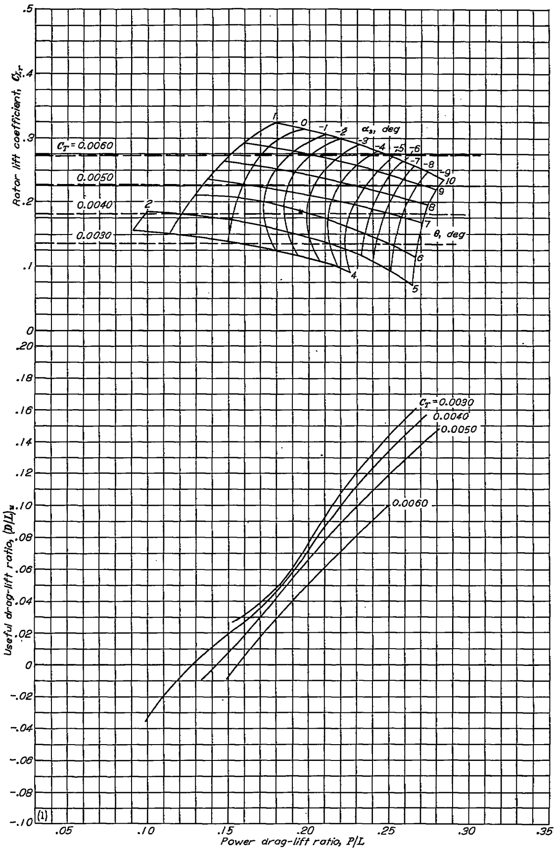
(1) \mu = 0.21 . FIGURE 11.—Continued.
