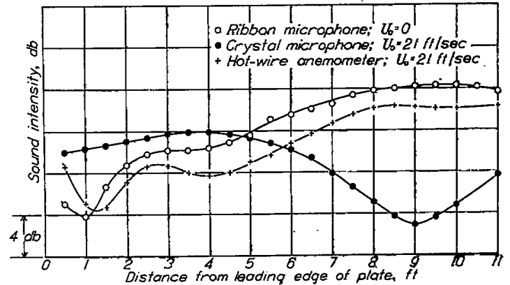
FIGURE 15.—Relative sound intensity from loudspeaker in ceiling of working chamber at leading edge of plate, measured along center 3 inches from plate. Frequency, 60 cycles per second.
