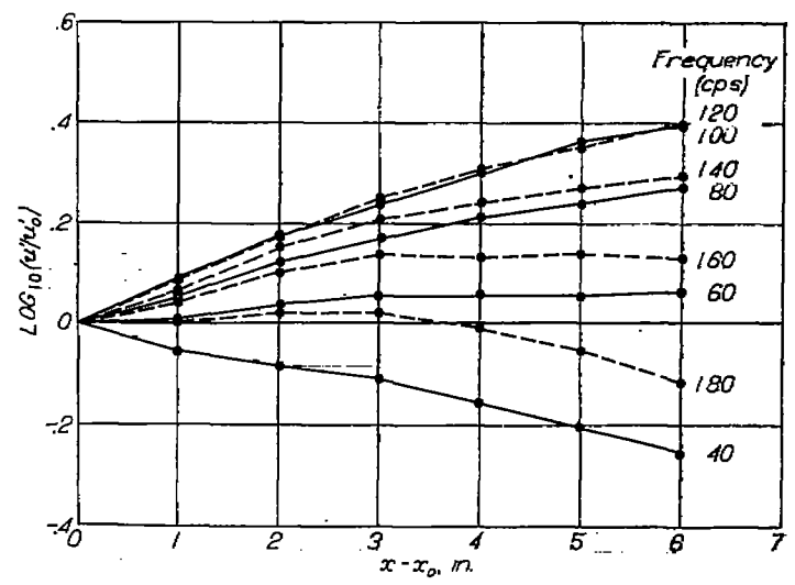
FIGURE 23.—Growth and decay of u -component of oscillations produced by vibrating ribbon 4 feet from leading edge of plate. x_0 , 2 inches downstream from ribbon; U_1=64 feet per second.
