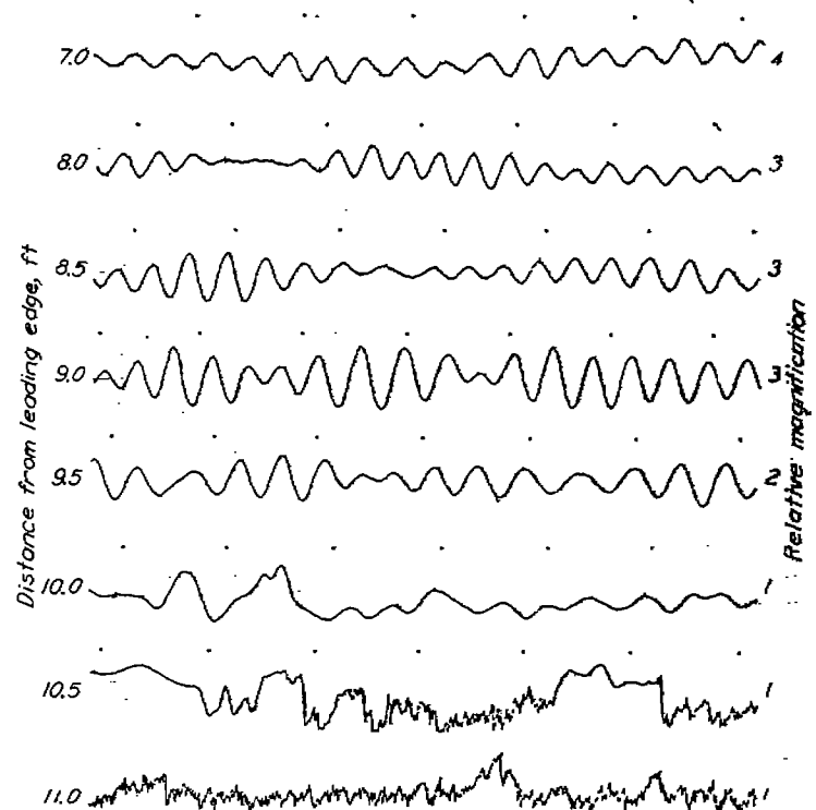
FIGURE 10.—Oscillograms of u -fluctuations showing laminar boundary-layer oscillations in boundary layer of flat plate. Distance from surface, 0.023 inch; U_0=58 feet per second; time interval between dots, \frac{1}{40} second.
