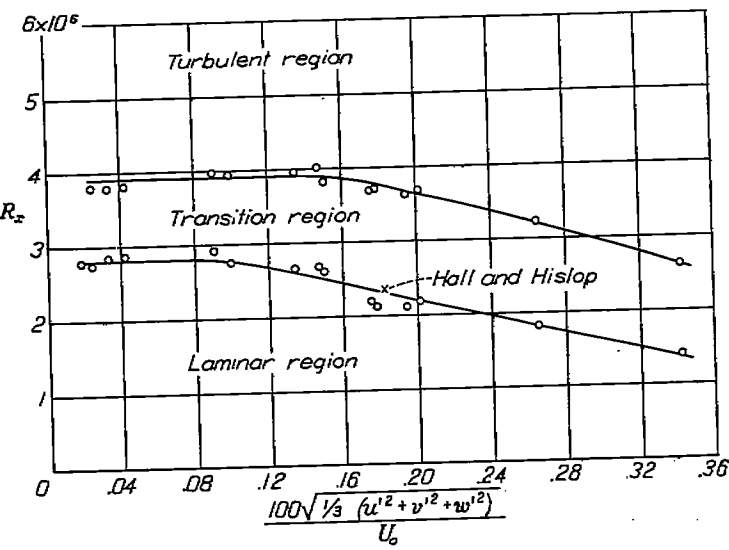
FIGURE 7.—Effect of turbulence on z -Reynolds number of transition. Flat plate; zero pressure gradient.
