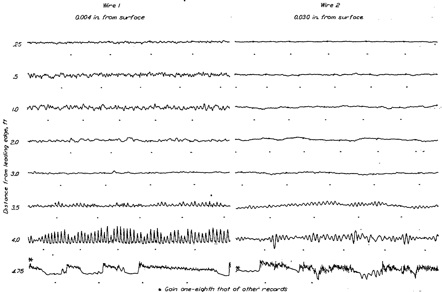
FIGURE 11.—Oscillograms of u -fluctuations showing evidence of frequency doubling near surface. U_1=105 feet per second; time interval between dots, 1/60 second.
