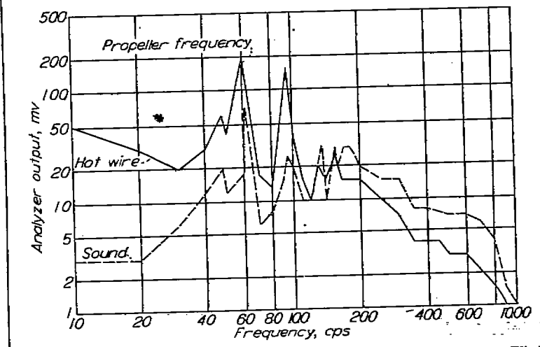
FIGURE 8.—Distribution with frequency of u -component of turbulence and sound. Wind speed, 80 feet per second; u'/U_0 (total) = 0.033 percent.
