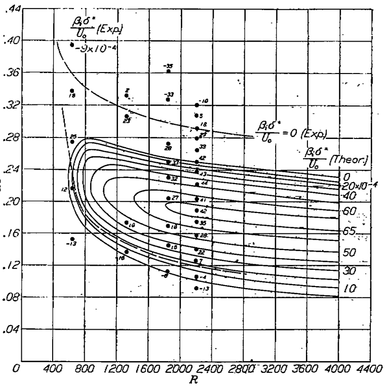
FIGURE 27.—Contours of equal amplification according to Schlichting. Values of \beta_1 \delta^* / U_0 (all values to be multiplied by 10^{-4} ) opposite points are amplifications determined by experiment. Fairred experimental contour of zero amplification shown by broken curves.
