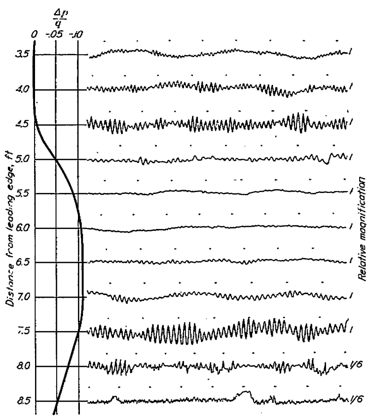
FIGURE 29.—Oscillograms of x -fluctuations showing effect of pressure gradient on boundary-layer oscillations. Distance from surface, 0.021 inch; U_0=95 feet per second; time interval between dots, \frac{1}{30} second.
