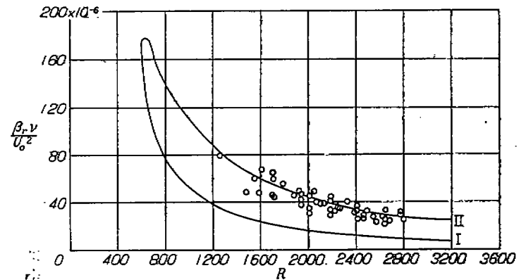
FIGURE 16.—Boundary-layer oscillations excited by loudspeaker. Points show sound frequency giving maximum amplification. Curve outlines theoretical amplification zone. (See fig. 13.)
