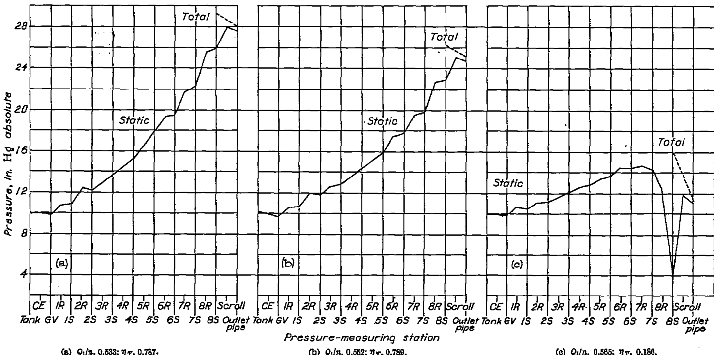
(a) Q/\dot{m} , 0.533; \eta_T , 0.787. (b) Q/\dot{m} , 0.552; \eta_T , 0.789. (c) Q/\dot{m} , 0.565; \eta_T , 0.186. FIGURE 18.—Pressure distribution from inlet tank to outlet pipe with stator blades reset for 75 percent of design speed at load coefficient of 0.65. Compressor Mach number, 0.7; inlet-air temperature, 0° F; inlet-air pressure, 10.16 inches mercury absolute. Pressure measurements made after each blade row. OE, at compressor entrance; GV, after guide vanes; R, after rotor blades; S, after stator blades.
