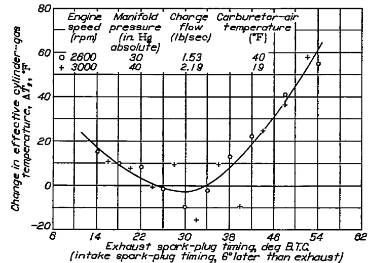
FIGURE 24.—Variation of change in effective cylinder-gas temperature with ignition timing for coolant-heat-rejection correlation. Fuel-air ratio, 0.095.
