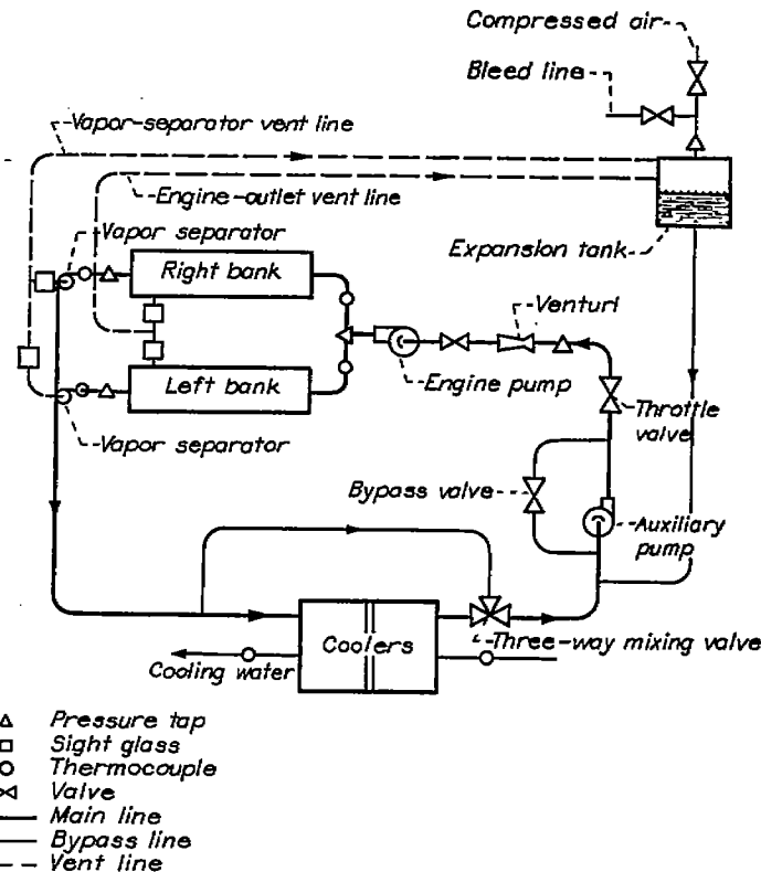
FIGURE 2.—Schematic diagram of engine coolant system.
