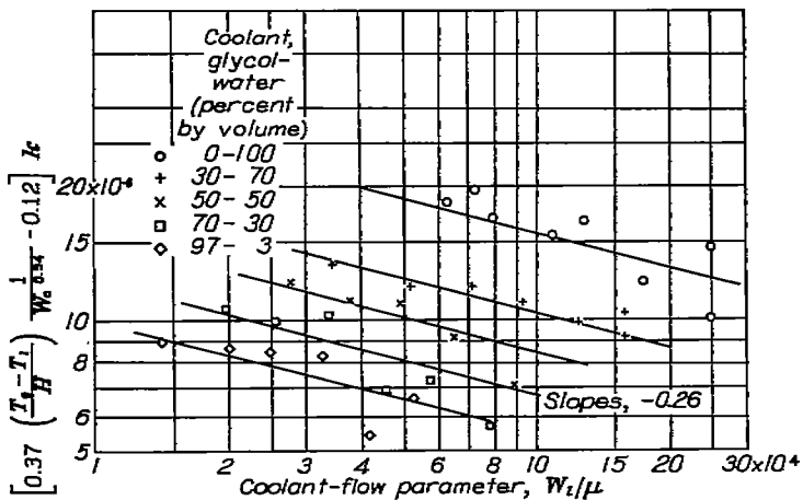
FIGURE 28.—Determination of exponent m on coolant-flow parameter W_i/\mu for coolant-heat-rejection correlation from variation of \left[0.37 \left(\frac{T_g - T_l}{H}\right) - \frac{1}{W_c^{0.94}} - 0.12\right] k with \frac{W_i}{\mu} for various coolants. Average coolant temperature, 245° F.
