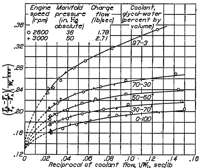
FIGURE 9.—Determination of factor Z from variation of \left(\frac{T_h - T_i}{T_g - T_h}\right) \left(\frac{1}{W_c^{0.60}}\right) with 1/W_i for cylinder-head-temperature correlation. Average coolant temperature, 245° F; engine D.
