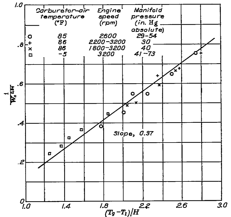
FIGURE 26.—Variation of 1/W_c^{0.94} with (T_g - T_i)/H . Fuel-air ratio, 0.095; exhaust pressure, 29-30 inches mercury absolute; standard ignition timing.
