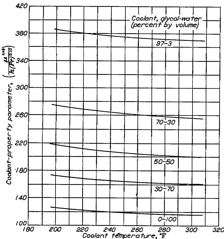
FIGURE 16.—Variation of coolant-property parameter \left(\frac{\mu^{0.48}}{k(P_r)^{0.38}}\right) with coolant temperature for cylinder-head-temperature correlation.
