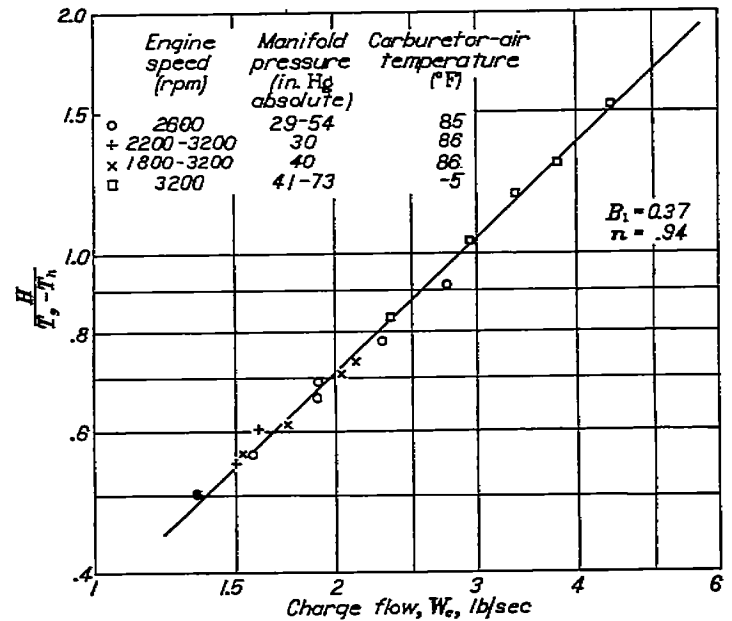
FIGURE 25.—Determination of exponent n and constant B_1 or coolant-heat-rejection correlation from variation of H/(T_g - T_i) with W_c . Fuel-air ratio, 0.095; exhaust pressure, 29-30 inches mercury absolute; standard ignition timing.
