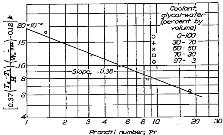
FIGURE 29.—Determination of exponent s on Prandtl number Pr for coolant-heat-rejection correlation from variation of \left[0.37 \left(\frac{T_g - T_l}{H}\right) - \frac{1}{W_c^{0.94}} - 0.12\right] k with Pr as obtained from cross plot of figure 28 at value of \frac{W_i}{\mu} of 55,000. Average coolant temperature, 245° F.
