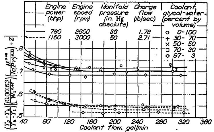
FIGURE 17.—Variation of \left(\frac{T_g - T_h}{T_h - T_i}\right) \left[ \left(\frac{0.00163}{W_i^{0.48}}\right) \left(\frac{\mu^{0.48}}{k(P_r)^{0.38}}\right) + Z \right] with coolant flow as indication of boiling. Average coolant temperature, 245^\circ F; engine D.
