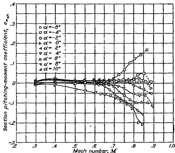
FIGURE 41.—The variation of section quarter-chord moment coefficient with Mach number at various angles of attack for the NACA 847C110 airfoil.
