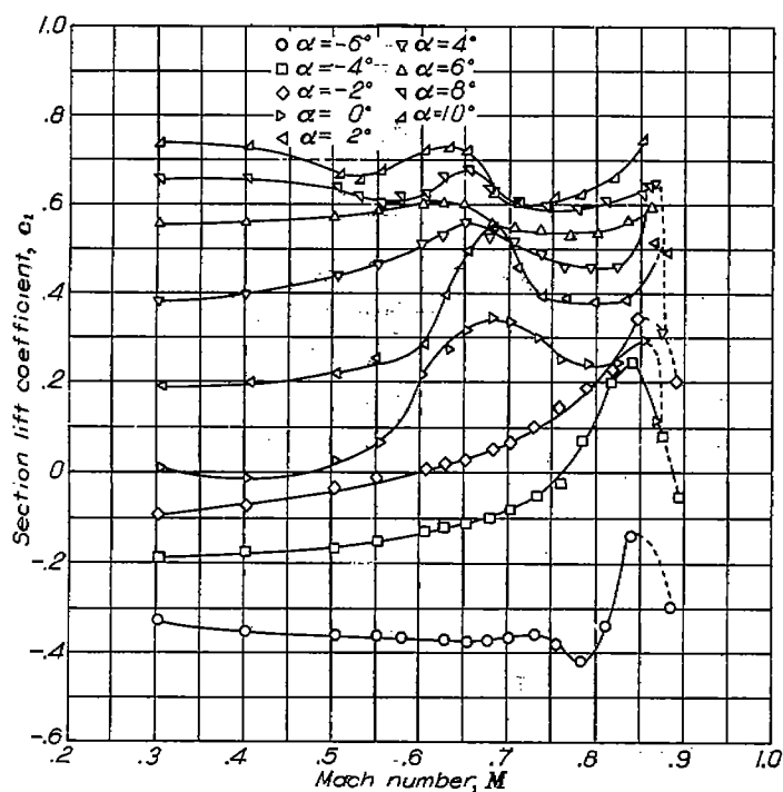
FIGURE 5.—The variation of section lift coefficient with Mach number at various angles of attack for the NACA 847A216 airfoil.
