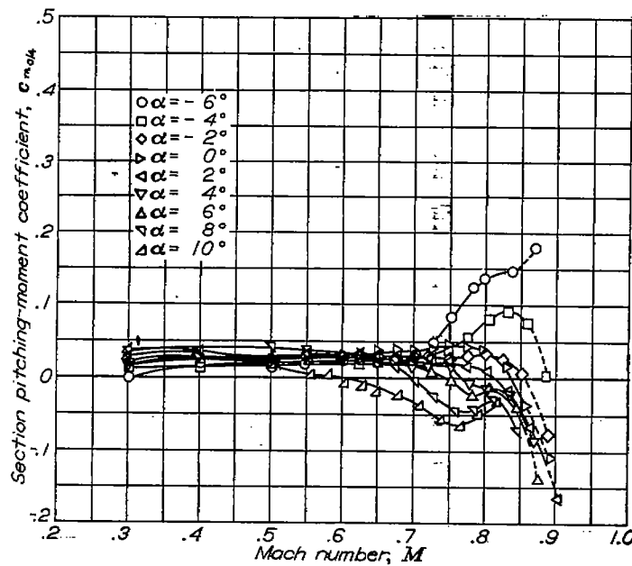
FIGURE 39.—The variation of section quarter-chord moment coefficient with Mach number at various angles of attack for the NACA 847A110 airfoil.
