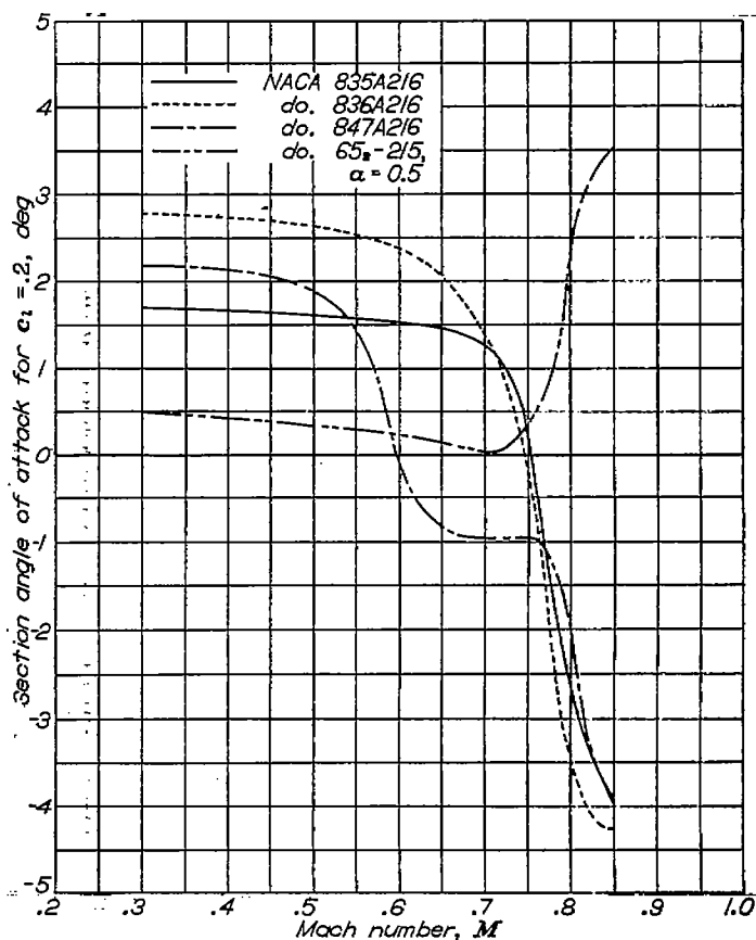
FIGURE 6.—The variation with Mach number of the section angle of attack for a lift coefficient of 0.2 for the NACA 835A216, 836A216, 847A216 and 65-215. \alpha = 0.5 , airfoils.
