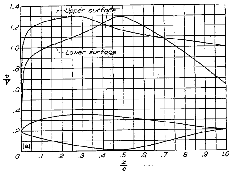
(a) NACA 835A210 airfoil.
