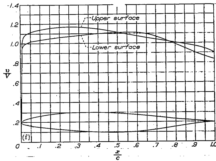
(f) NACA 836D110 airfoil.
