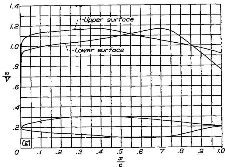
(g) NACA 847A110 airfoil.
