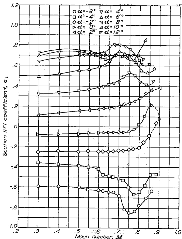
FIGURE 31.—The variation of section lift coefficient with Mach number at various angles of attack for the NACA 847A110 airfoil.
