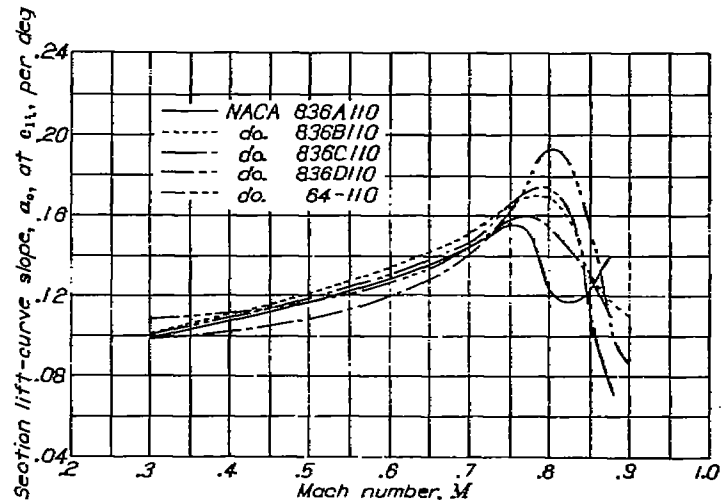
FIGURE 19.—The variation with Mach number of the section lift-curve slope at the design lift coefficient for the NACA 836A110, 836B110, 836C110, 836D110 and the 64-110 airfoils.
