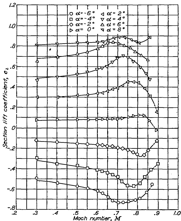
FIGURE 13.—The variation of section lift coefficient with Mach Number at various angles of attack for the NACA 64-110 airfoil.
