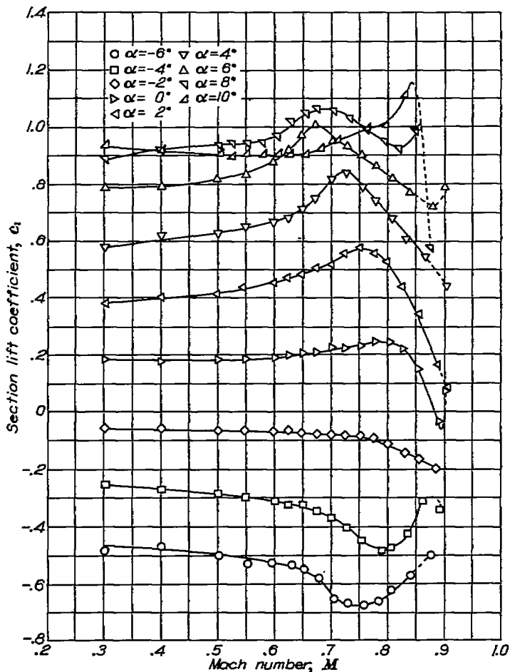
FIGURE 42.—The variation of section lift coefficient with Mach number at various angles of attack for the NACA 65-210 airfoil with a 20-percent-chord plain flap. \alpha_i, 0^\circ .
