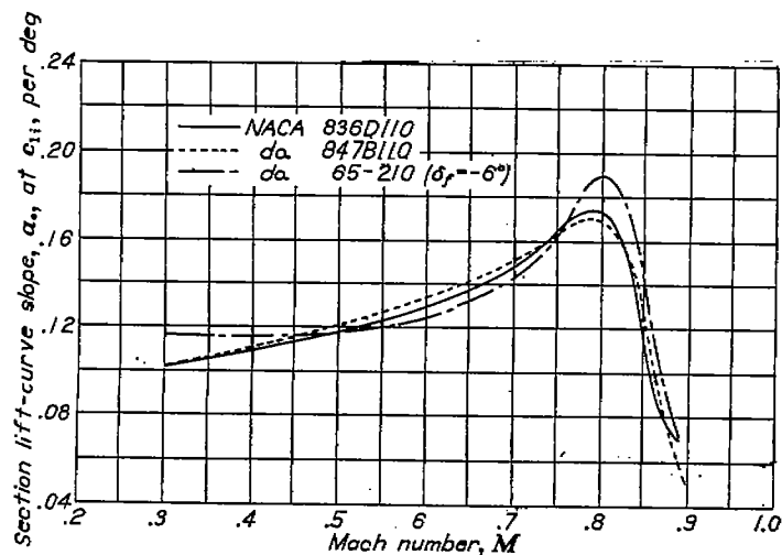
FIGURE 44.—The variation with Mach number of the section lift-curve slope at a lift coefficient of 0.1 for the NACA 65-210 ( \delta_f = -6^\circ ), 836D110 and 847B110 airfoils.
