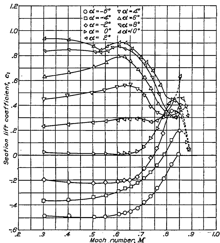
FIGURE 3.—The variation of section lift coefficient with Mach number at various angles of attack for the NACA 835A216 airfoil.
