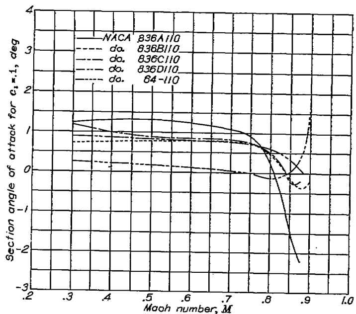
FIGURE 20.—The variation with Mach number of the section angle of attack for a lift coefficient of 0.1 for the NACA 836A110, 836B110, 836C110, 836D110 and 64-110 airfoils.
