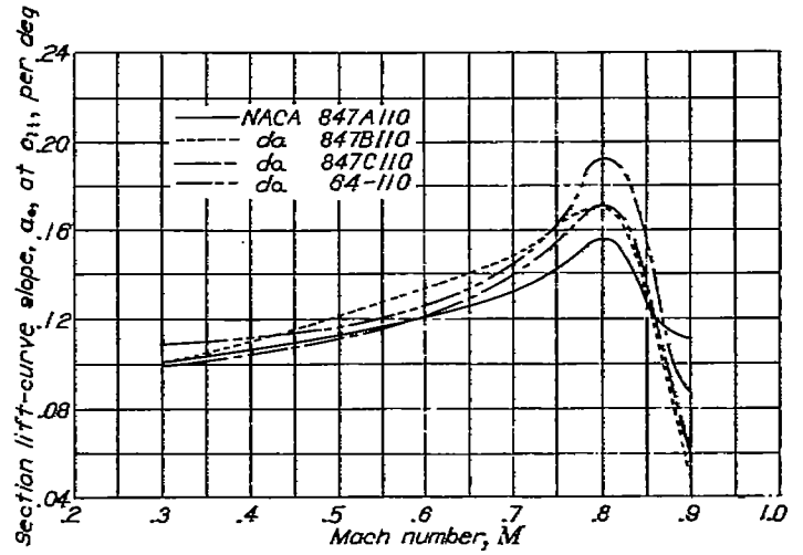
FIGURE 34.—The variation with Mach number of the section lift-curve slope at the design lift coefficient for the NACA 847A110, 847B110, 847C110 and 64-110 airfoils.
