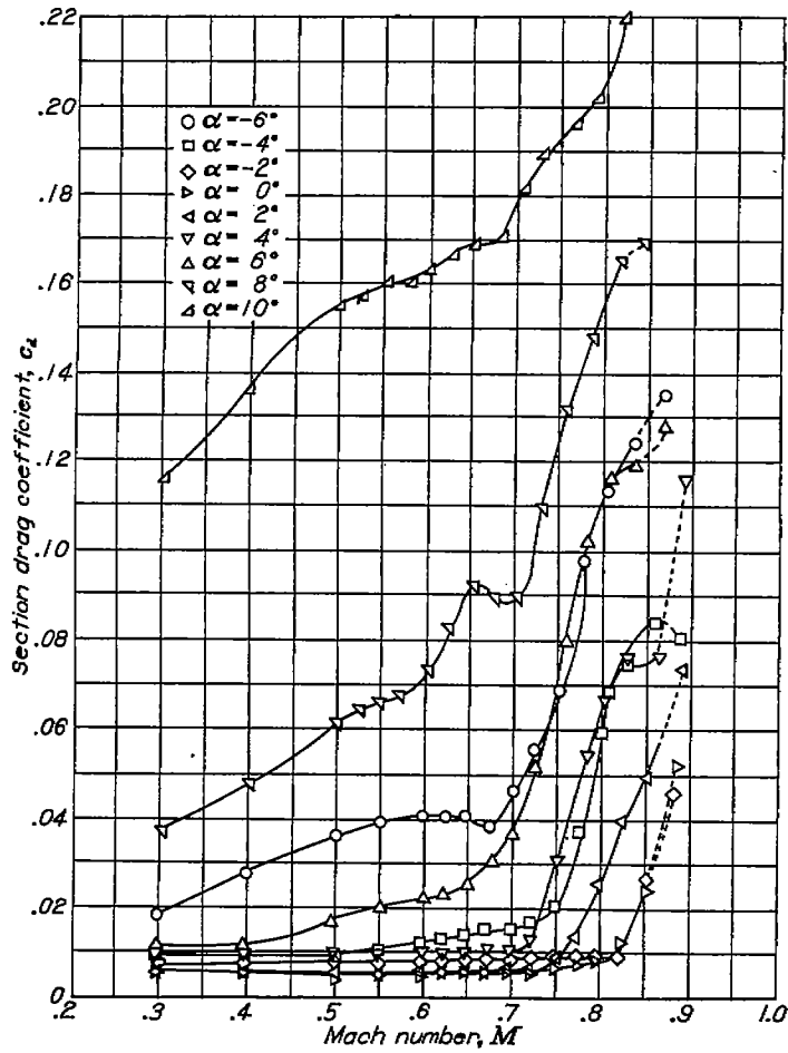
FIGURE 37.—The variation of section drag coefficient with Mach number at various angles of attack for the NACA 847B110 airfoil.
