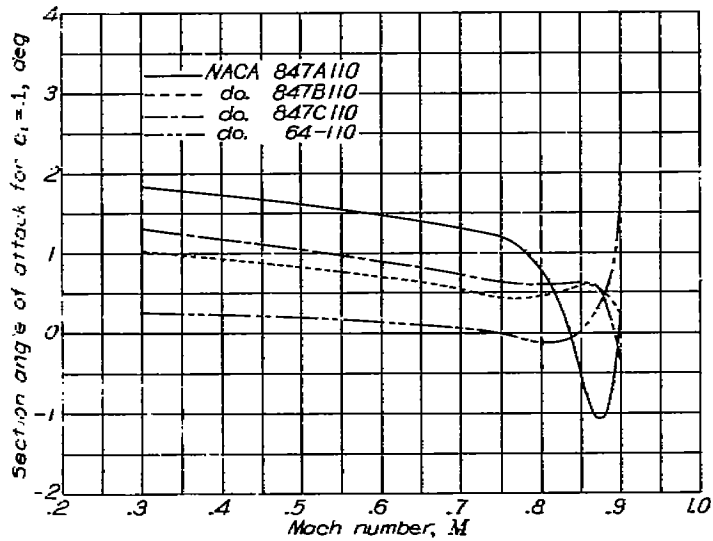
FIGURE 35.—The variation with Mach number of the section angle of attack for a lift coefficient of 0.1 for the NACA 847A110, 847B110, 847C110, and 64-110 airfoils.
