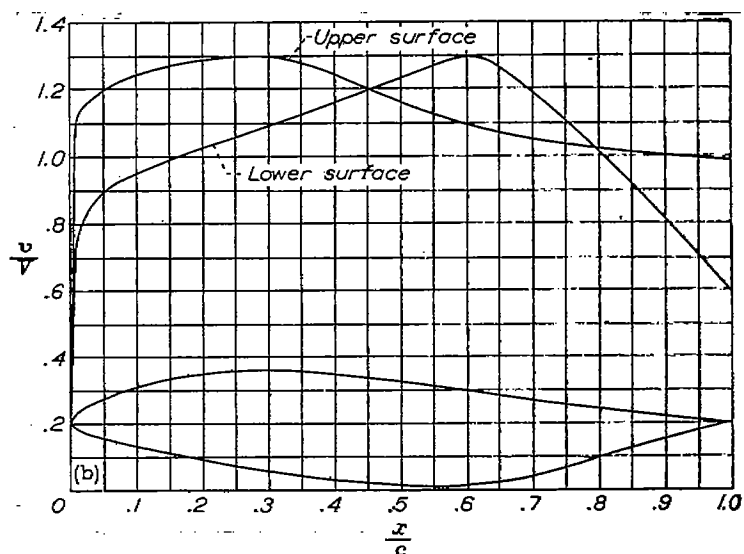
(b) NACA 836A210 airfoil.
