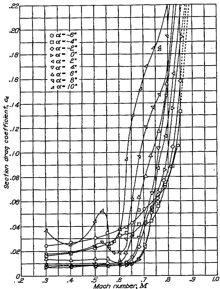
FIGURE 8.—The variation of section drag coefficient with Mach number at various angles of attack for the NACA 835A216 airfoil.
