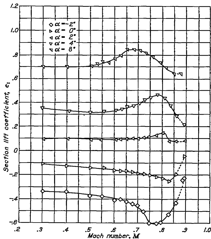
FIGURE 43.—The variation of section lift coefficient with Mach number at various angles of attack for the NACA 65-210 airfoil with a 20-percent-chord plain flap. \alpha_i, -6^\circ .
