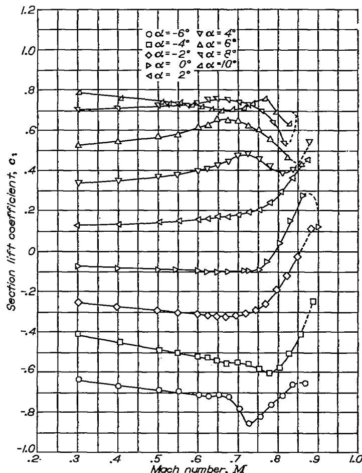
FIGURE 14.—The variation of section lift coefficient with Mach number at various angles of attack for the NACA 836A110 airfoil.
