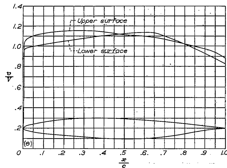
(e) NACA 836B110 airfoil.
