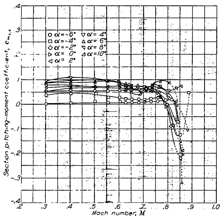
FIGURE 12.—The variation of section quarter-chord moment coefficient with Mach number at various angles of attack for the NACA 836A216 airfoil.
