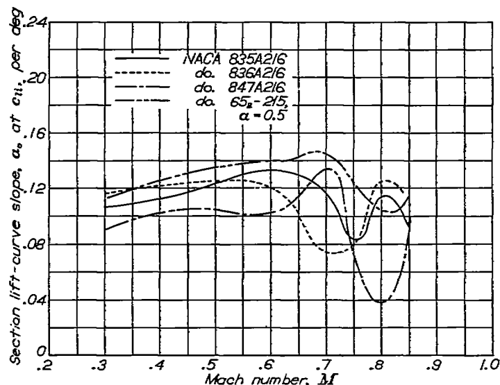
FIGURE 7.—The variation with Mach number of the section lift-curve slope at the design lift coefficient for the NACA 835A216, 836A216, 847A216 and 65 2 -215, \alpha=0.5 , airfoils.
