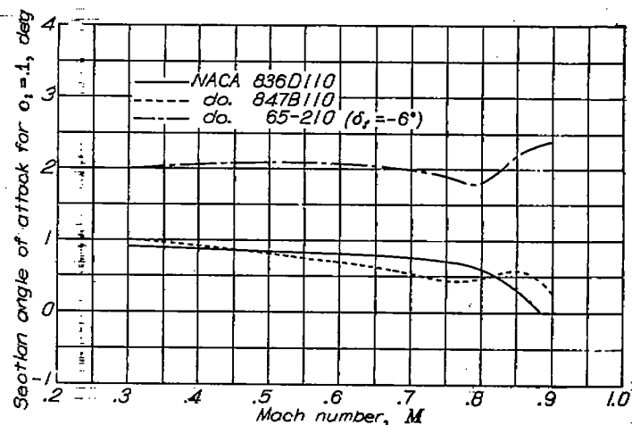
FIGURE 45.—The variation with Mach number of the angle of attack for a lift coefficient of 0.1 for the NACA 65-210 ( \delta_f = -6^\circ ), 836D110 and 847B110 airfoils.
