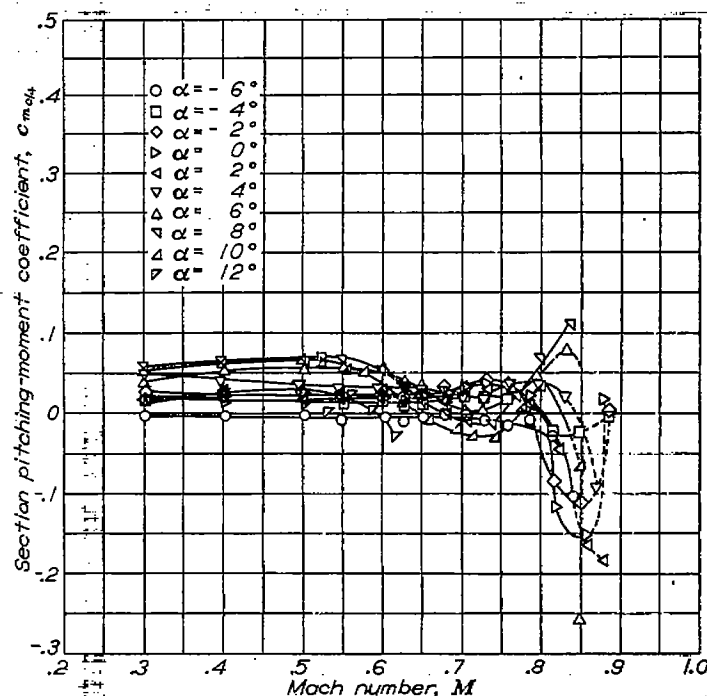
FIGURE 11.—The variation of section quarter-chord moment coefficient with Mach number at various angles of attack for the NACA 835A216 airfoil.
