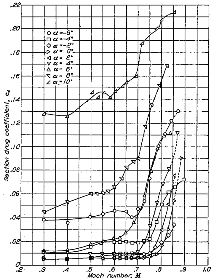
FIGURE 23.—The variation of section drag coefficient with Mach number at various angles of attack for the NACA 836C110 airfoil.
