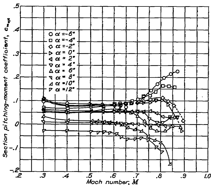
FIGURE 28.—The variation of section quarter-chord moment coefficient with Mach number at various angles of attack for the NACA 836C110 airfoil.
