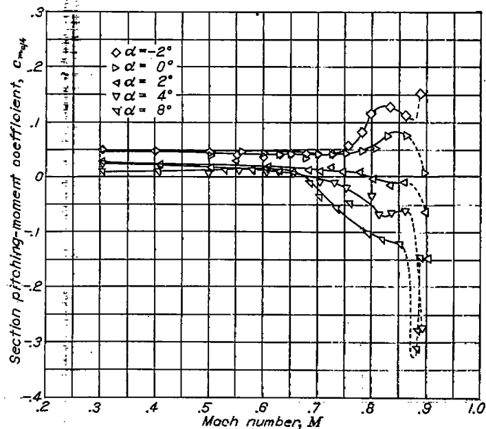
FIGURE 47.—The variation of section quarter-chord moment coefficient at various angles of attack for the NACA 65-210 airfoil with a 20-percent-chord plain flap. \delta_f = -6^\circ .
