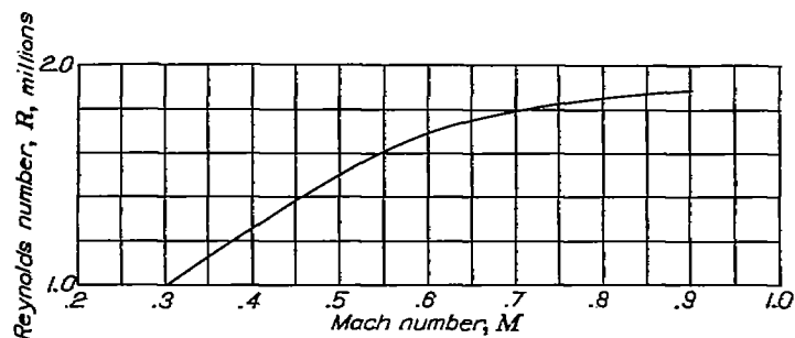
FIGURE 2.—The variation of Reynolds number with Mach number for tests of 6-inch-chord airfoil models in the Ames 1- by 3¼-foot high-speed wind tunnel.
