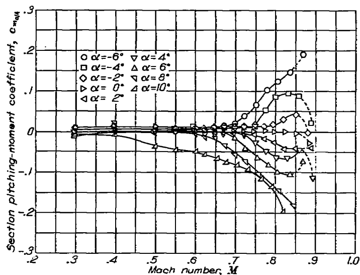
FIGURE 40.—The variation of section quarter-chord moment coefficient with Mach number at various angles of attack for the NACA 847B110 airfoil.
