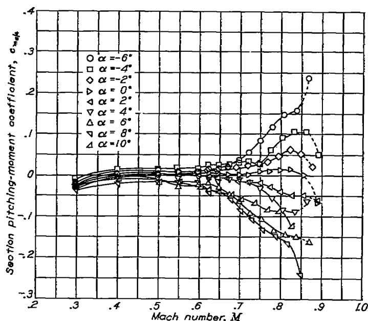
FIGURE 29.—The variation of section quarter-chord moment coefficient with Mach number at various angles of attack for the NACA 836D110 airfoil.
