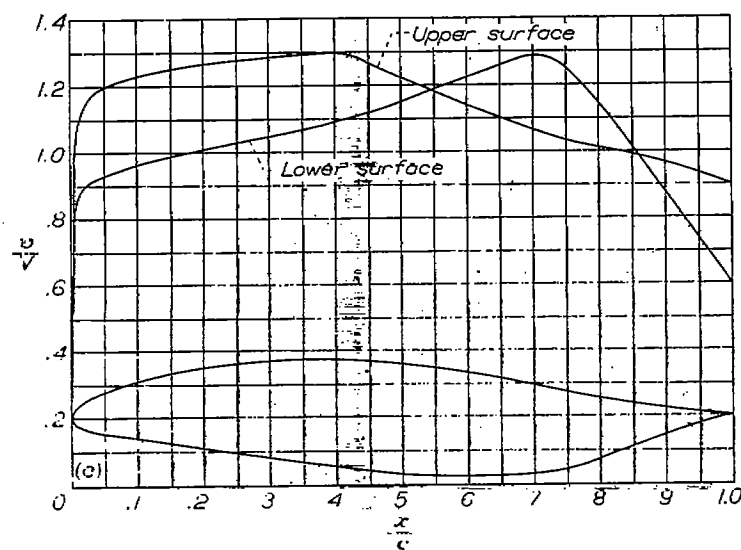
(c) NACA 847A210 airfoil.
