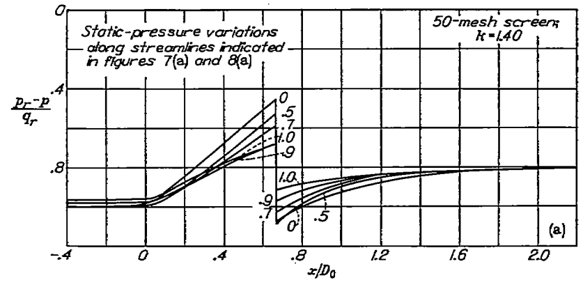
(a) Screens placed \frac{3}{4} duct diameter from diffuser entrance.
