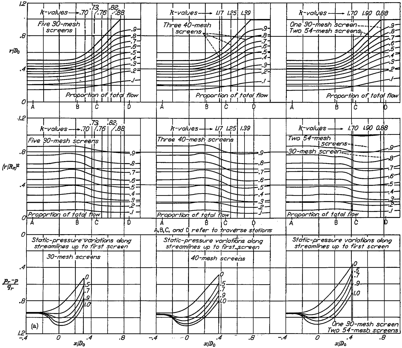
(a) Charts showing streamline patterns, proportion of diffuser area filled by various proportions of total flow, and static-pressure distributions along selected streamlines FIGURE 10.—Results of tests of diffuser B with various multiple-screen combinations
