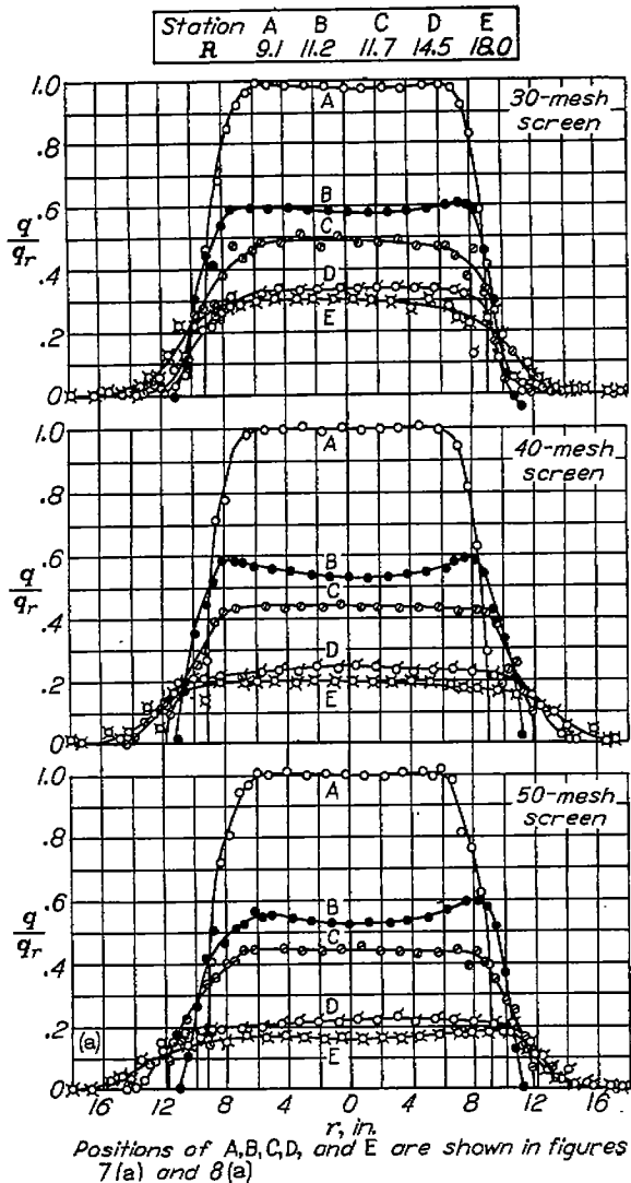
FIGURE 8.—Results of tests of diffuser A with various single screens. Charts showing dynamic-pressure distributions at various diffuser sections and proportions of diffuser area filled by various proportions of total flow.
