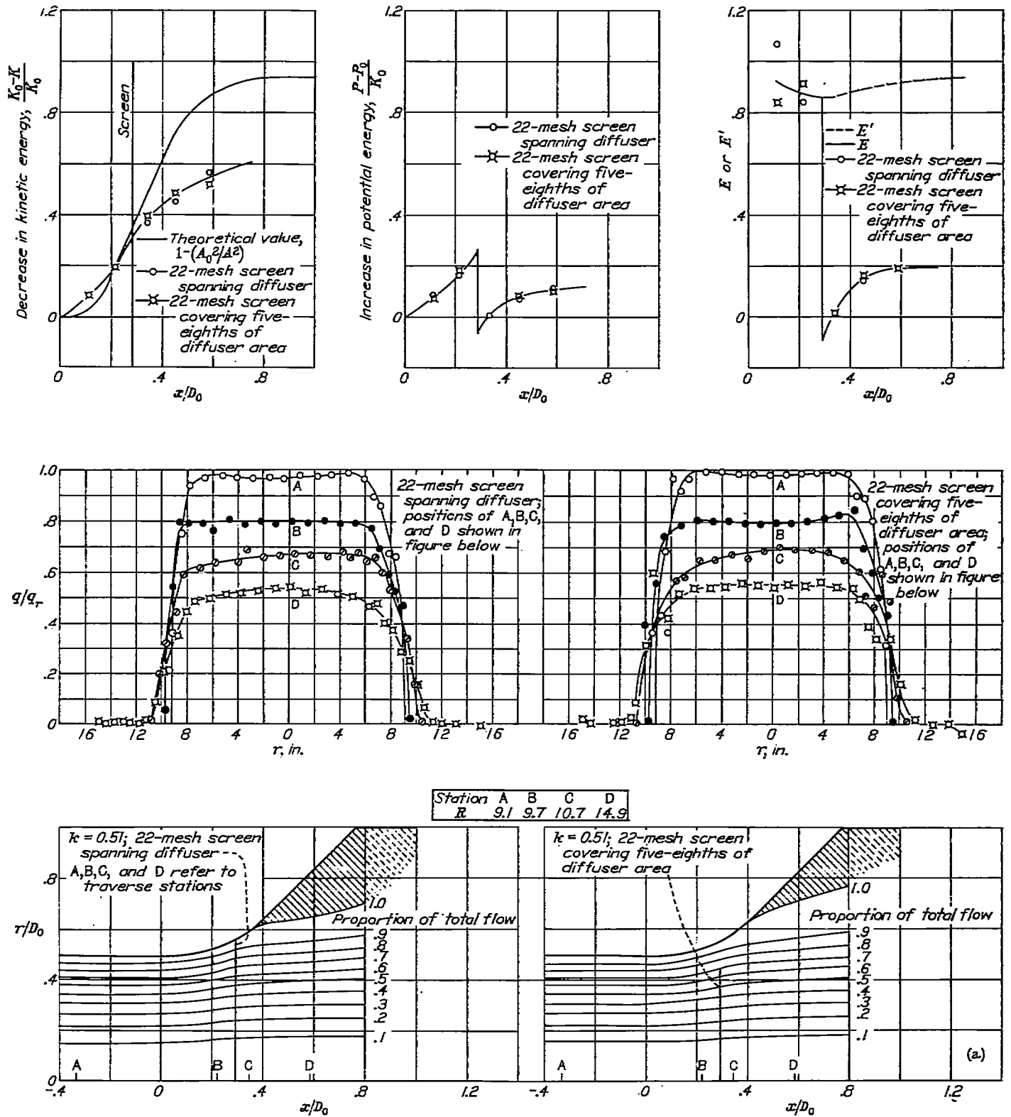
(a) Single 22-mesh screen placed 0.29 duct diameter from diffuser entrance. (See also fig. 13 (a).)
