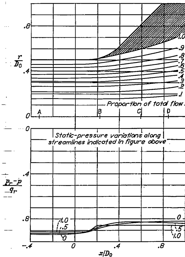
FIGURE 10.—Results of tests of diffuser B without screens. Charts showing changes in kinetic and potential energies, efficiency, dynamic- and static-pressure distributions at various diffuser sections, approximate streamline pattern, and static-pressure distributions along selected streamlines.
