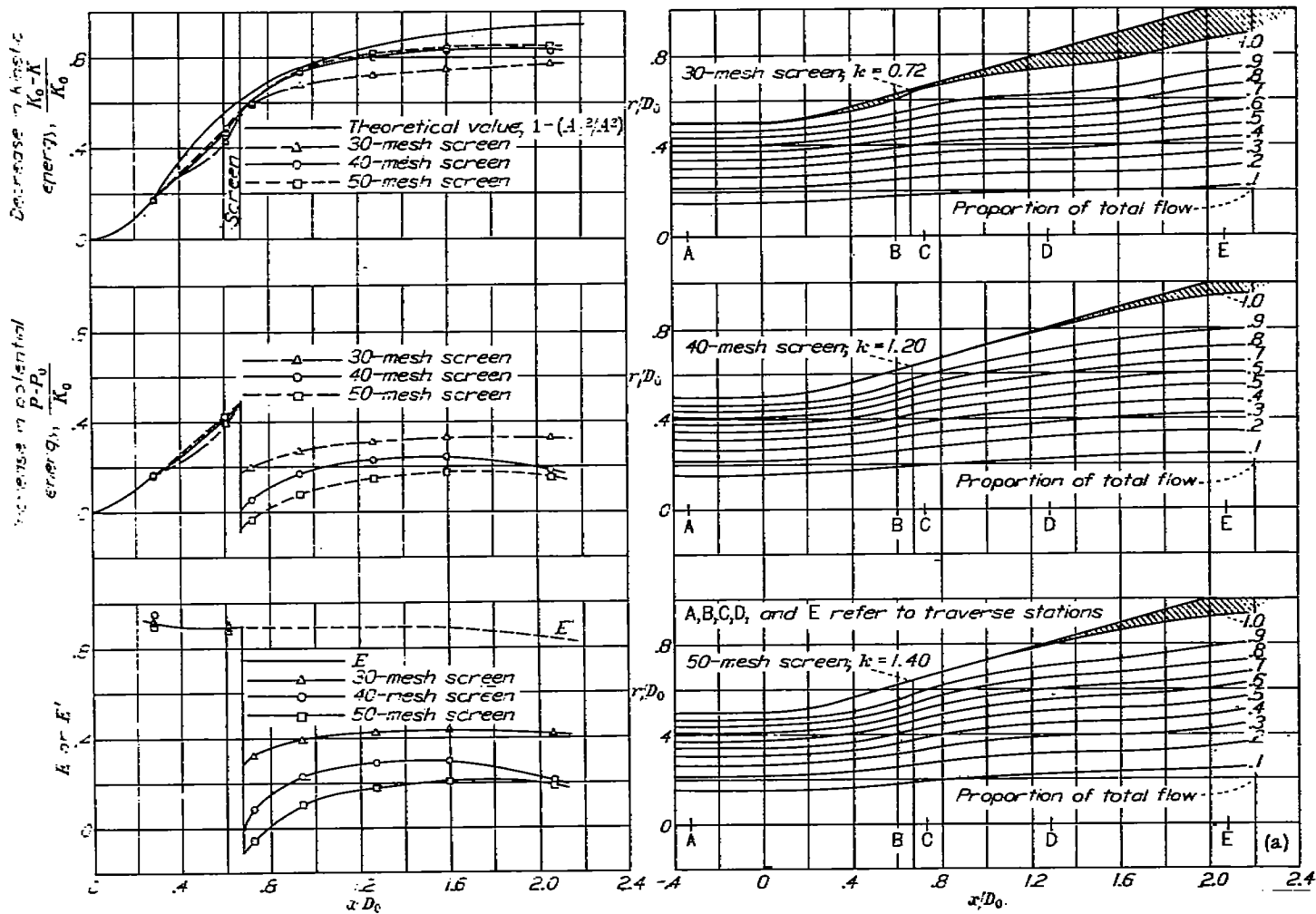
(a) Screens placed \frac{1}{2} duct diameter from diffuser entrance.
