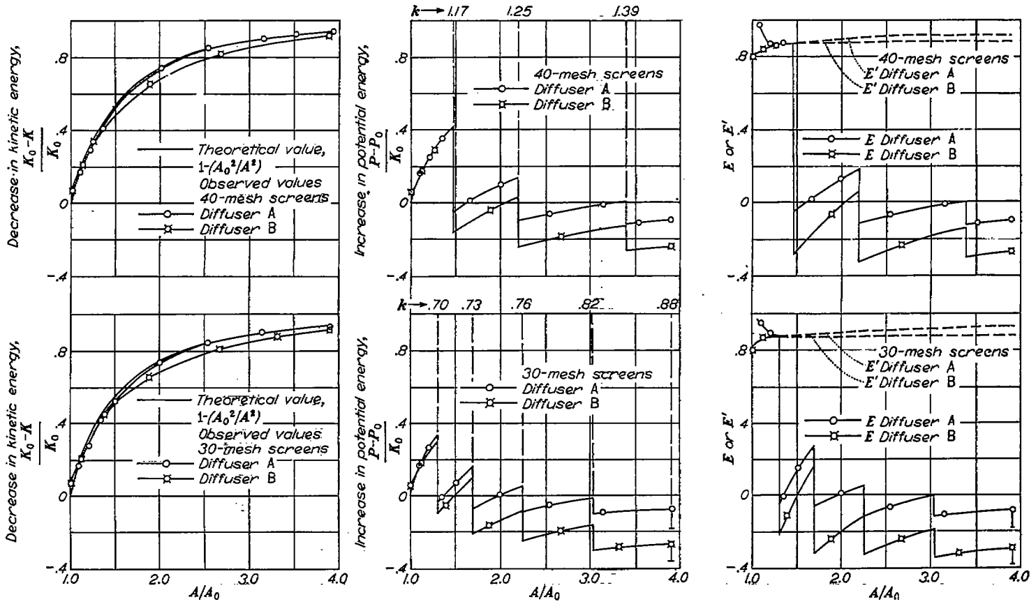
FIGURE 17.—Comparison of test results of diffusers A and B with the 30- and 40-mesh multiple-screen combinations shown in figures 15 and 16. Charts showing changes in kinetic and potential energies and efficiencies.
