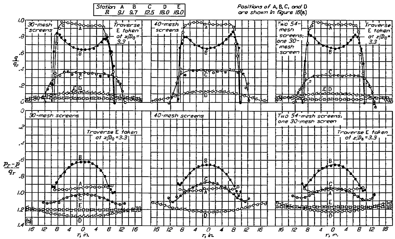
(b) Charts showing changes in kinetic and potential energies, efficiencies, and dynamic- and static-pressure distributions at various diffuser sections.
