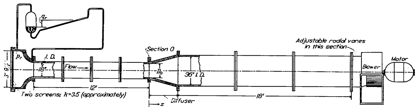
FIGURE 1.—Diffuser and duct-system assembly used to study effects of fine screens in diffusers.
