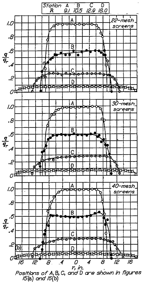
(b) Charts showing dynamic-pressure distributions at various diffuser sections and proportion of diffuser area filled by various proportions of total flow.
