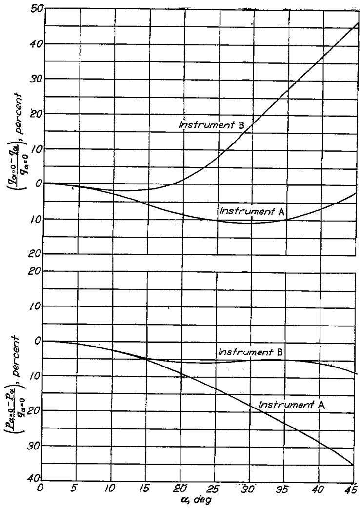
FIGURE 4.—Pitot-static-tube characteristics.
