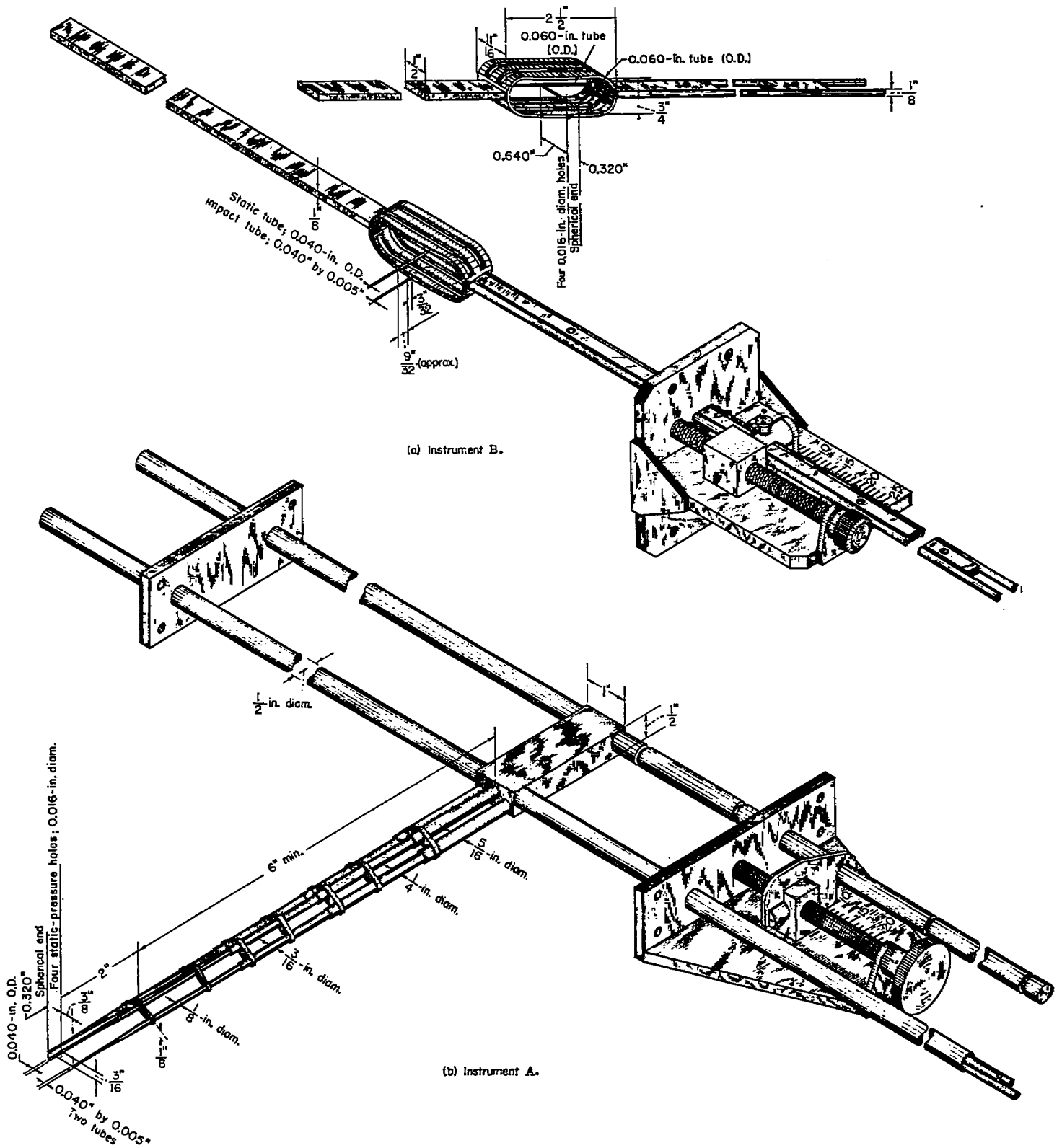
FIGURE 3.—Pitot-static-tube assemblies. Instrument A used in back of screens; instrument B used ahead of and between screens.
