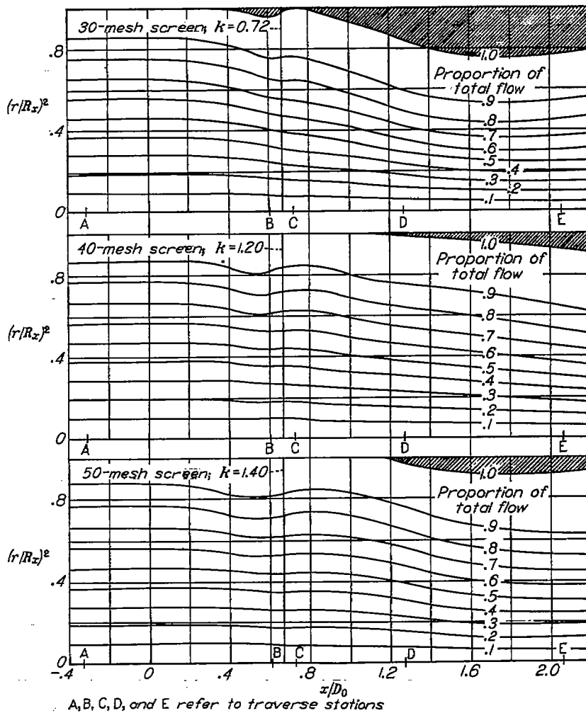
(a) Screens placed \frac{1}{4} duct diameter from diffuser entrance.
