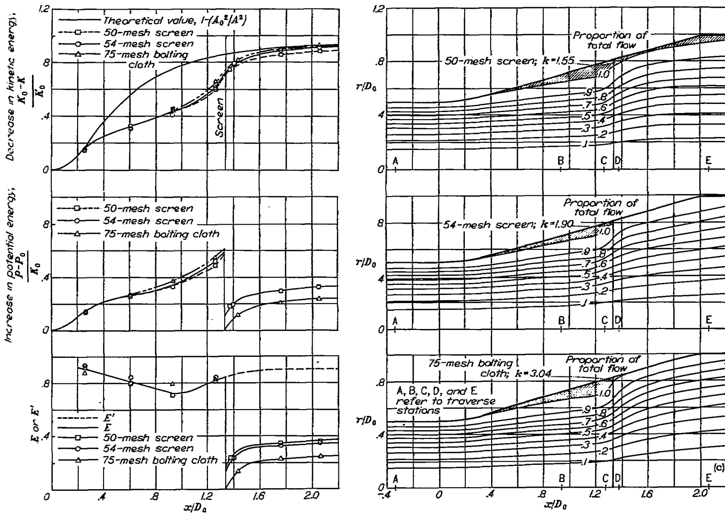
(c) Screens placed 1\frac{1}{4} duct diameters from diffuser entrance
