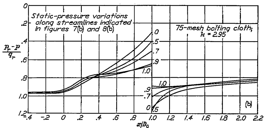
(b) Screens placed 1.0 duct diameter from diffuser entrance.
