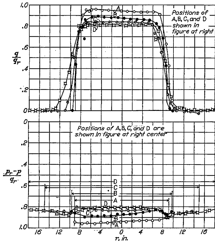
FIGURE 10.—Results of tests of diffuser B without screens. Charts showing changes in kinetic and potential energies, efficiency, dynamic- and static-pressure distributions at various diffuser sections, approximate streamline pattern, and static-pressure distributions along selected streamlines.
