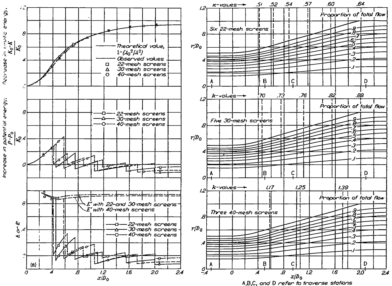
(a) Charts showing changes in kinetic and potential energies, efficiencies, and streamlines.
