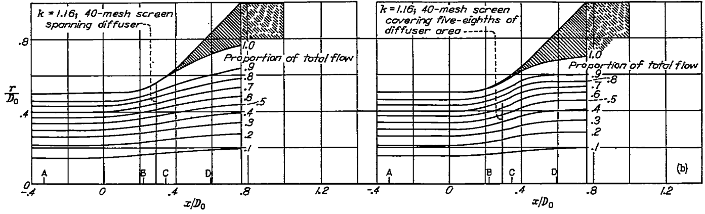
(b) Single 40-mesh screen placed 0.20 duct diameter from diffuser entrance. (See also fig. 12 (b).)
