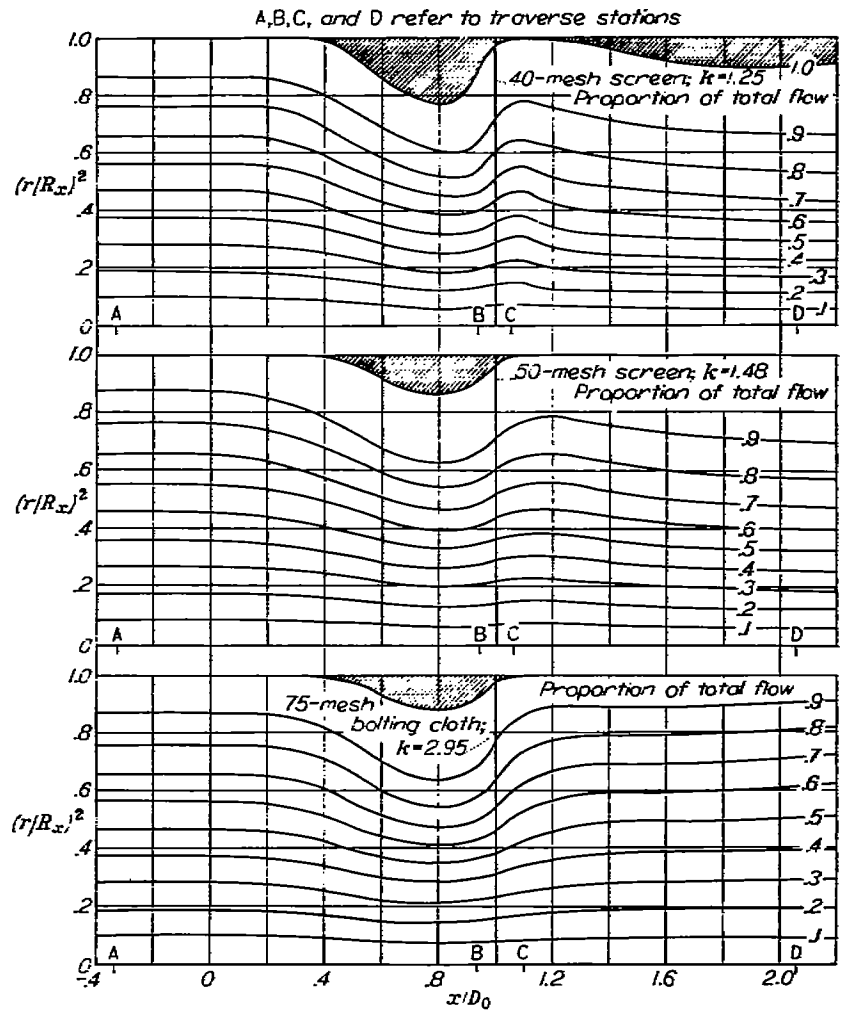
(b) Screens placed 1.0 duct diameter from diffuser entrance.
