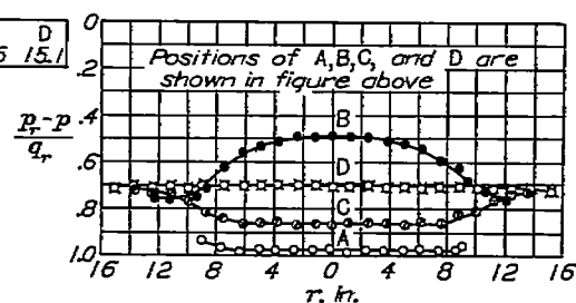
FIGURE 13.—Results of tests of diffuser C with 40-mesh screen.
