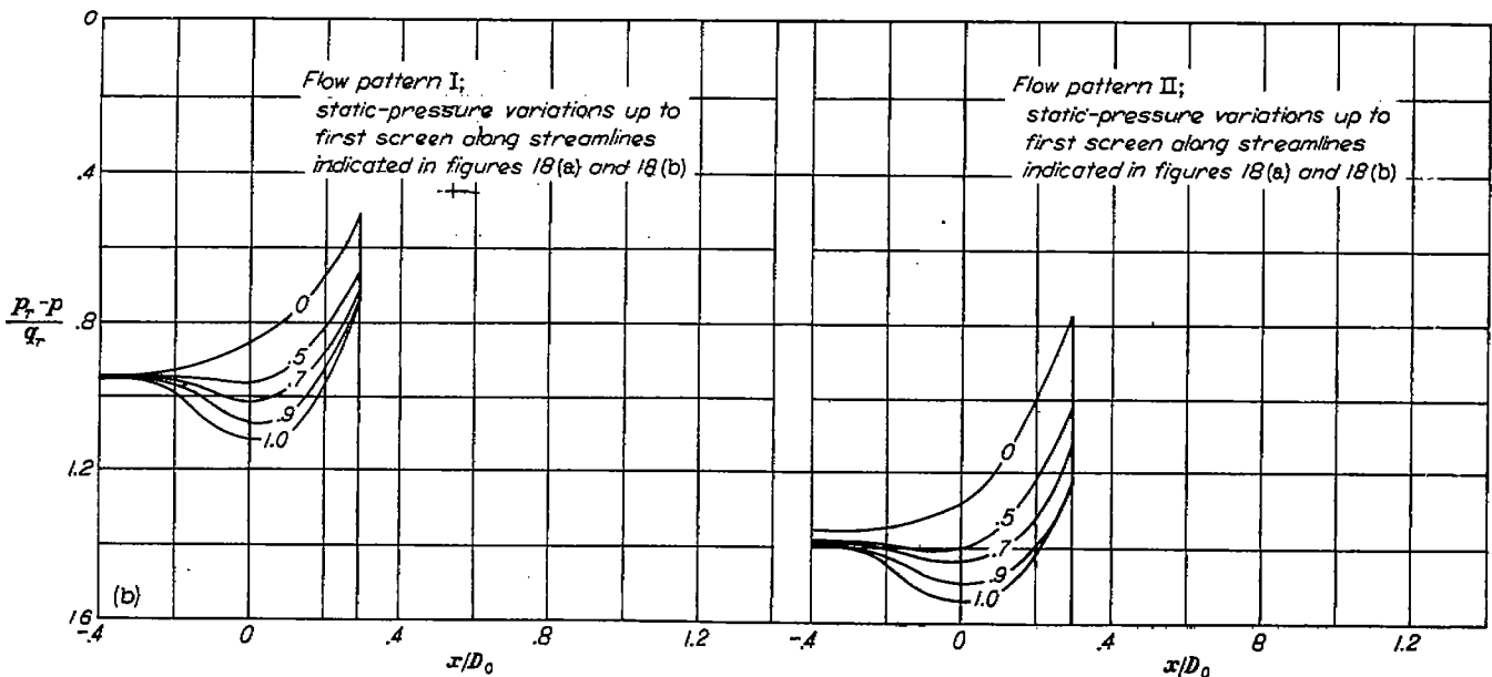
(b) Charts showing proportion of diffuser area filled by various proportions of total flow, static-pressure distributions at various diffuser sections, and static-pressure distributions along selected streamlines.
