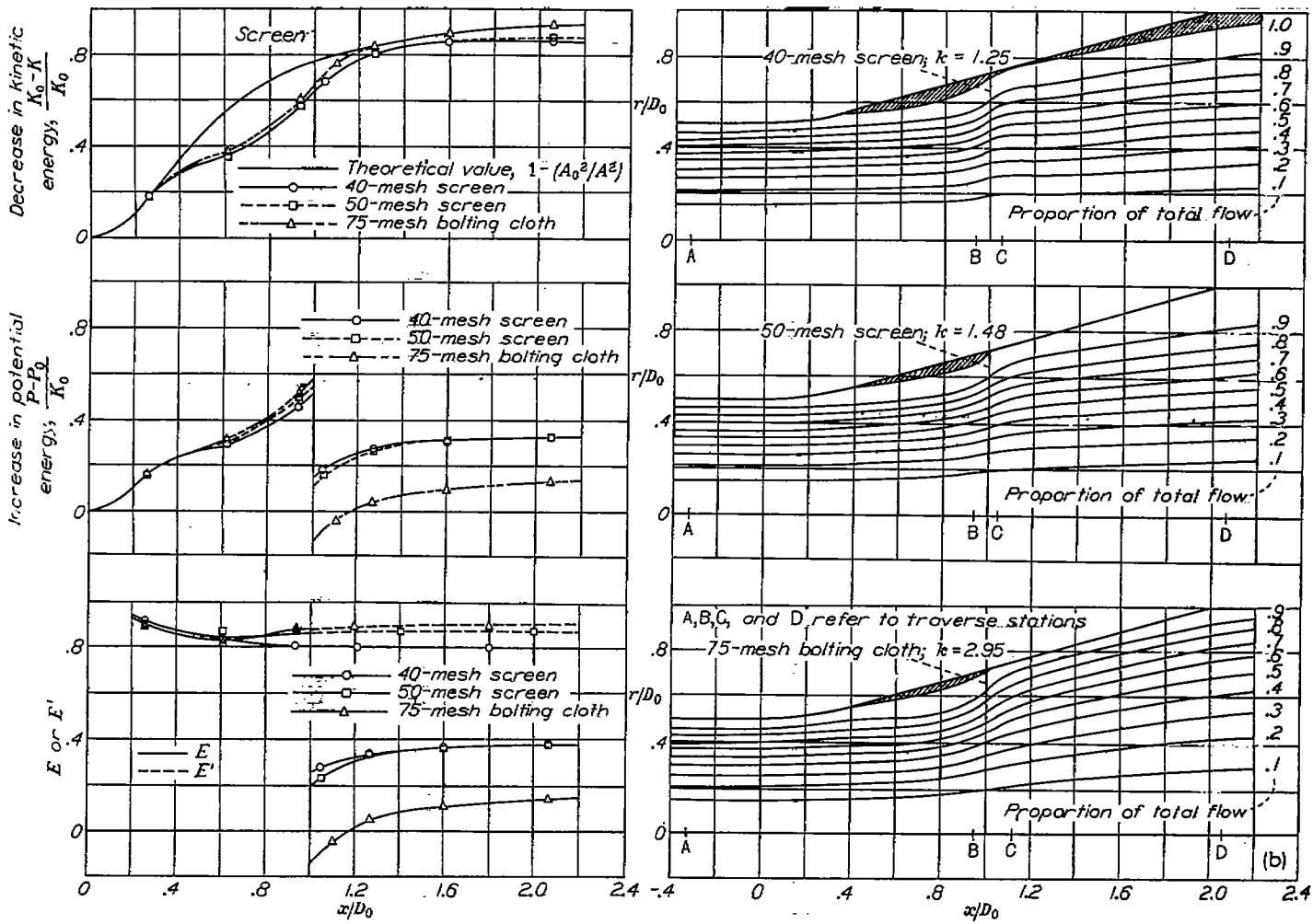
(b) Screens placed 1.0 duct diameter from diffuser entrance.
