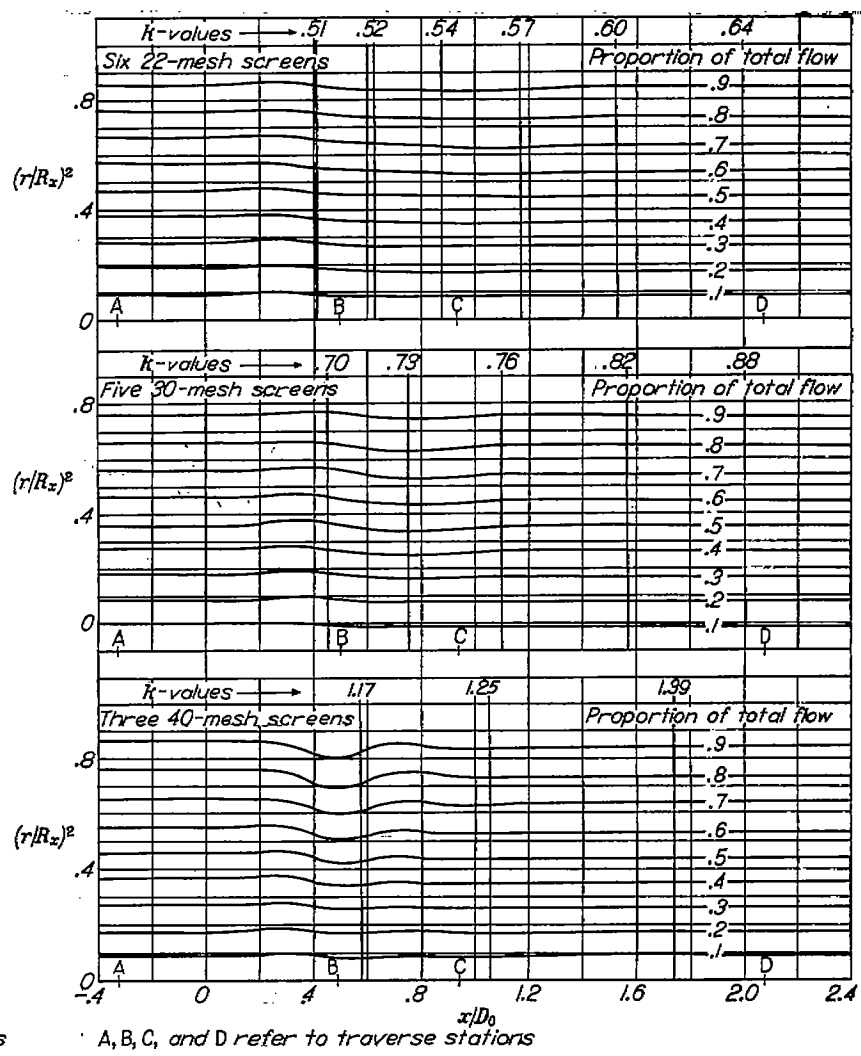
(b) Charts showing dynamic-pressure distributions at various diffuser sections and proportion of diffuser area filled by various proportions of total flow.
