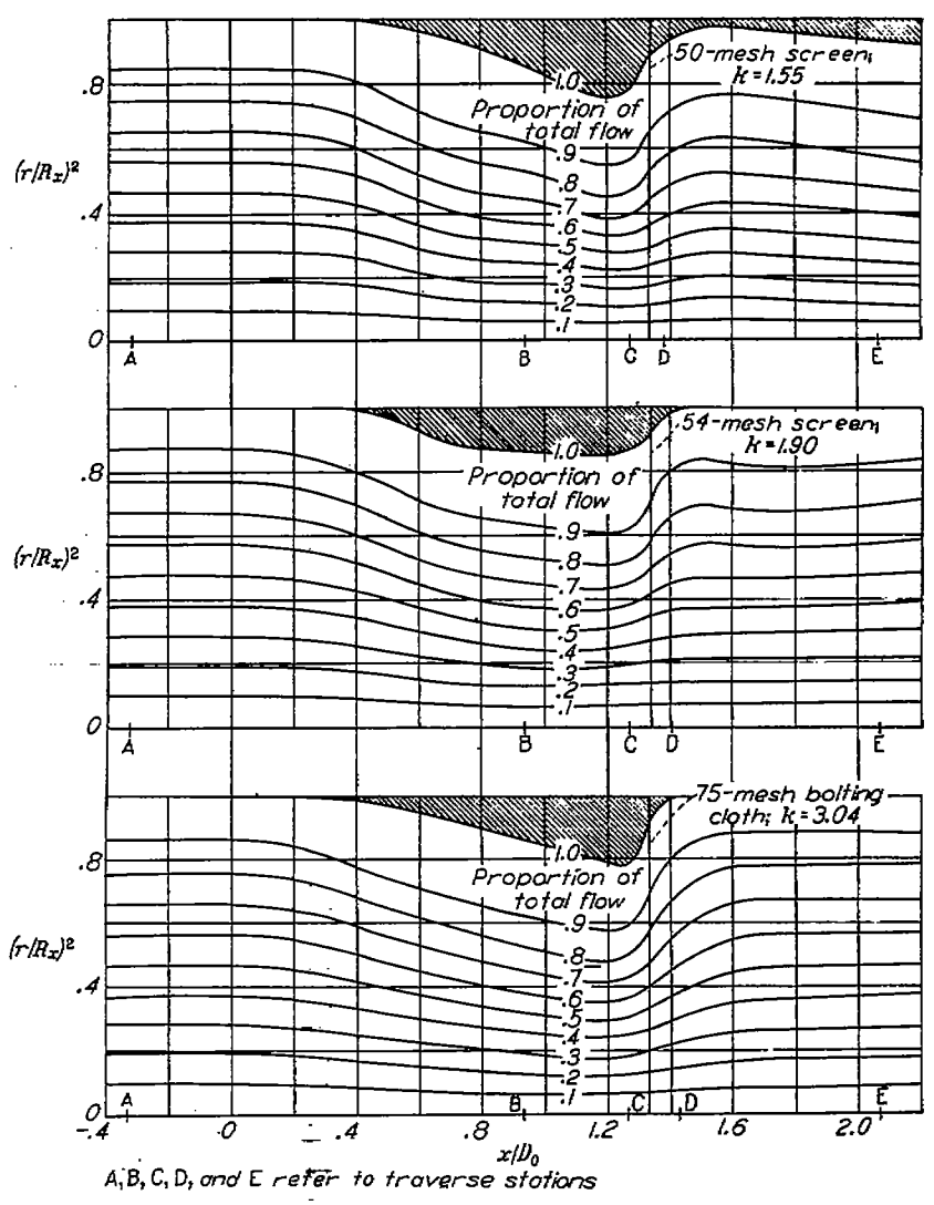
(c) Screens placed 1\frac{1}{4} duct diameters from diffuser entrance.
