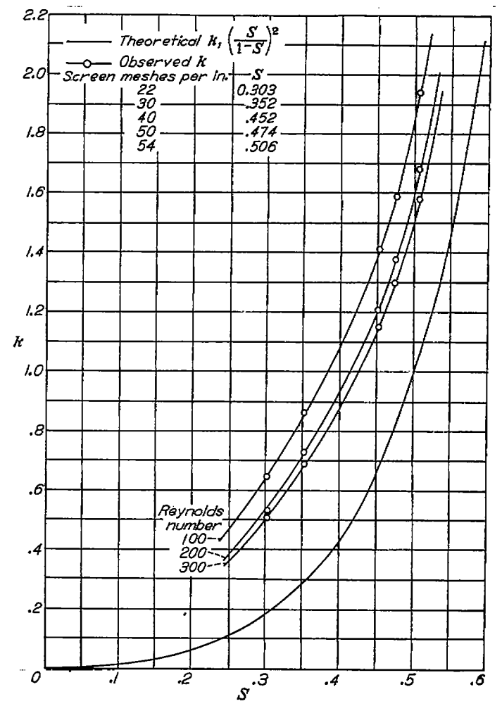
FIGURE 5.—Variation of pressure-drop coefficient with solidity for screens at various Reynolds numbers. Curve without points is theoretical curve according to Eckert and Pflüger (reference 3).
