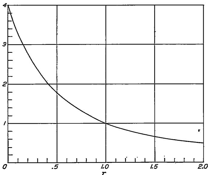
FIGURE 3.—Compressive-buckling coefficients for infinitely long solid-core sandwich plates stressed in the elastic range. k = \frac{4}{(1+r)^2} for r \leq 1 ; k = \frac{1}{r} for r \geq 1 .
