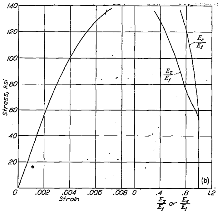
(b) Typical stress-strain relations for stainless steel. FIGURE 6.—Concluded.
