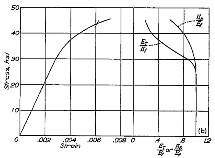
(b) Typical stress-strain relations for 24S-T3 aluminum alloy. FIGURE 4.—Concluded.
