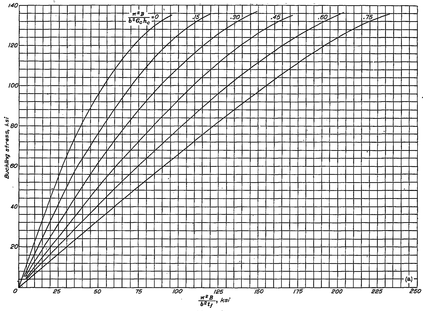
FIGURE 6.—Charts for long solid-core sandwich plates with stainless-steel faces. \mu_f = \frac{1}{3} .
