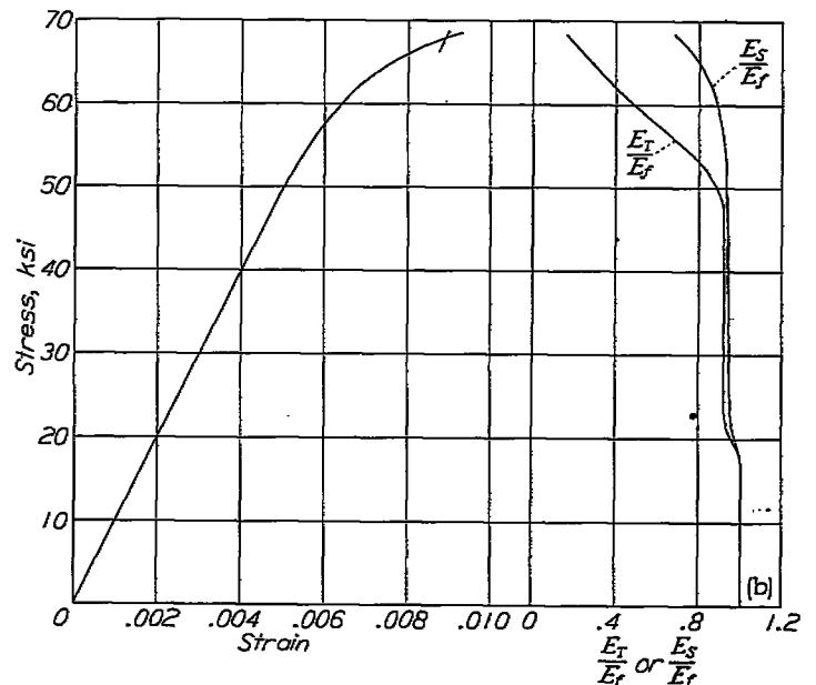
(b) Typical stress-strain relations for 75S-T6 Alclad aluminum alloy.
