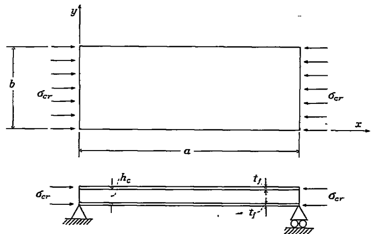
FIGURE 1.—Simply supported solid-core sandwich plate under compression.
