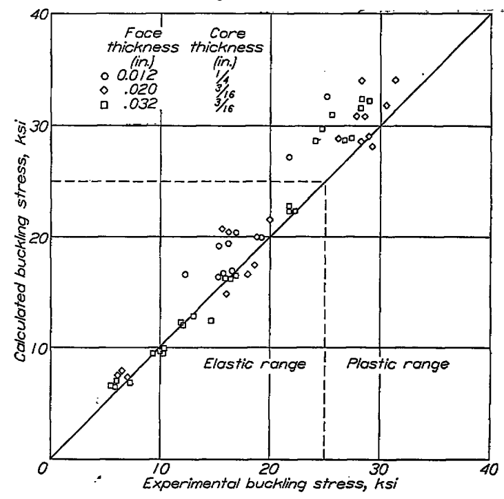
FIGURE 7.—Comparison of calculated and experimental buckling stresses for square solid-core sandwich plates with 24S-T Alclad aluminum-alloy faces.
