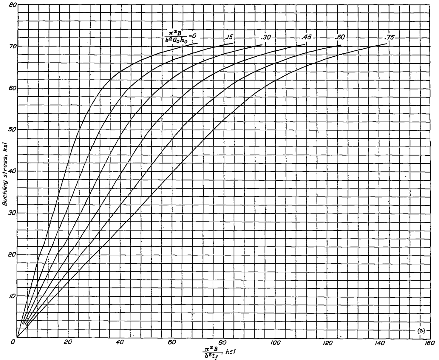
FIGURE 5.—Charts for long solid-core sandwich plates with 75S-T6 Alclad aluminum-alloy faces; \nu_f = \frac{1}{8} .
