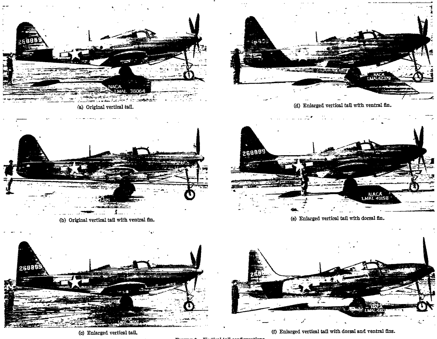
FIGURE 6.—Vertical-tail configurations.
