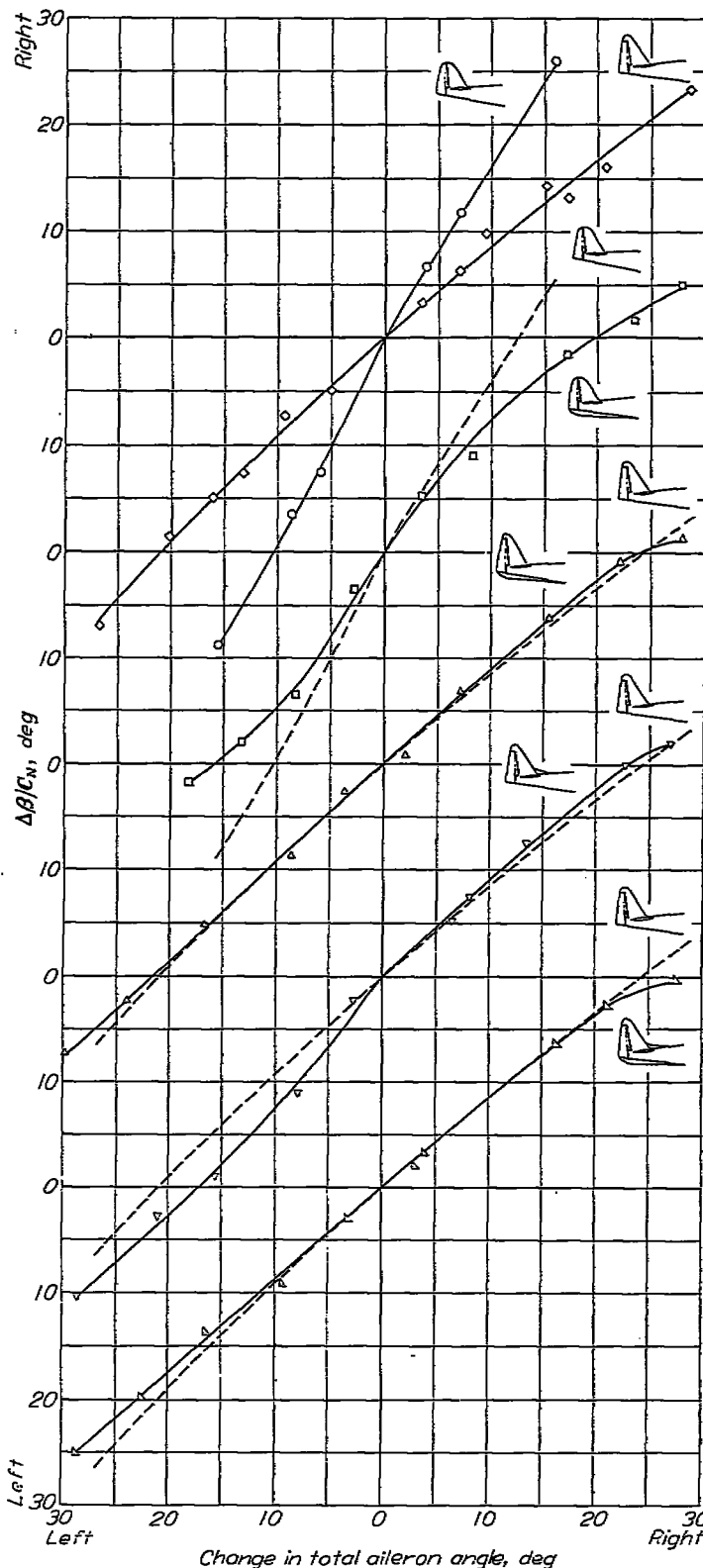
FIGURE 14.—Effect of various vertical-tail modifications on the ability to restrict yaw due to ailerons in rudder-fixed rolls out of turns at 125 to 130 miles per hour with engine idling. Ratio \frac{\Delta\beta}{C_N} is maximum change in sideslip angle per unit airplane normal-force coefficient.
