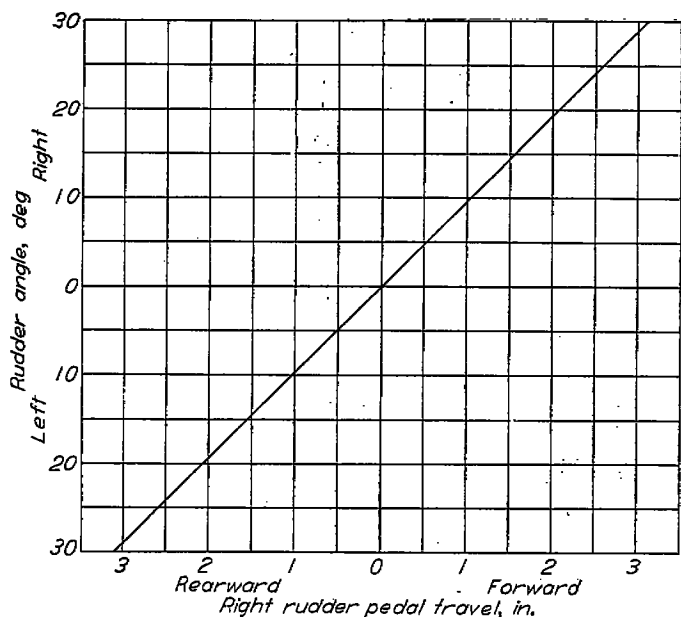
FIGURE 7.—Variation of rudder angle with position of right rudder pedal. Rudder-pedal moment arm 10\frac{3}{4} inches. Pedal travel measured along arc.
