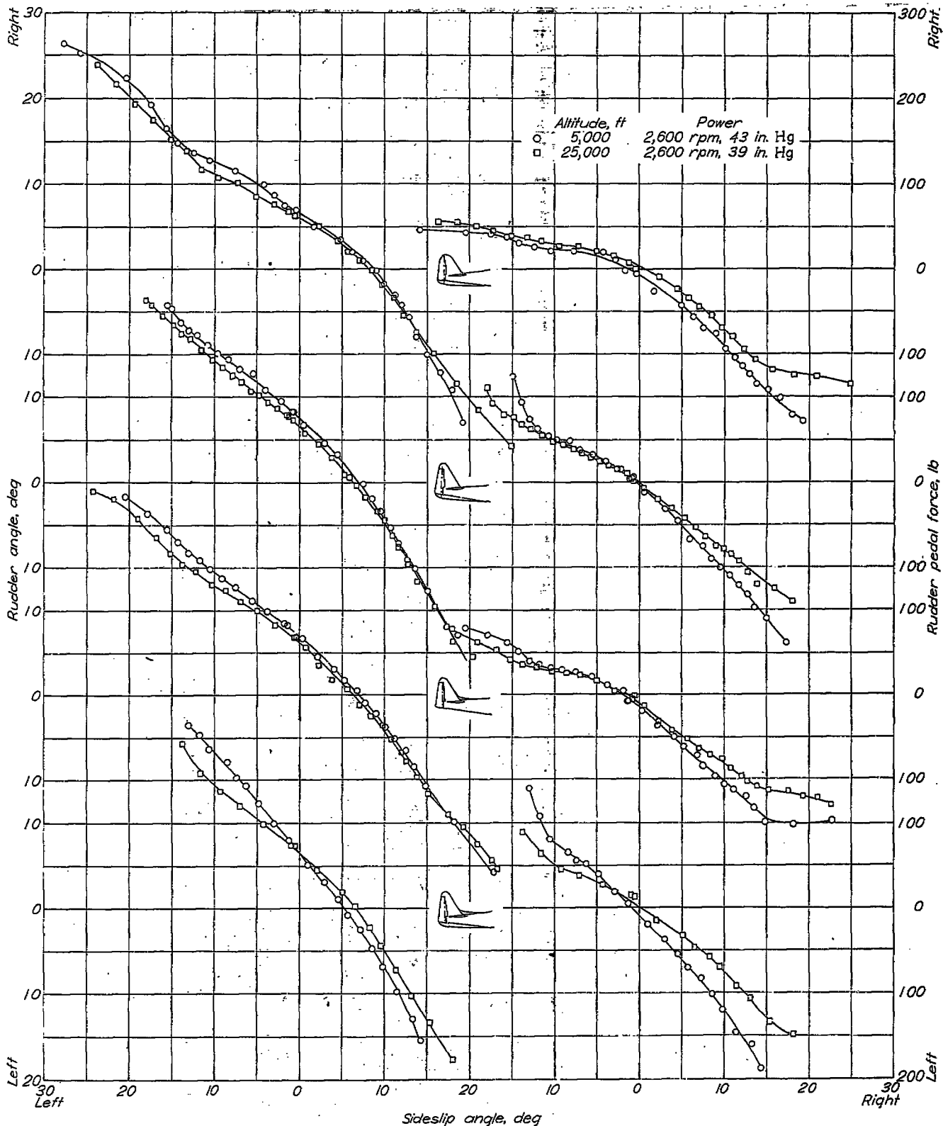
FIGURE 13.—Effect of altitude on the directional characteristics in sideslips at 150 miles per hour. Normal rated power.
