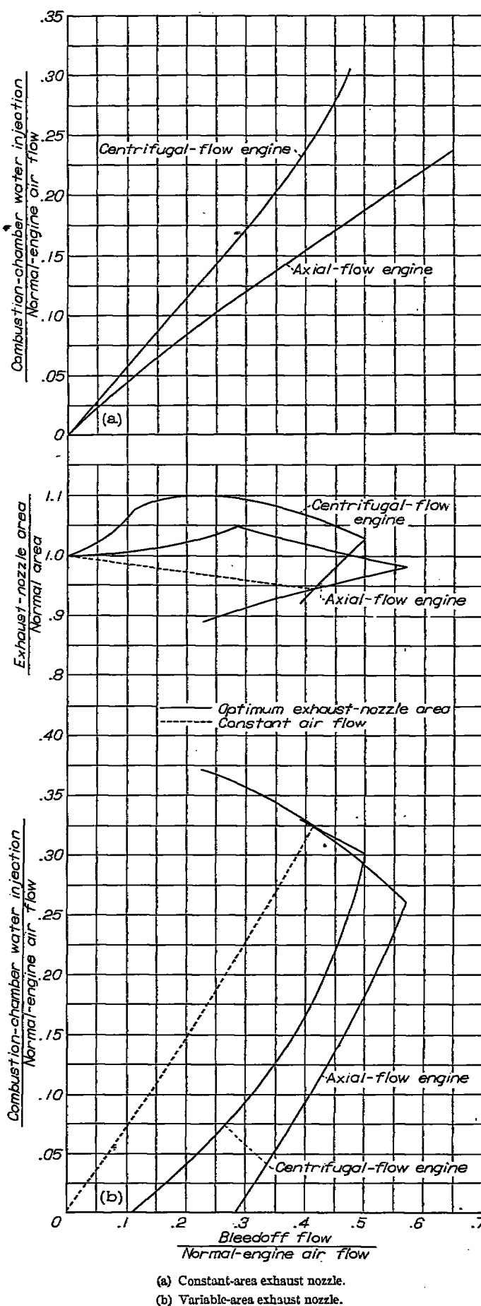
FIGURE 17.—Variation of water-injection rate into primary-engine combustion chambers with bleedoff flow. Flight Mach number, 0; altitude, sea level.
