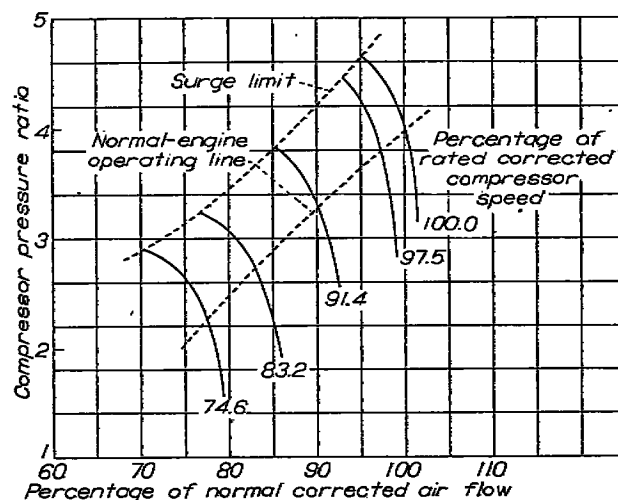
FIGURE 12.—Compressor characteristics assumed for analysis of thrust augmentation by water injection into engine combustion chambers.
