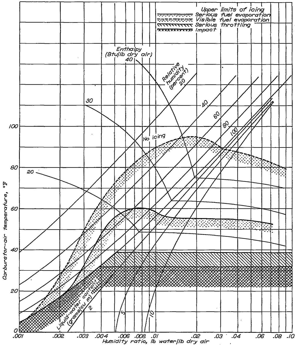
FIGURE 13.—Representative limits of visible and serious icing in engine induction system. Carburator-deck pressure, 23.86 inches mercury absolute.
