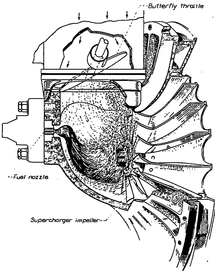
FIGURE 5.—Eddying fuel spray in system utilizing butterfly-type throttles and wall-mounted fuel nozzle.
