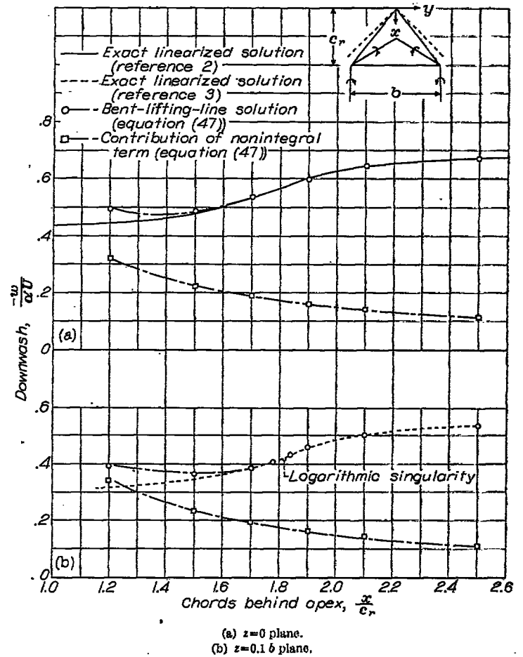
FIGURE 12.—Downwash in y=0 plane behind triangular wing with aspect ratio 2b/c_r of 3.2 using bent lifting line. M=\sqrt{2} .
