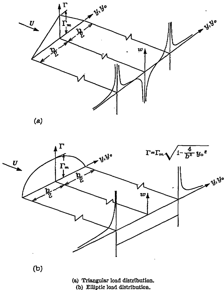
FIGURE 5.—Upwash in z=0 plane an infinite distance behind wings of triangular and elliptic loading.
