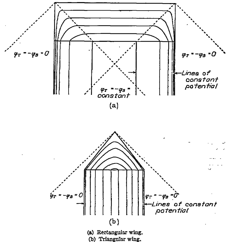
FIGURE 4.—Lines of constant potential for rectangular and triangular wings.
