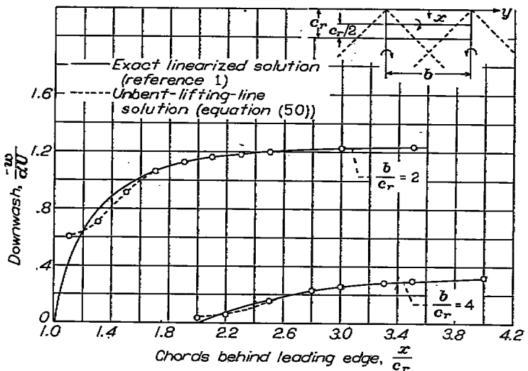
FIGURE 14.—Downwash along line y=0, z=0 behind rectangular wing using unbent (horseshoe) lifting line at \frac{1}{2} -chord point. M=\sqrt{2} .
