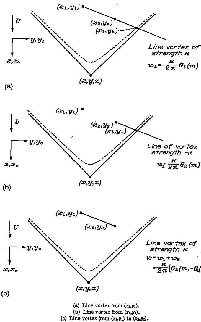
FIGURE 2.—Superposition for obtaining upwash induced by line-vortex segment from (x_1, y_1) to (x_2, y_2) .
