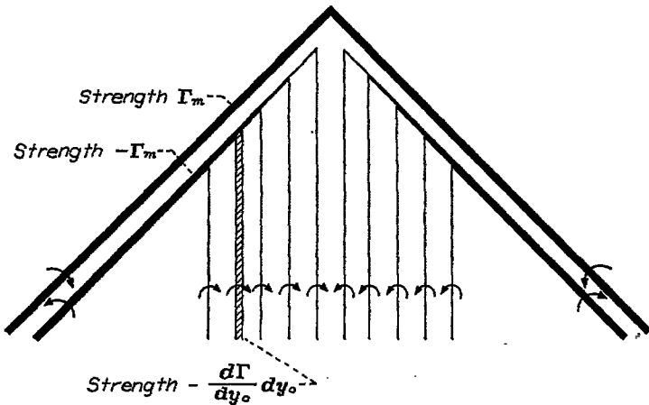
FIGURE 9.—Superposition of bent line vortices yielding bent-lifting-line representation of supersonic wing (equation (41)).
