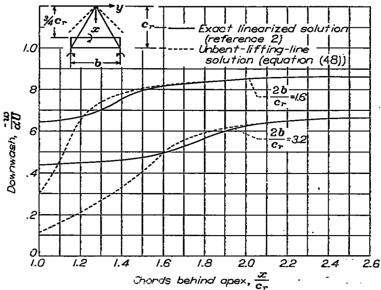
FIGURE 13.—Downwash along line y=0, z=0 behind triangular wing using unbent (horseshoe) lifting line at \frac{1}{4} -chord point. M=\sqrt{2} .
