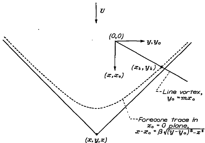
FIGURE 1.—Geometric relations for determination of upwash induced by line vortex.
