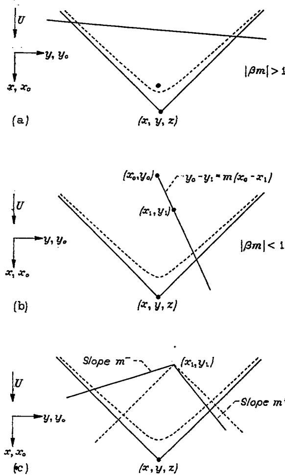
(a) Infinite line vortex inclined supersonically to free stream. (b) Infinite line vortex inclined subsonically to free stream. (c) Bent line vortex.
