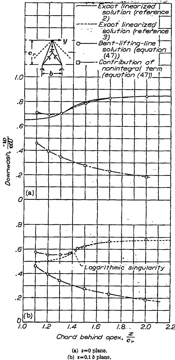
FIGURE 11.—Downwash in y=0 plane behind triangular wing with aspect ratio 2b/c_r of 1.6 using bent lifting line. M=\sqrt{2} .
