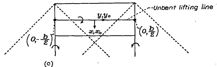
(a) Bent-lifting-line representation of triangular wing. (b) Unbent-lifting-line representation of triangular wing. (c) Unbent-lifting-line representation of rectangular wing.
