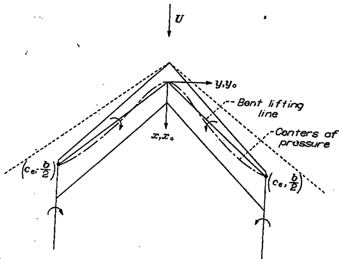
FIGURE 7.—Bent-lifting-line approximation for sweptback wing.
