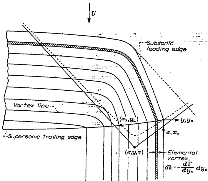
FIGURE 6.—Wing tip formed by intersection of subsonic leading and supersonic trailing plan-form edges.
