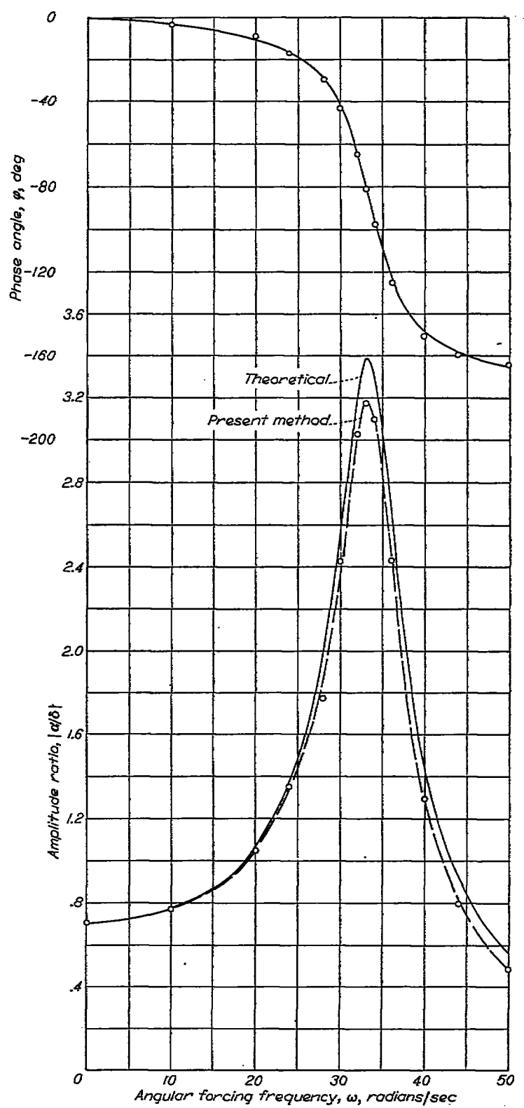
FIGURE 5.—Comparison of the theoretical response and the computed response determined from the computed frequency responses of figure 4.
