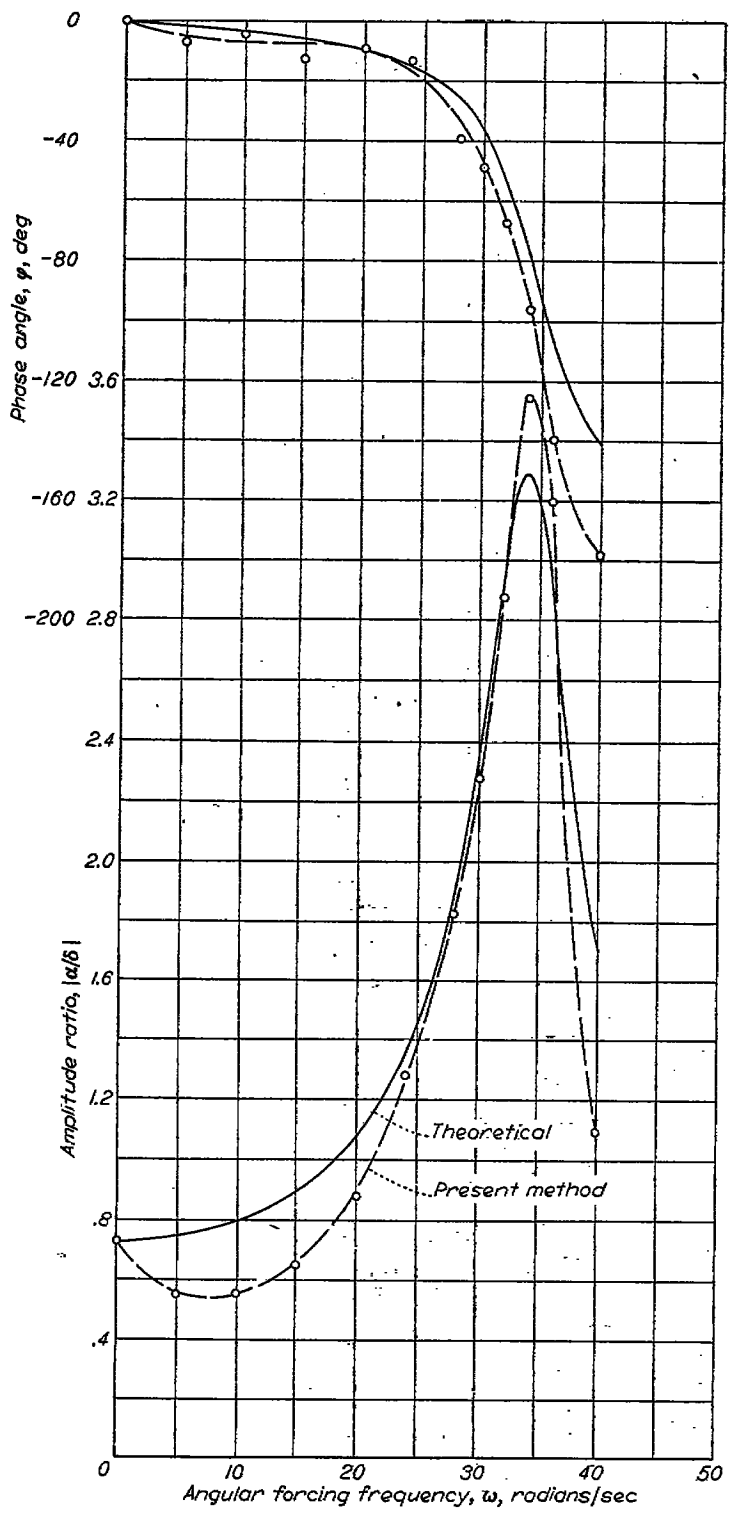
FIGURE 9.—Comparison of theoretical and computed aircraft angle-of-attack frequency responses as determined from flight-test data.
