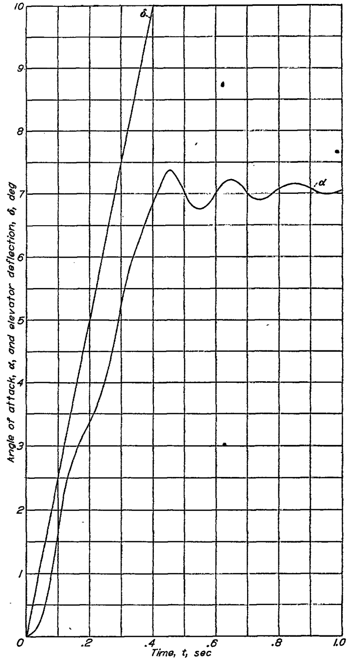
FIGURE 6.—The input \delta and output \alpha transients for the ramp-function-input example.
