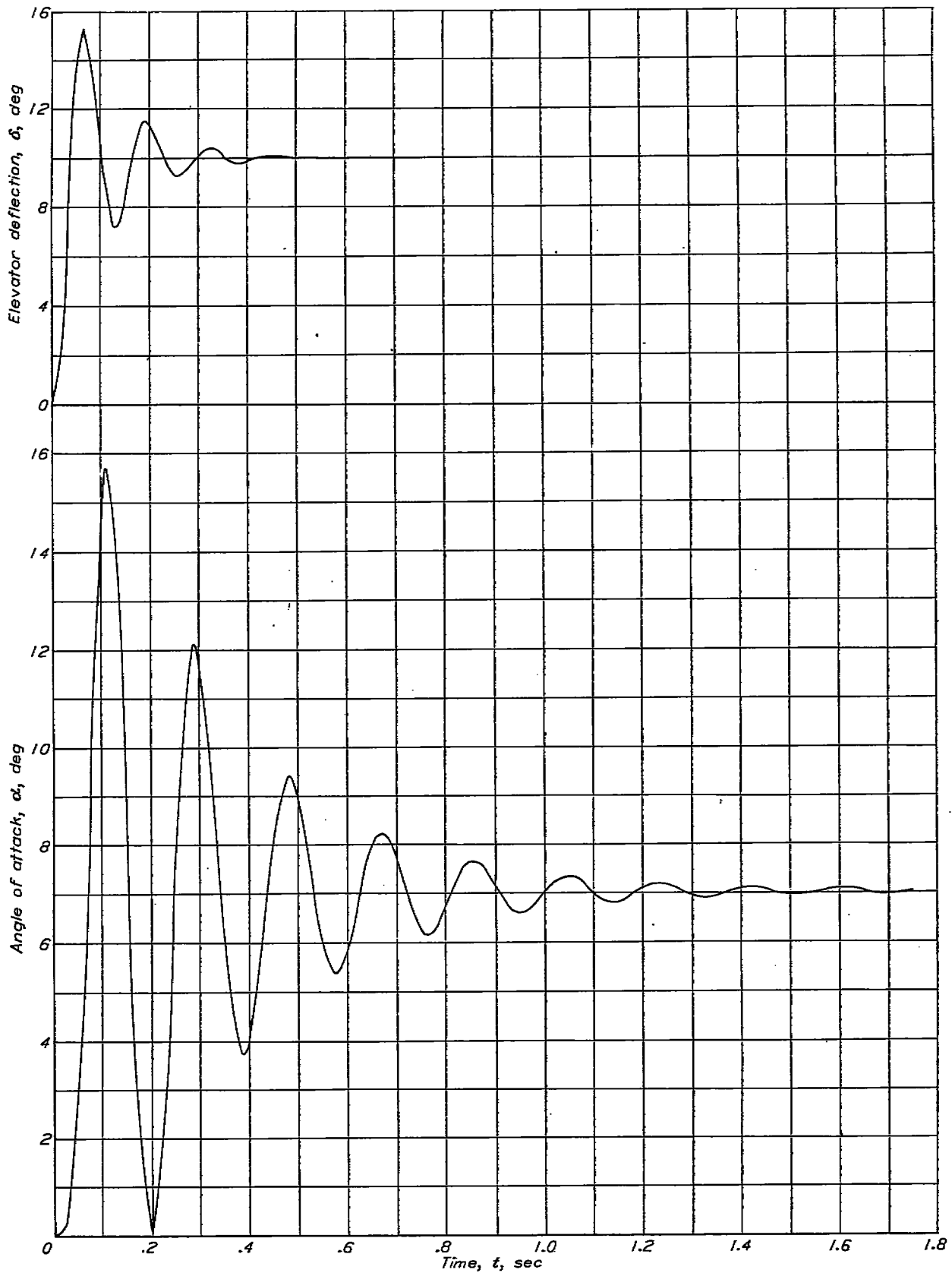
FIGURE 3.—Calculated input \delta and output \alpha' transients.
