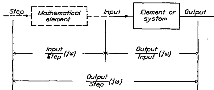
FIGURE 2.—Block diagram showing method for determining frequency response when input is arbitrary.
