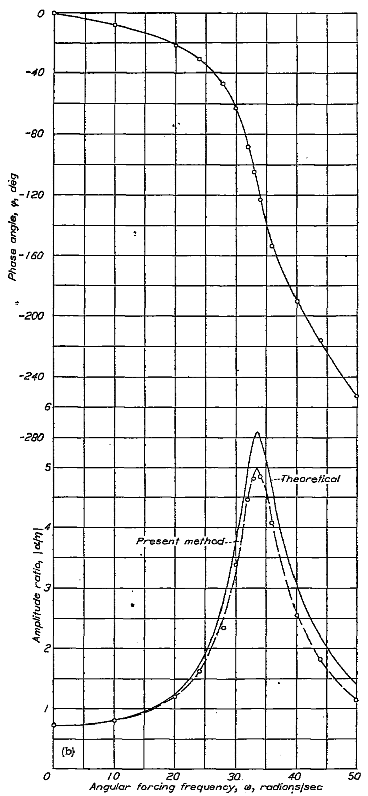
(b) Over-all frequency response, a/\eta . FIGURE 4.—Concluded.
