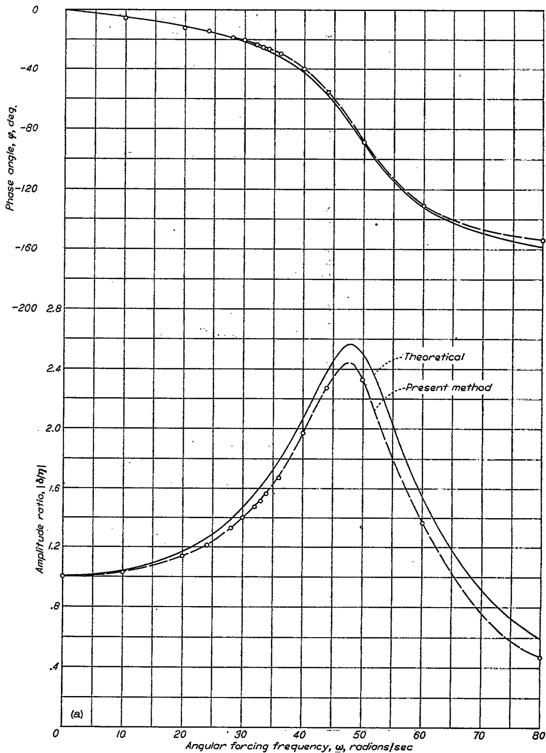
(a) One-degree-of-freedom frequency response, \delta/\eta . FIGURE 4.—Comparison of theoretical frequency responses and computed frequency responses determined from the transients of figure 3.
