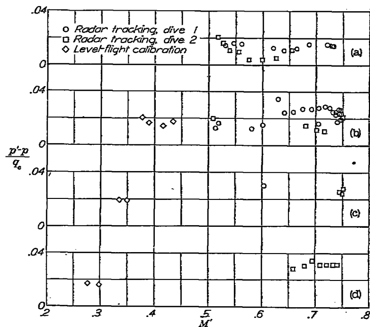
(a) Lift coefficient from 0.03 to 0.10. (b) Lift coefficient from 0.10 to 0.20. (c) Lift coefficient from 0.20 to 0.30. (d) Lift coefficient from 0.30 to 0.40.
