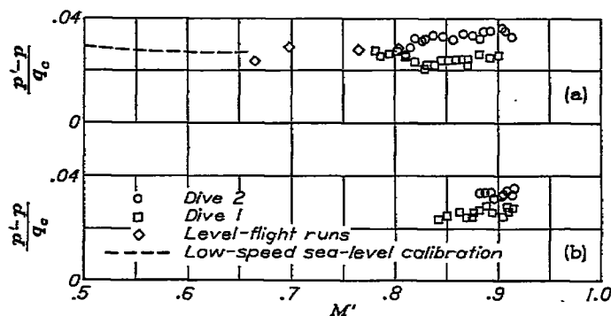
(a) Lift coefficient from 0 to 0.1. (b) Lift coefficient from 0.1 to 0.2.
