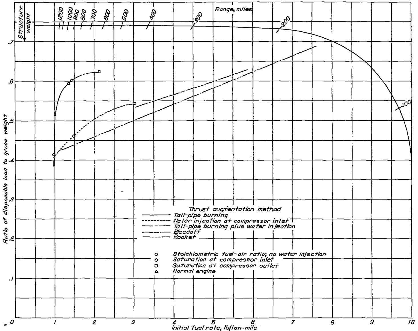
FIGURE 8.—Load-range characteristics of airplane powered by augmented turbojet engines. Altitude, 35,332 feet; flight Mach number, 1.50.
