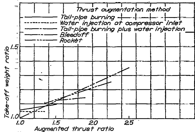
FIGURE 7.—Variation at take-off of the ratio of weight of engine plus augmentation equipment plus fuel and liquid to the weight of normal engine plus fuel with augmented thrust ratio.
