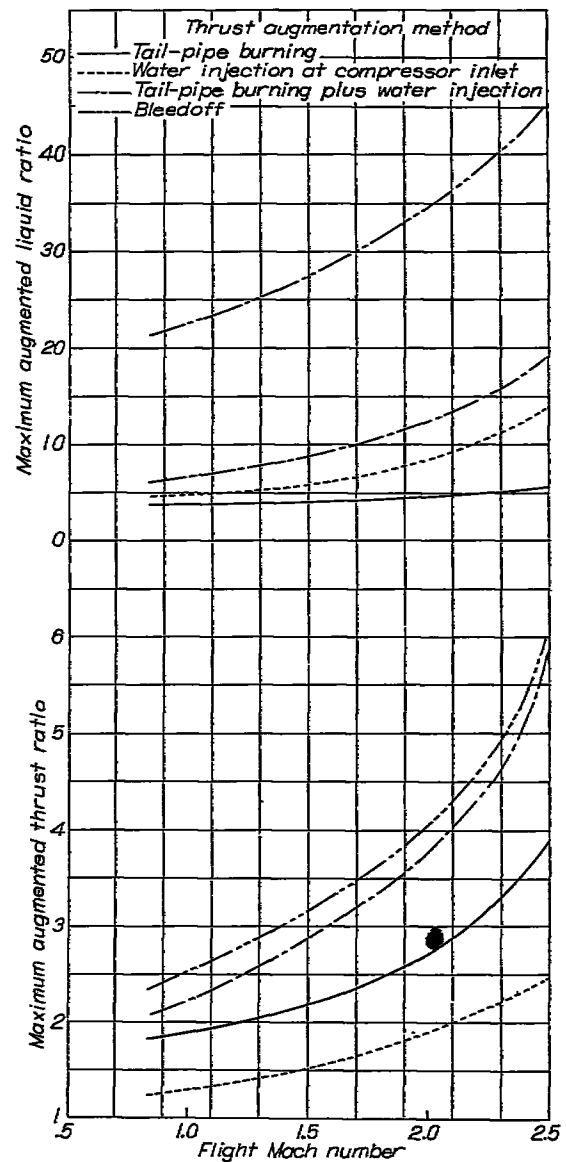
FIGURE 5.—Maximum augmented thrust and maximum augmented liquid ratios as functions of flight Mach number for altitude of 35,332 feet.
