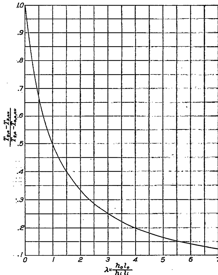
FIGURE 5.—Chart for calculation of spanwise temperature distribution through air-cooled turbine blade for average cooling-air temperature.
