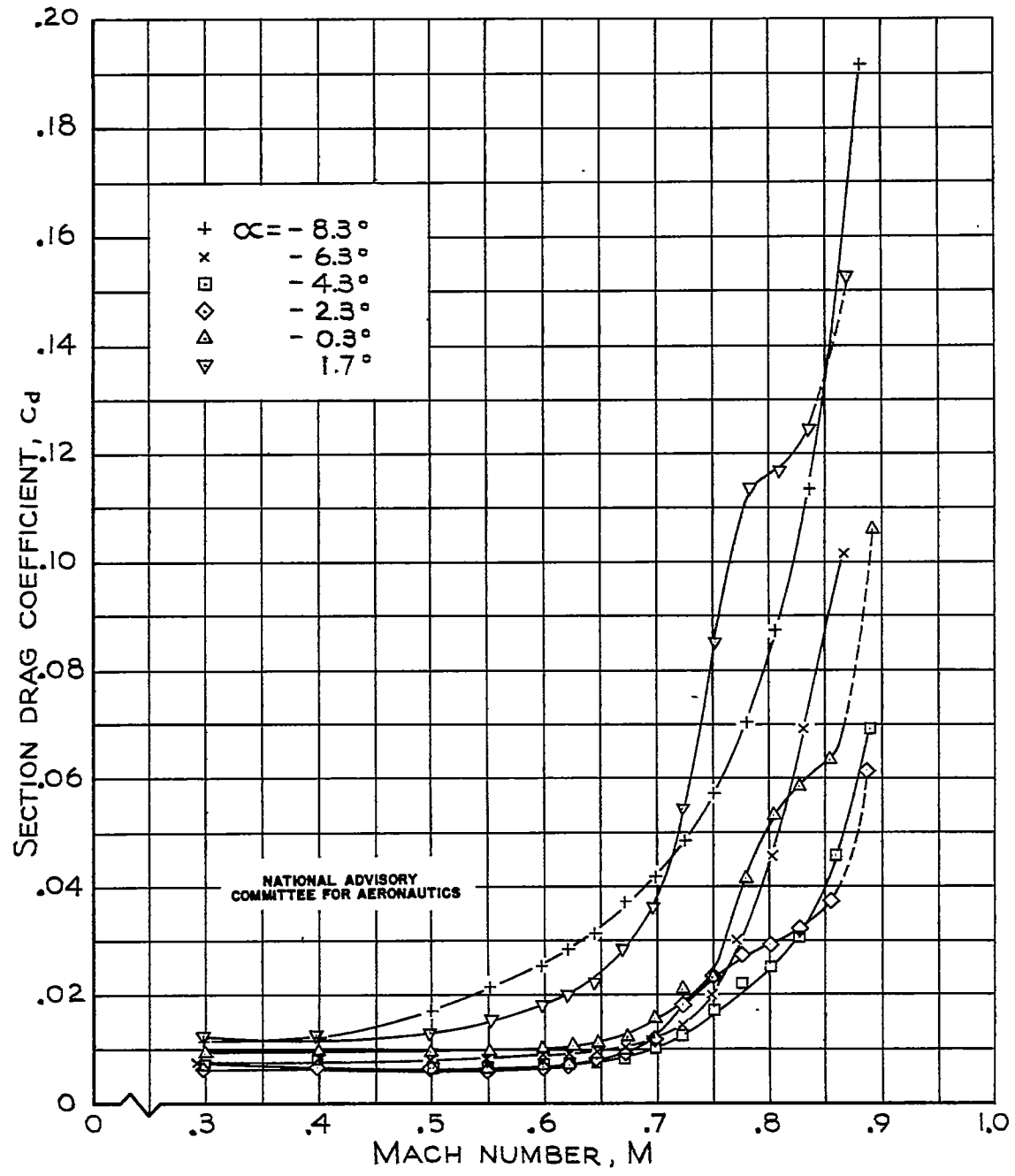
(b) \delta_f = 10.2^\circ FIGURE 7.-CONCLUDED. NACA 0006 AIRFOIL WITH 35-PERCENT-CHORD PLAIN FLAP.
