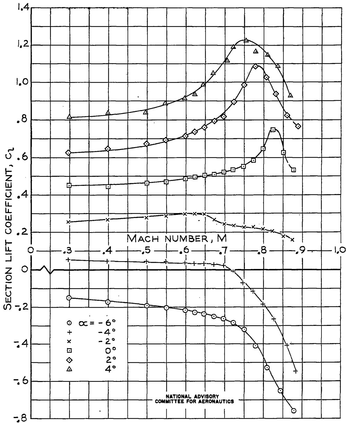
(b) \delta_f = 10.5^\circ FIGURE 3.- CONCLUDED. NACA 0006 AIRFOIL WITH 15-PERCENT-CHORD PLAIN FLAP.
