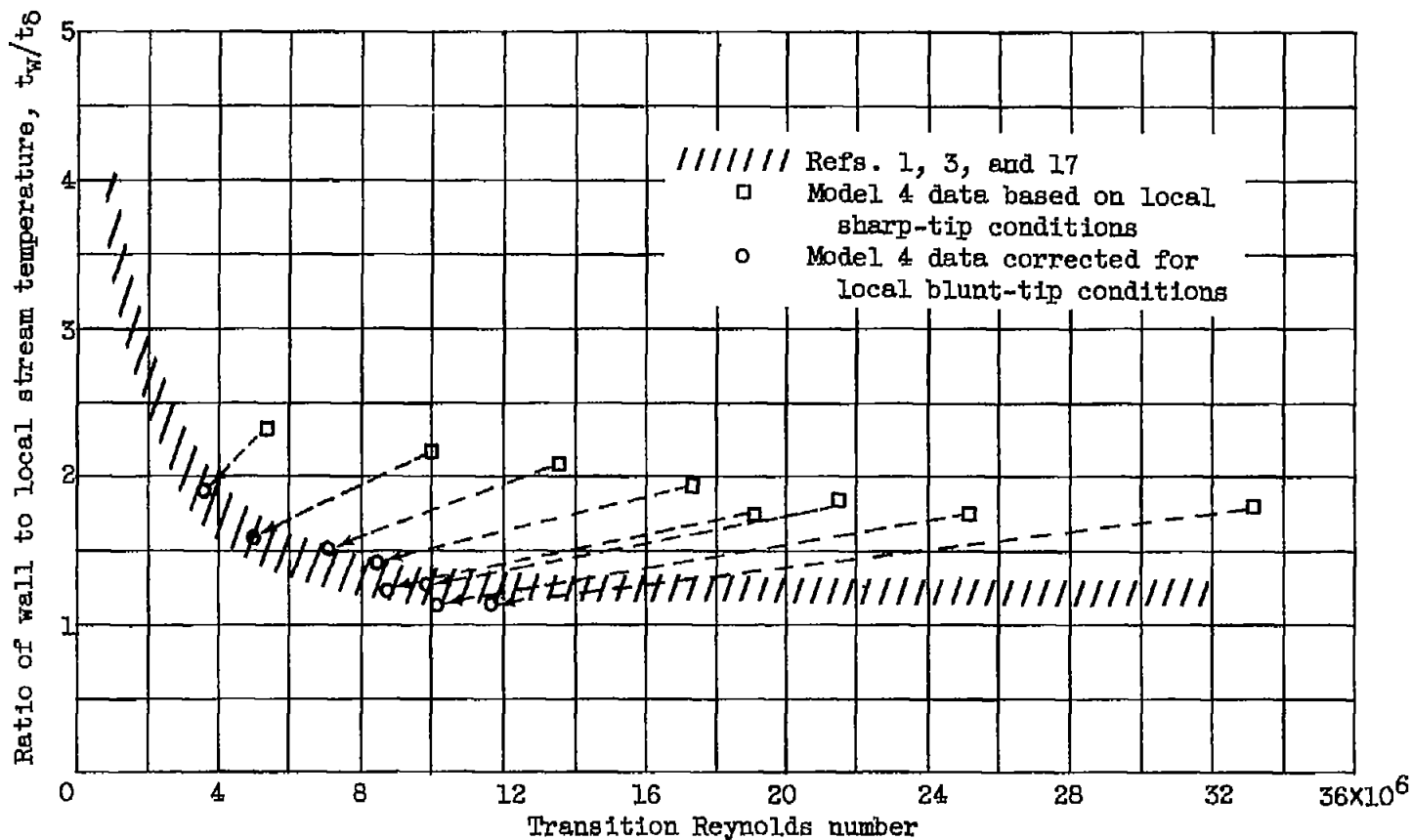
Figure 10. - Comparison of transition Reynolds numbers and local temperature ratios of model 4 (2-micron. average roughness) with data from other investigations.
