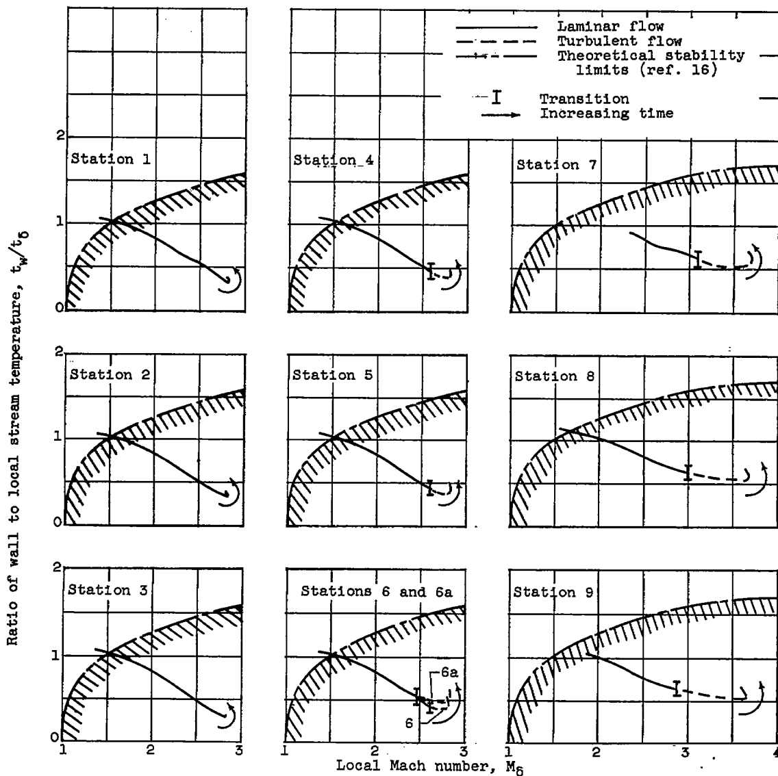
Figure 11. - Variation of local temperature ratio with local Mach number for model 3 (50-micron. average roughness).
