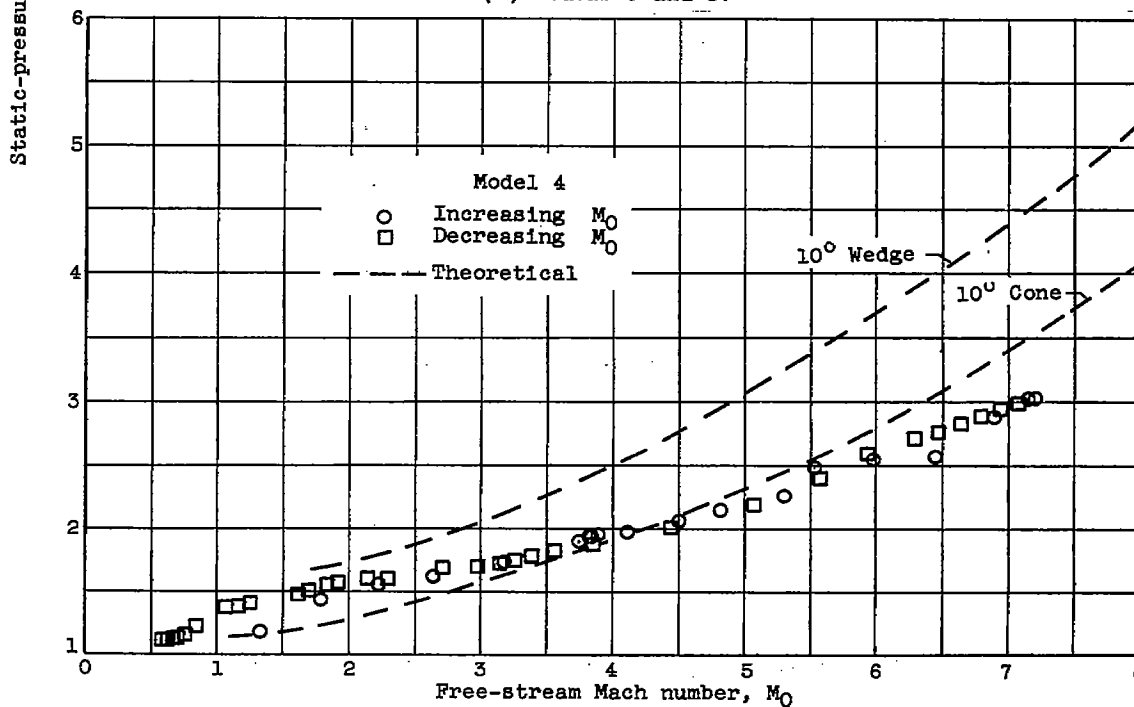
(b) Model 4.
