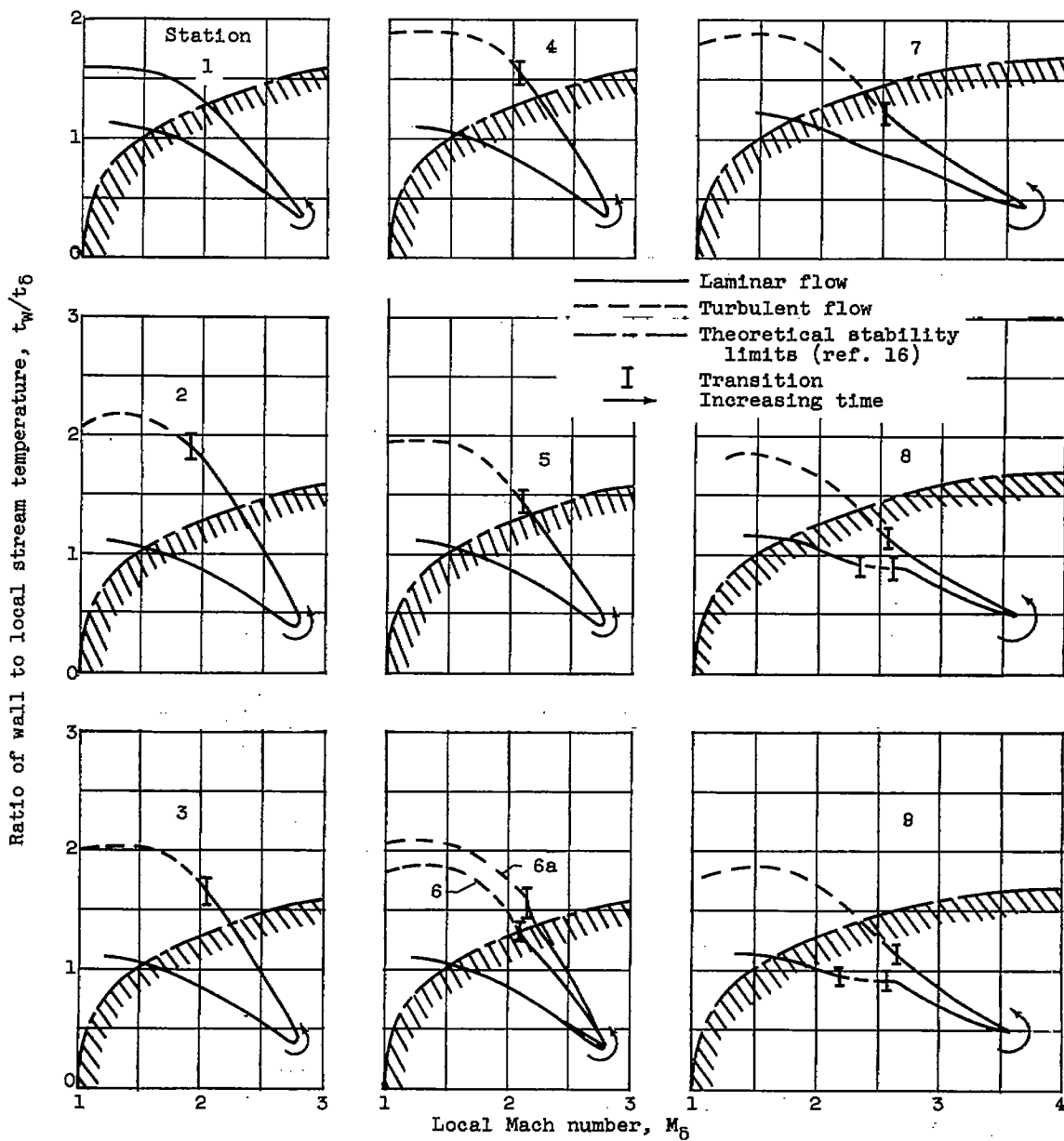
Figure 8. - Variation of local temperature ratio with local Mach number for model 4 (2-microin. average roughness).
