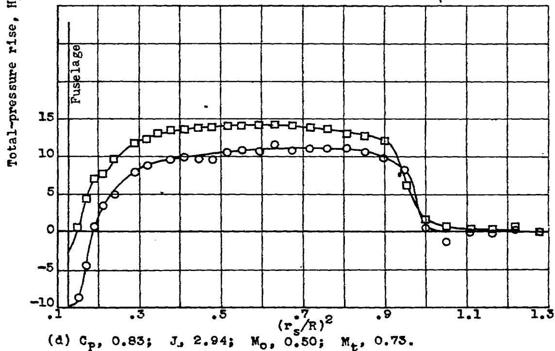
Figure 11.- Continued. Effect of power coefficient C_p on blade thrust load distribution at advance-diameter ratio J of approximately 2.90 and free-stream Mach number M_o of approximately 0.50. Curtiss 838-1C2-18R1 four-blade propeller.
