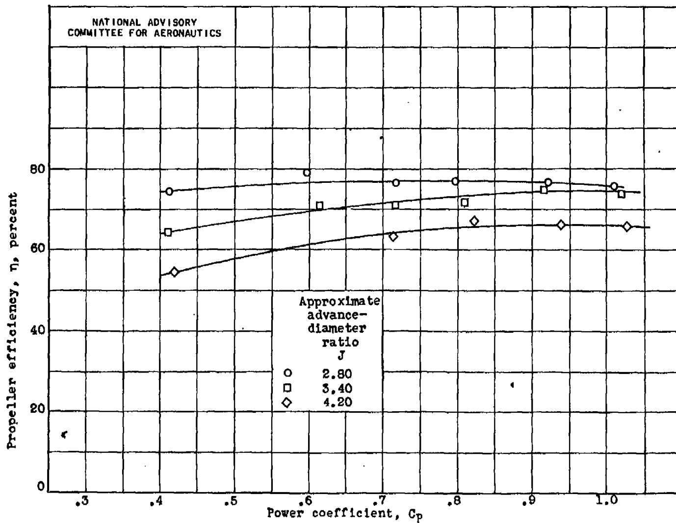
Figure 10.- Effect of power coefficient C_p on propeller efficiency \eta at free-stream Mach number M_0 of approximately 0.50. Curtiss 838-1C2-18R1 four-blade propeller.
