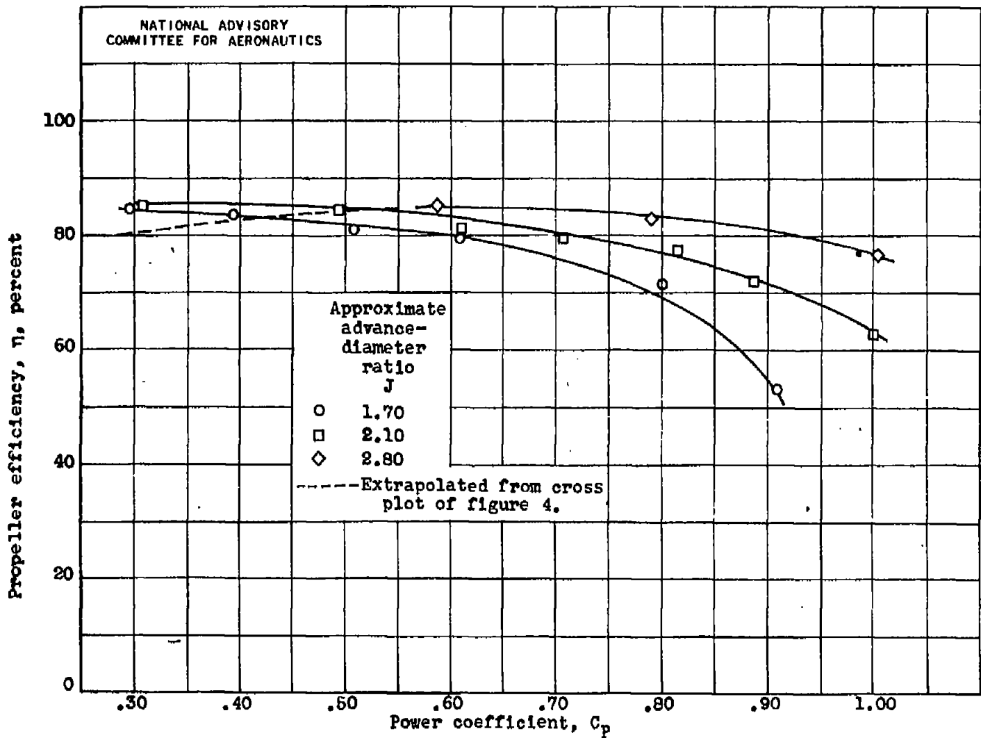
Figure 5.- Effect of power coefficient C_p on propeller efficiency \eta at constant advance-diameter ratios at free-stream Mach number M_o of approximately 0.40. Curtiss B58-1C2-18R1 four-blade propeller.
