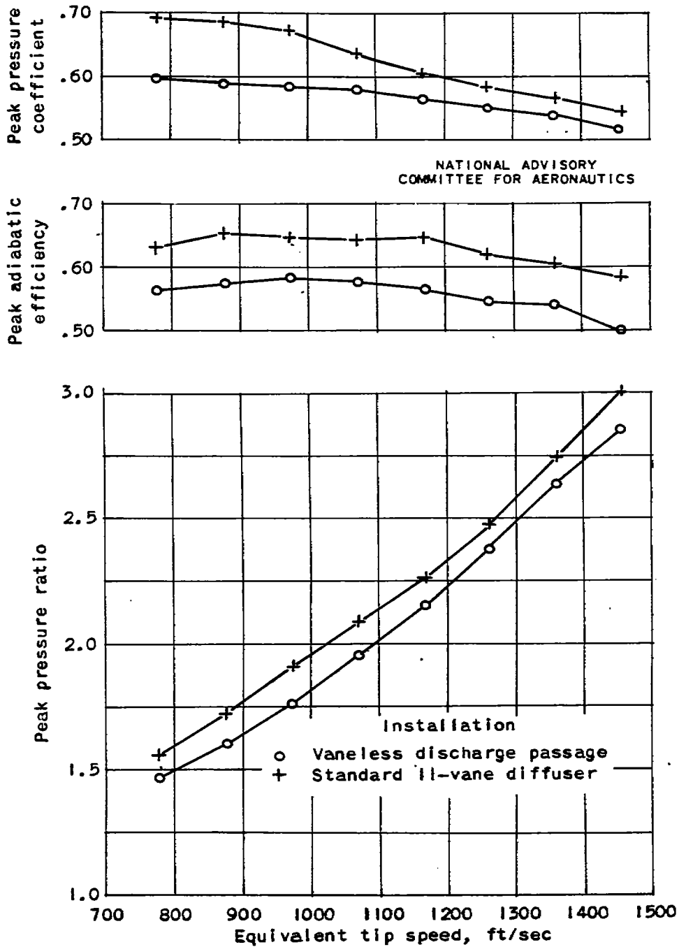
Figure 7. - Peak performance characteristics of auxiliary-stage supercharger with carburetor installed for V-1710-93 engine with standard 11-vane diffuser and vaneless discharge passage at various equivalent impeller tip speeds.
