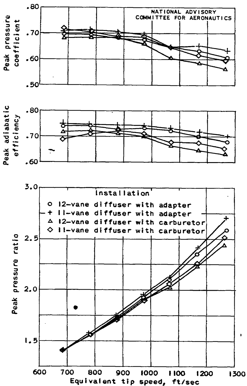
Figure 5. - Peak performance characteristics of auxiliary-stage supercharger for V-1710-93 engine with standard 11-vane diffuser and 12-vane diffuser at various equivalent tip speeds.
