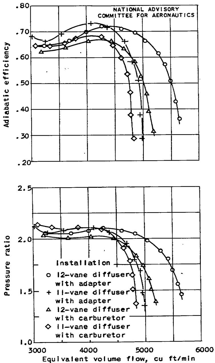
Figure 4. - Typical performance curves of auxiliary-stage supercharger for V-1710-93 engine with standard 11-vane diffuser and 12-vane diffuser at equivalent tip speed of 1073 feet per second.
