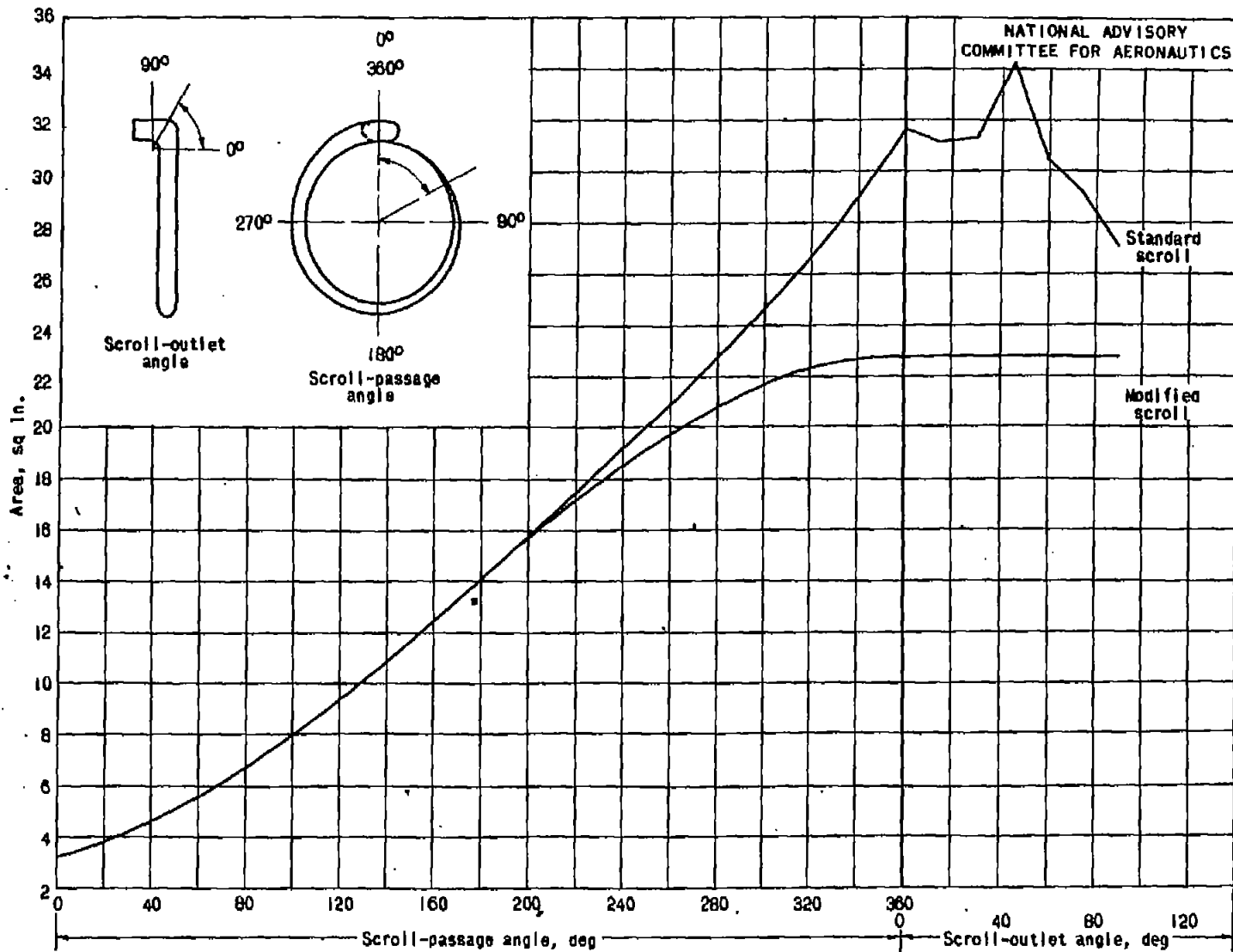
Figure 3. - Variation of area through scroll passage and scroll outlet of auxiliary-stage supercharger for V-1710-93 engine.
