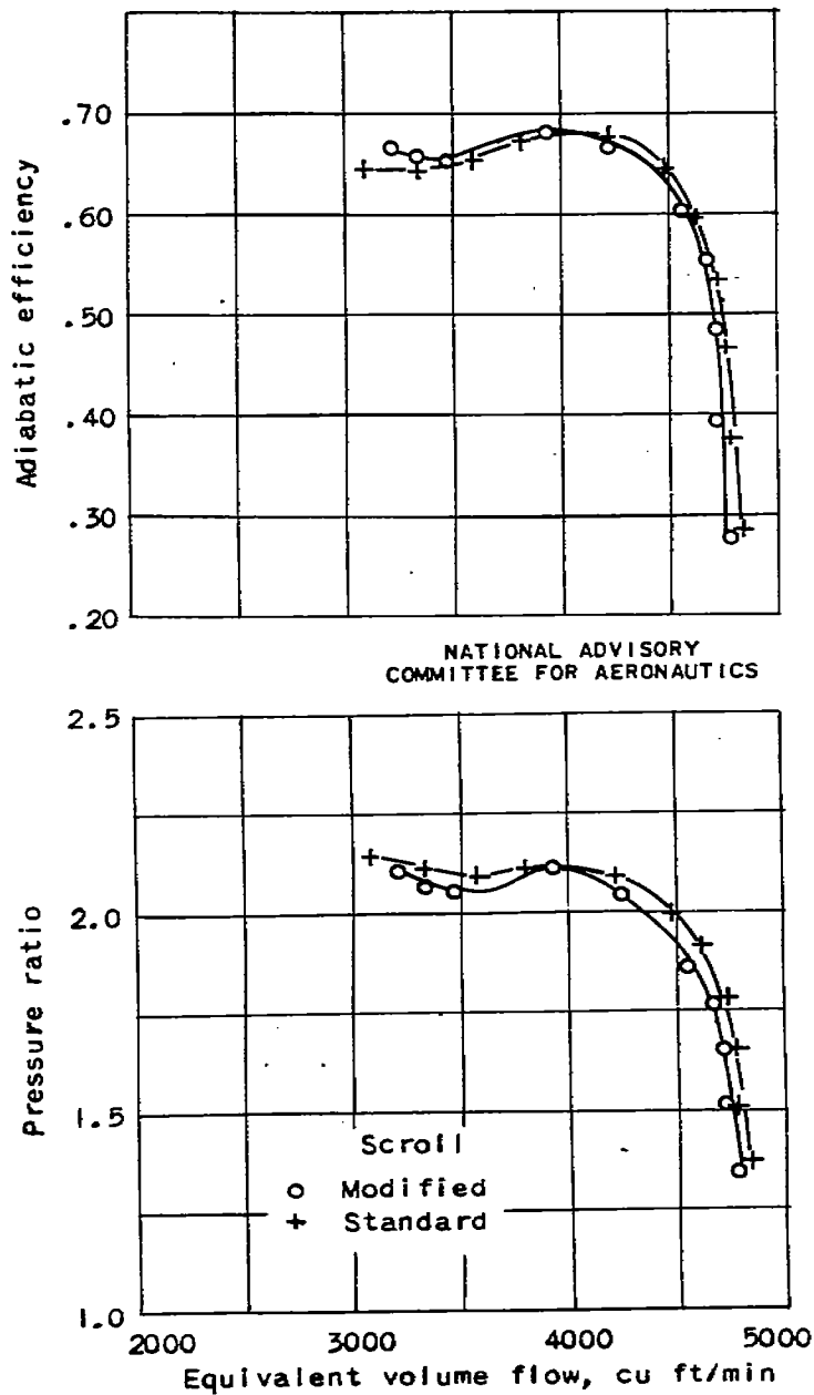
Figure 8. - Typical performance curves of auxiliary-stage supercharger with carburetor installed for V-1710-93 engine with standard and modified scroll at equivalent tip speed of 1073 feet per second.
