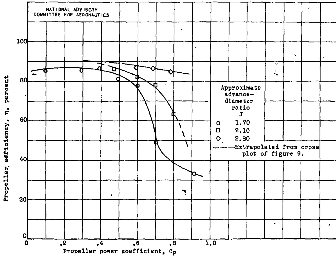
Figure 10.— Effect of power coefficient C_p on propeller efficiency \eta at constant advance-diameter ratio J and free-stream Mach number M_0 of 0.40. Curtiss 836-14C2-1B1 four-blade propeller.
