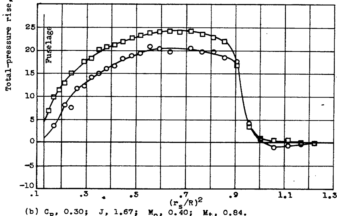
Figure 11.- Effect of power coefficient C_p on blade thrust load distribution at advance-diameter ratio J of approximately 1.70 and free-stream Mach number M_0 of approximately 0.40. Curtiss 836-14C2-18R1 four-blade propeller.
