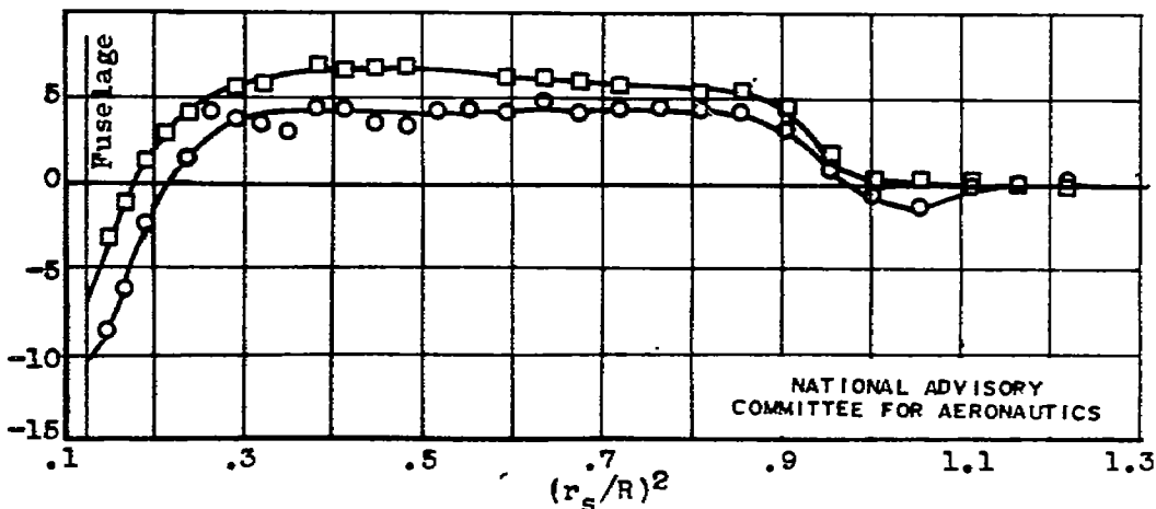
(f) C_p, 1.03 ; J, 4.32 ; M_o, 0.50 ; M_t, 0.62 .
