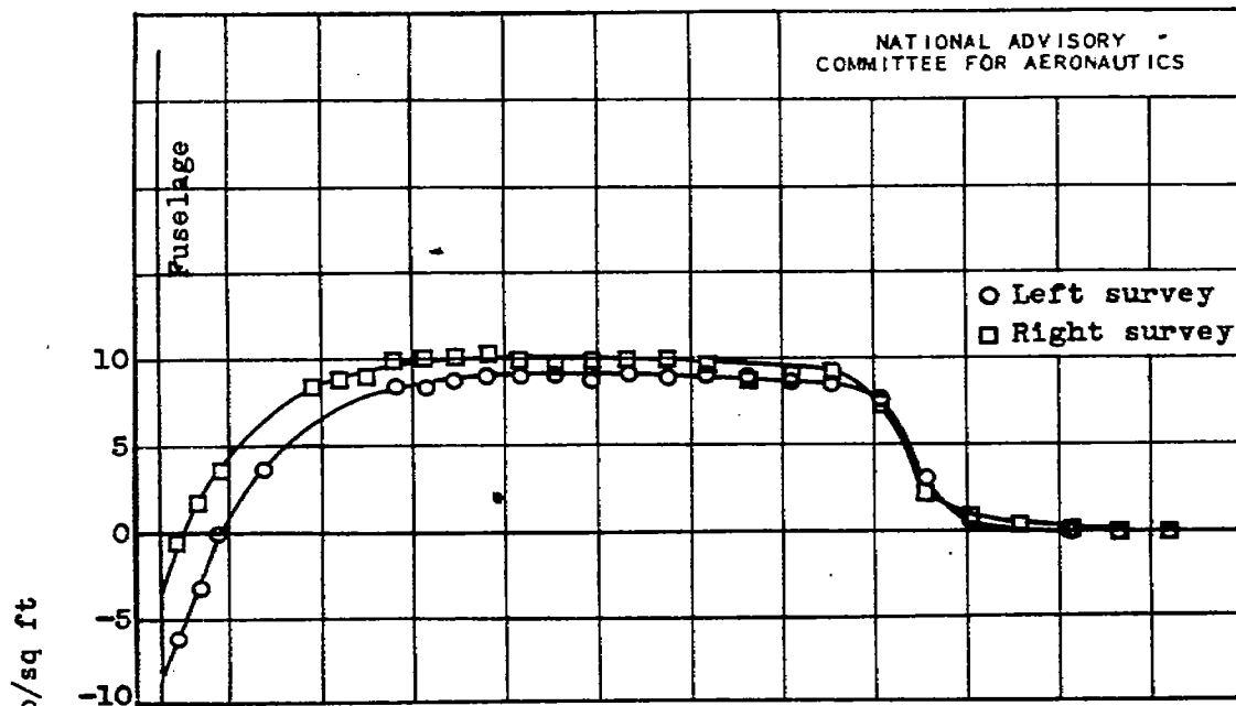
(c) C_p, 1.02 ; J, 3.42 ; M_o, 0.50 ; M_t, 0.68 .
