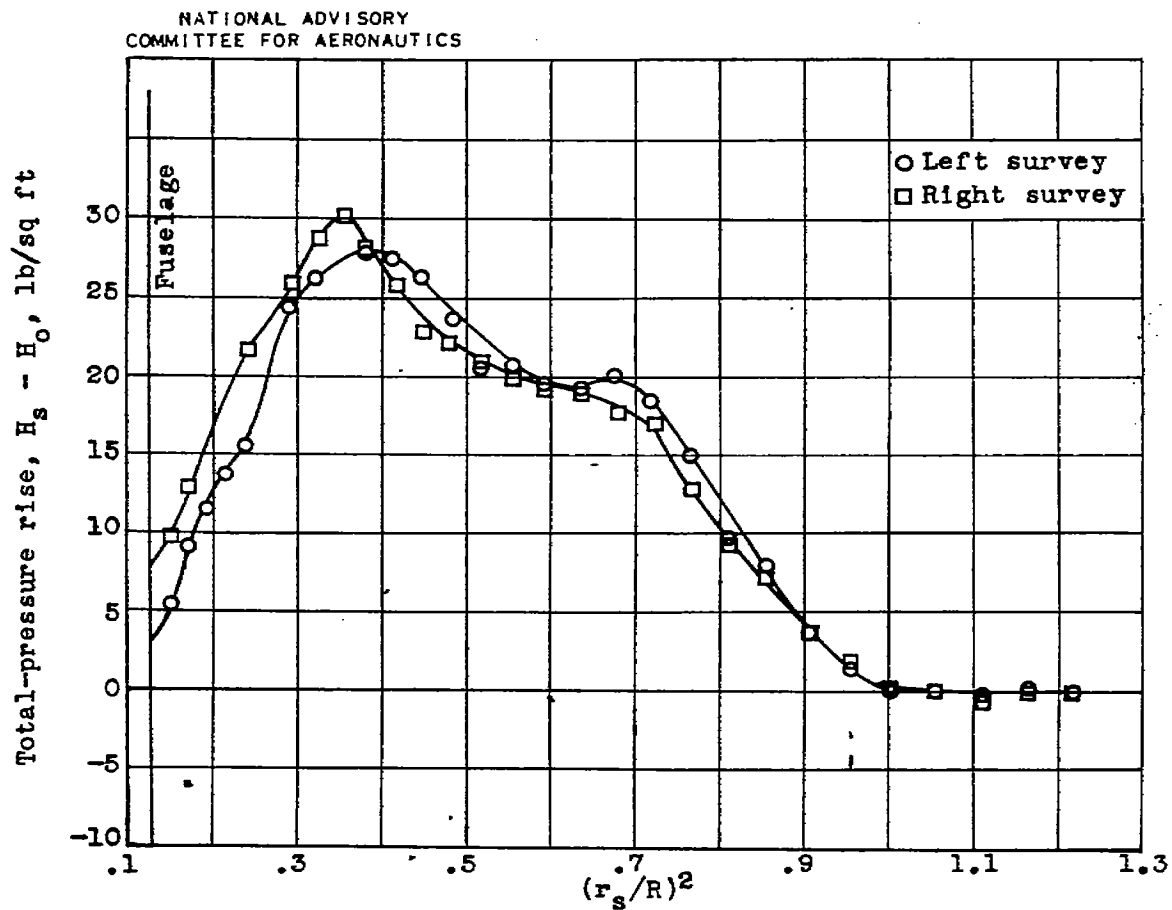
(g) C_p , 0.68; J , 1.11; M_o , 0.28; M_t , 0.85. Figure 6.- Concluded. Effect of power coefficient C_p on blade thrust load distribution at advance-diameter ratio J of approximately 1.00 and free-stream Mach number M_o of approximately 0.30. Curtiss 836-14C2-18R1 four-blade propeller.
