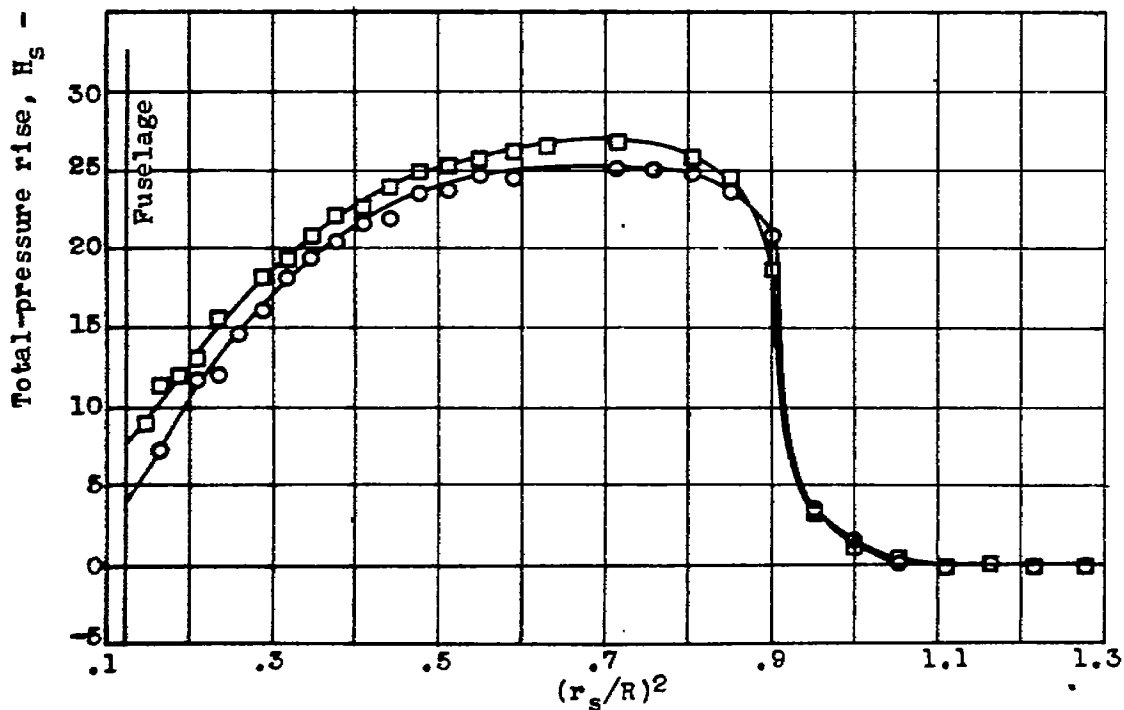
(b) C_p, 0.39 ; J, 1.16 ; M_o, 0.28 ; M_t, 0.82 .
