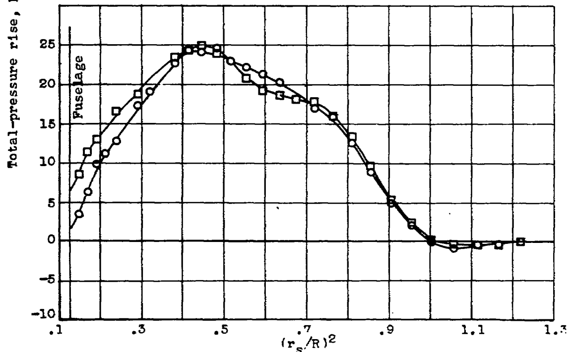
(e) C_p , 0.70; J , 1.50; M_o , 0.38; M_t , 0.89.
