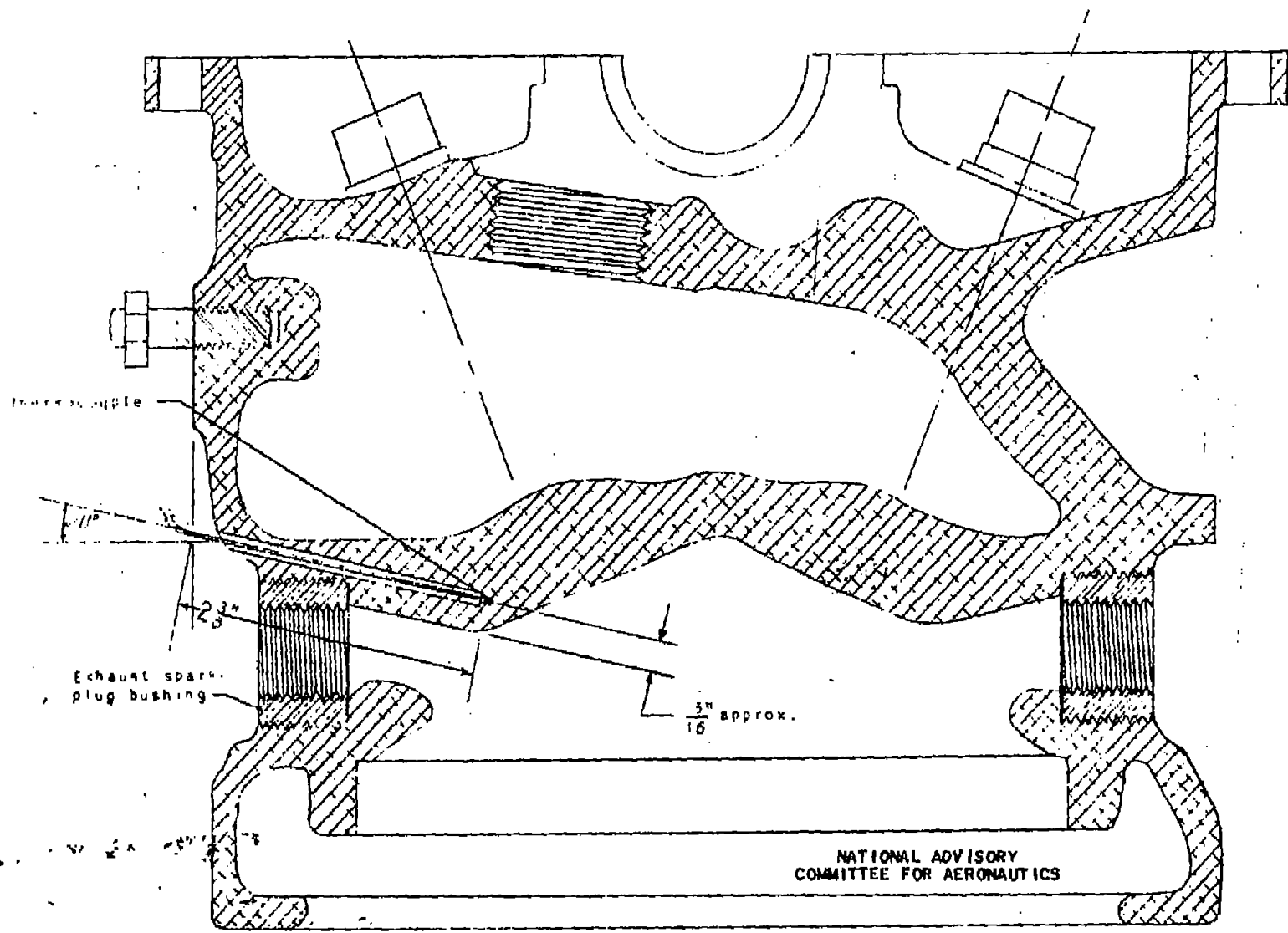
Figure 3. - Section through cylinder head of a v-type, liquid-cooled aircraft engine showing location of cylinder-head thermocouple.
