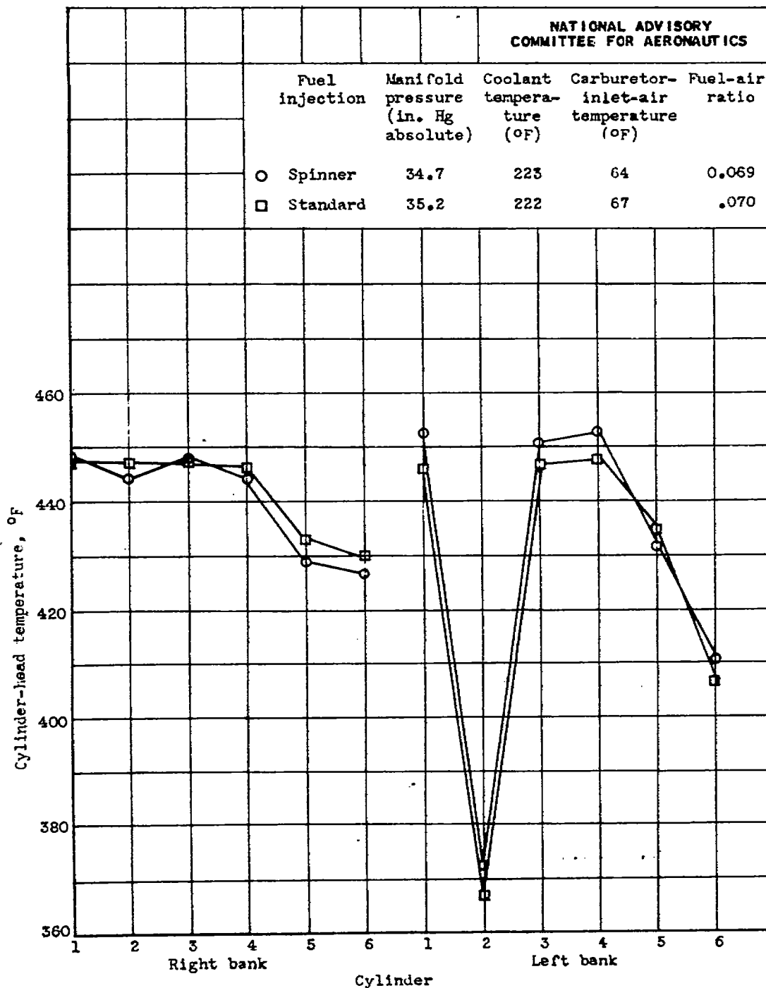
(c) Manifold pressure, 35 inches of mercury absolute.
