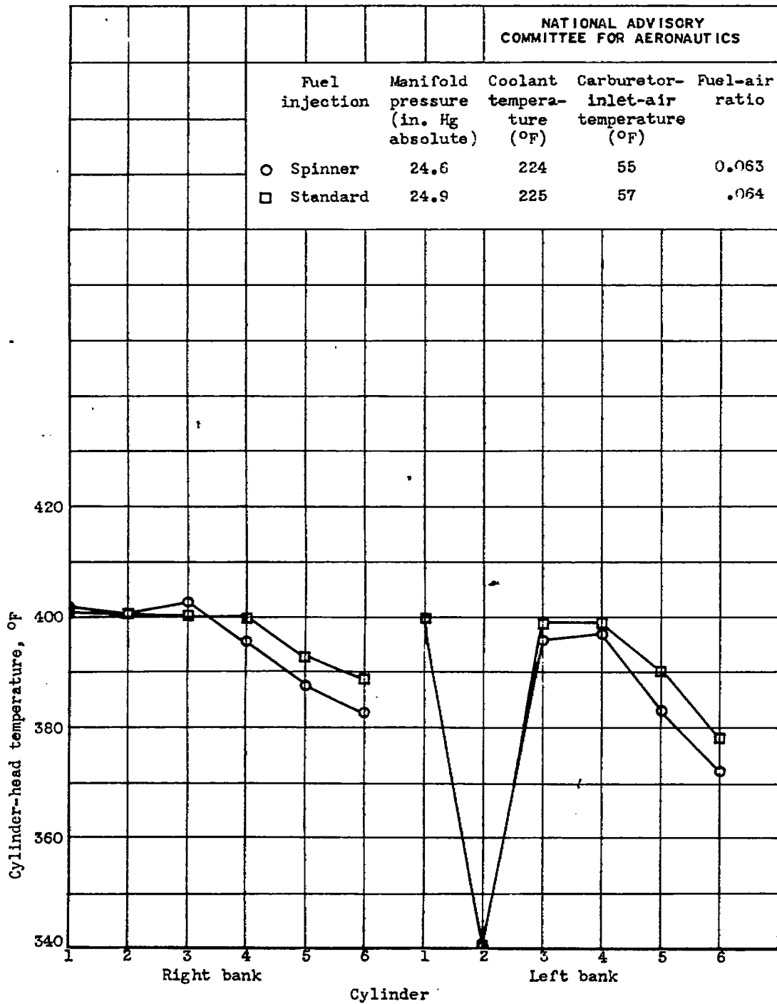
(e) Manifold pressure, 25 inches of mercury absolute.
