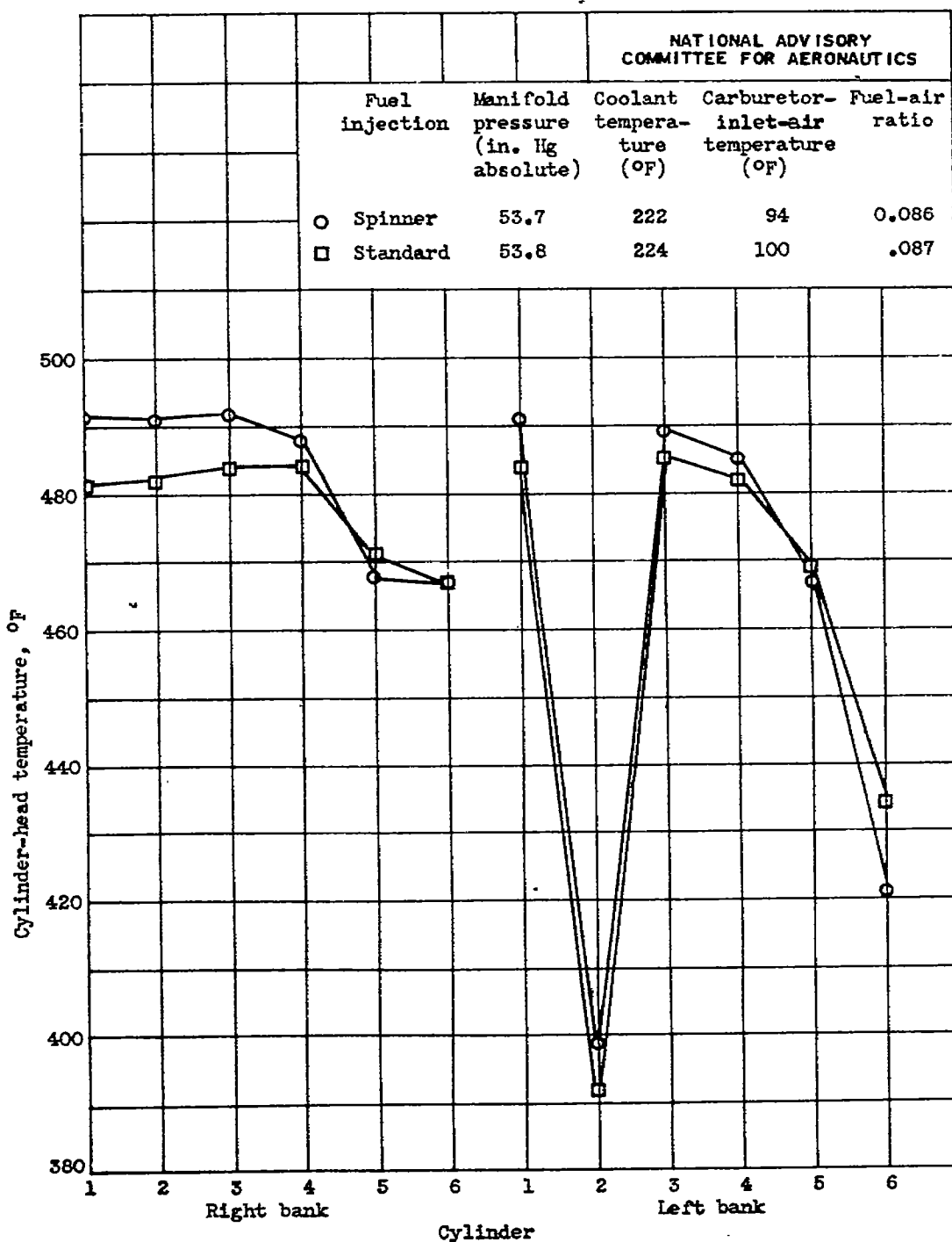
(a) Manifold pressure, 54 inches of mercury absolute.
