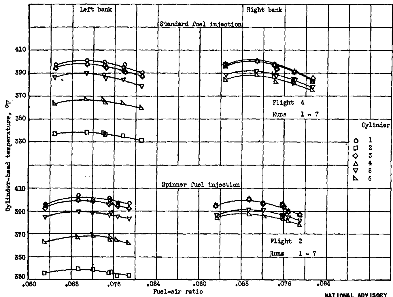
(a) Manifold pressure, 25 inches of mercury absolute.
